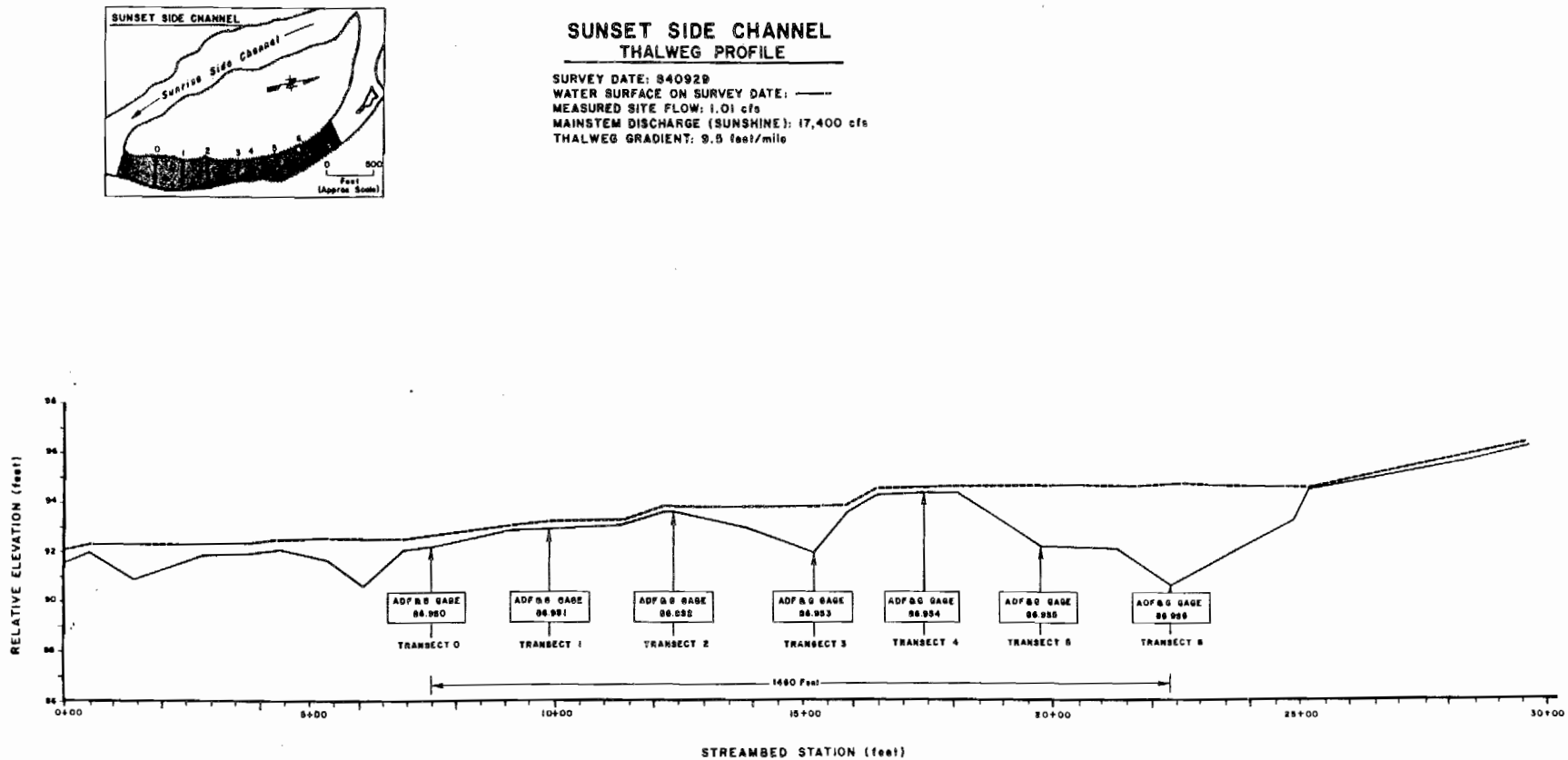
Attachment Figure C-5 Thalweg profile of Sunset Side Channel study site.
