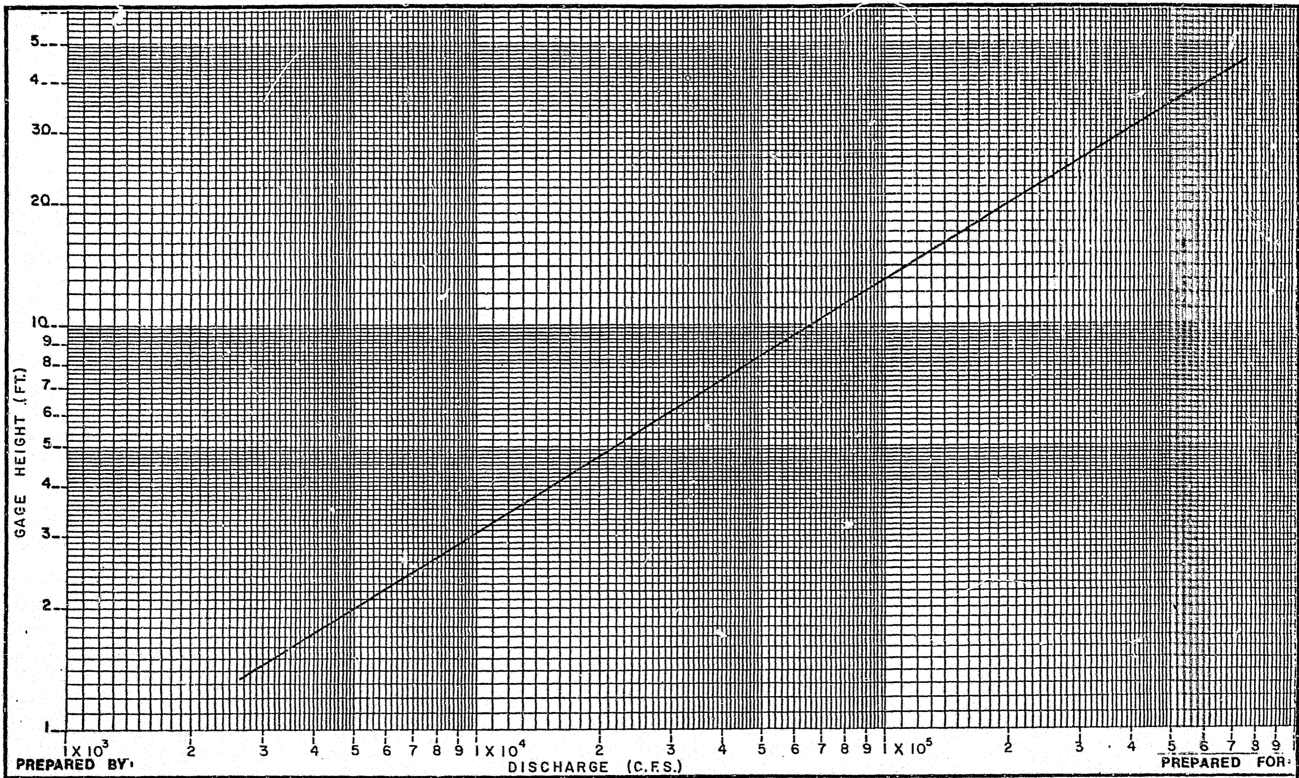
RATING CURVE FOR SUSITNA RIVER AT SUNSHINE
