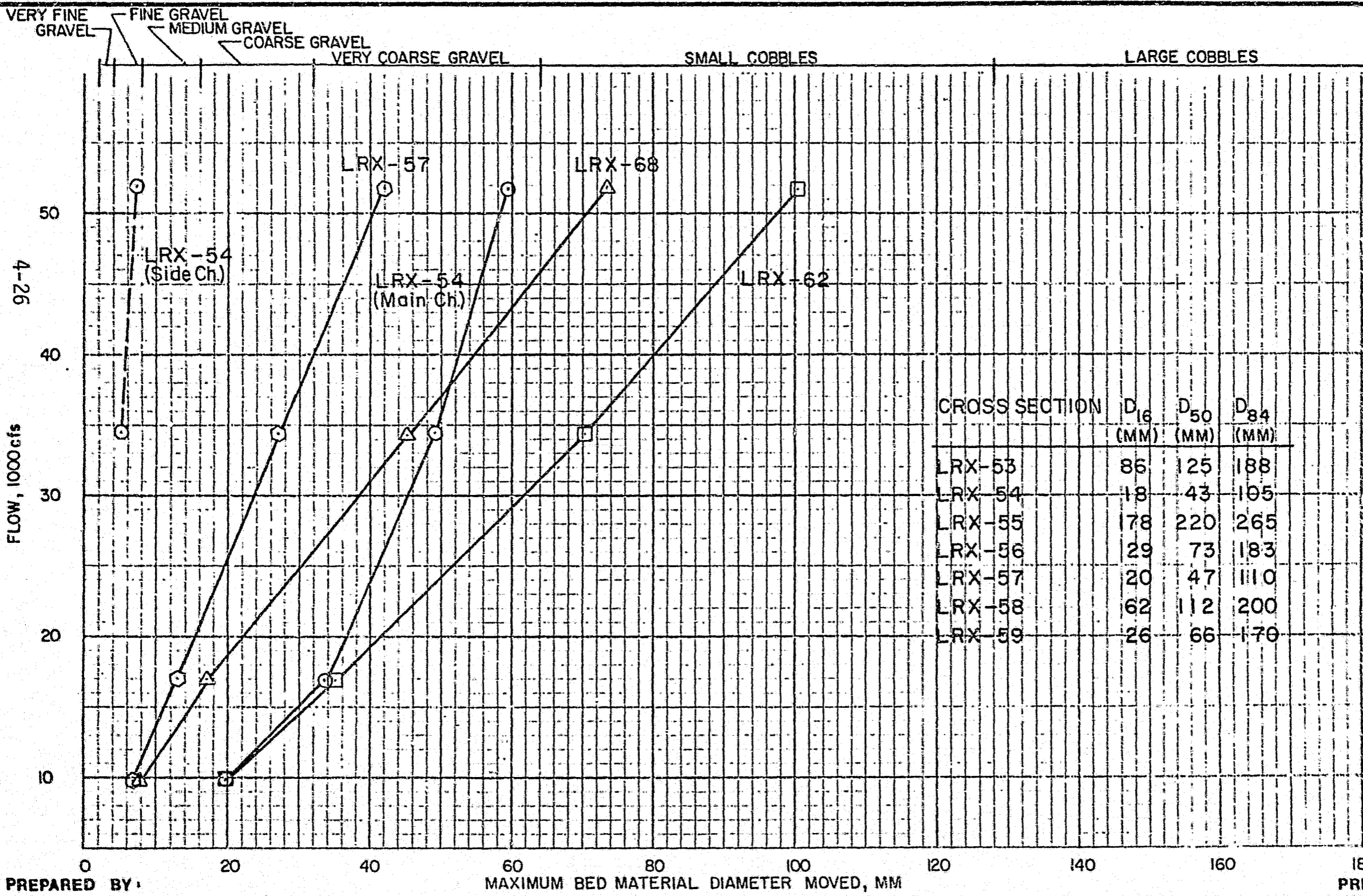
BED MATERIAL MOVEMENT CURVES LRX -54, -57, -62, -68
