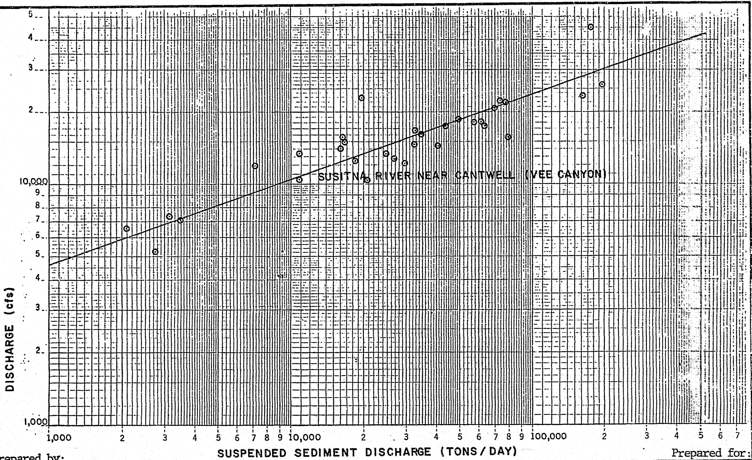
SUSPENDED SEDIMENT RATING CURVE SUSITNA RIVER NEAR CANTWELL (VEE CANYON)
