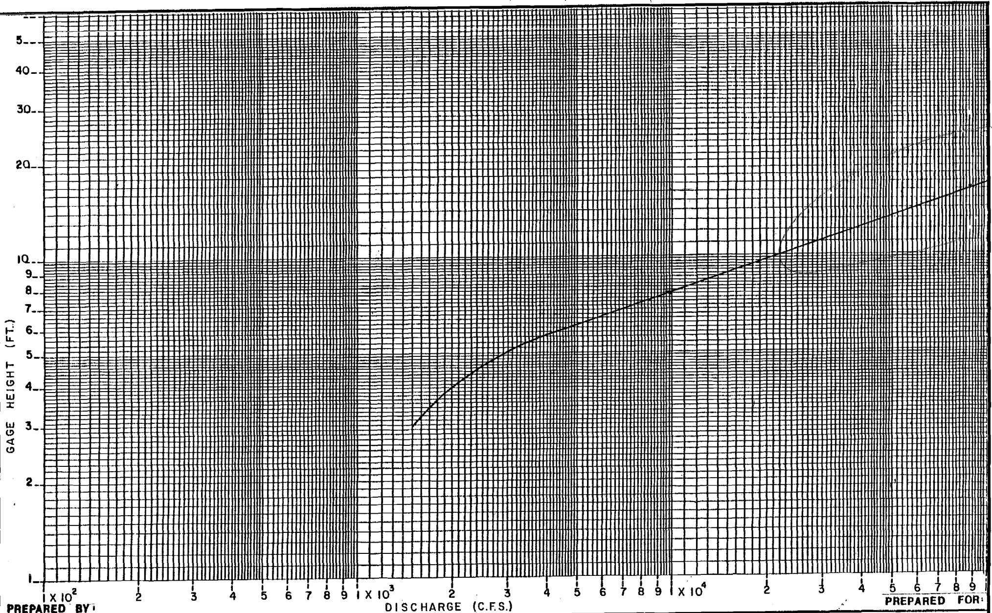
RATING CURVE FOR SUSITNA RIVER AT GOLD CREEK
