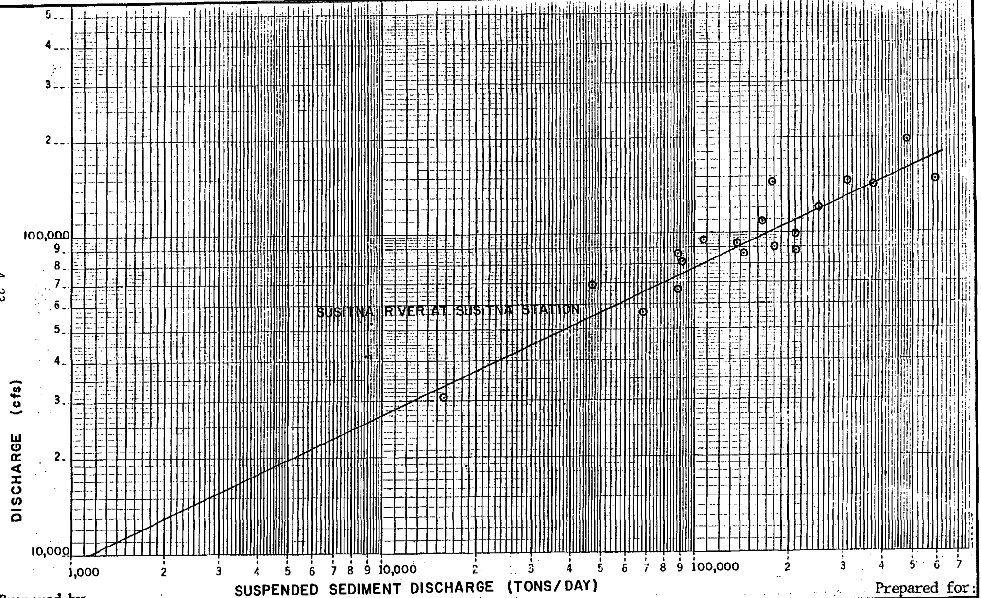
SUSPENDED SEDIMENT RATING CURVE SUSITNA RIVER AT SUSITNA STATION
