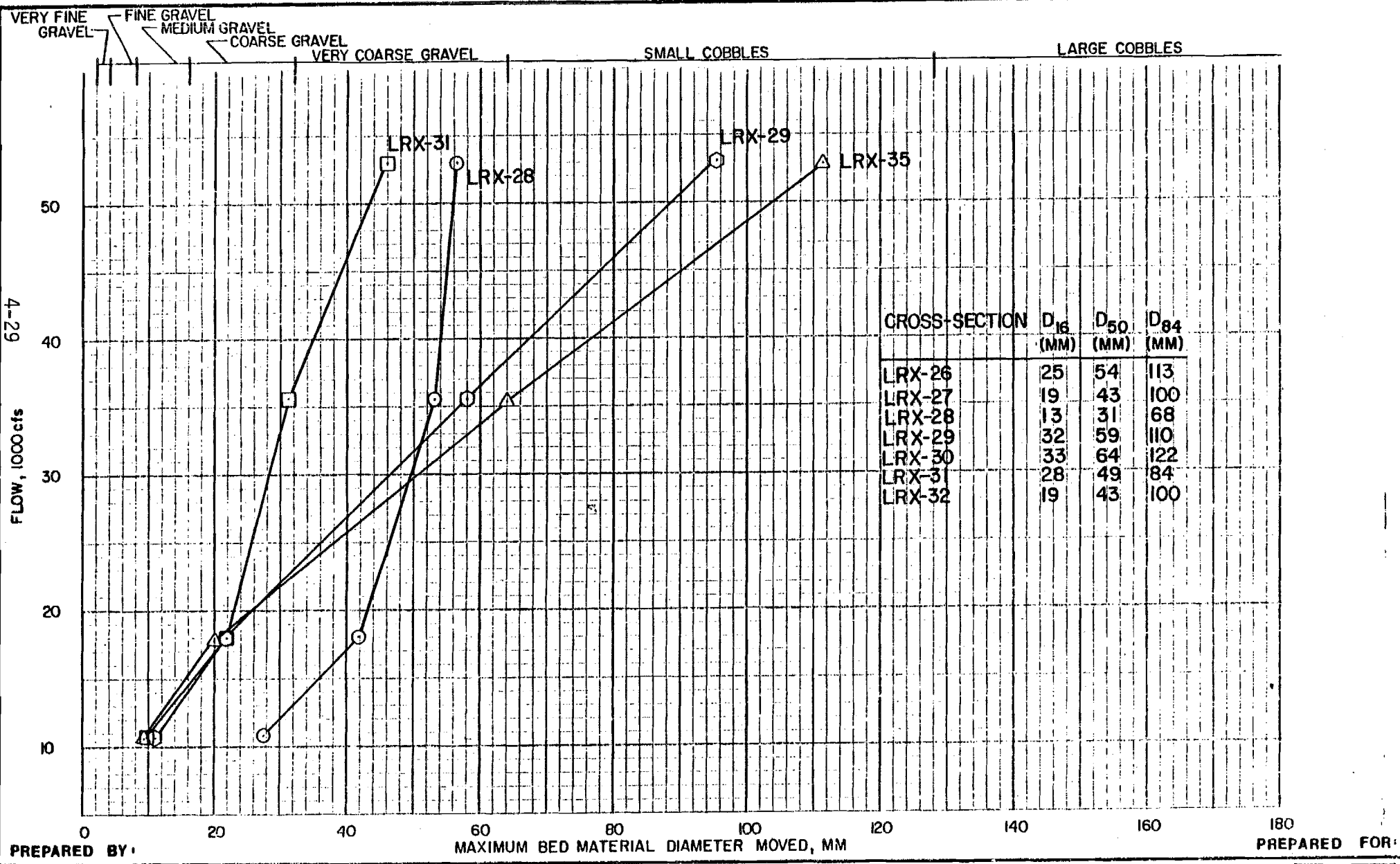
BED MATERIAL MOVEMENT CURVES LRX-28,-29,-31,-35
