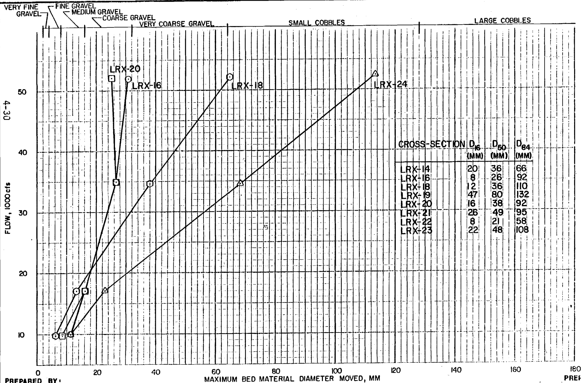
BED MATERIAL MOVEMENT CURVES LRX-16, -18, -20, -24
