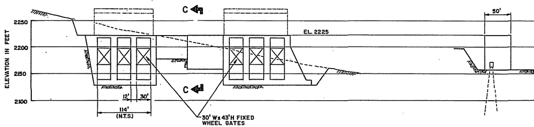
SECTION C-C
