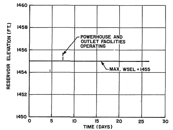
RESERVOIR ROUTING 1:50 YR. SUMMER FLOOD
