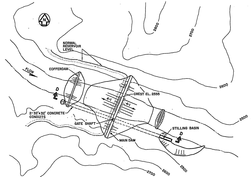
DENALI GENERAL ARRANGEMENT SCALE: A
