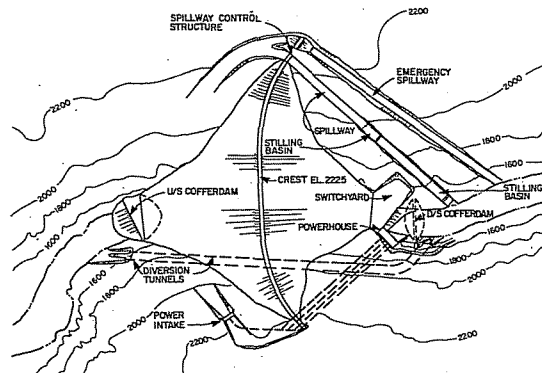
ALTERNATIVE 2C
