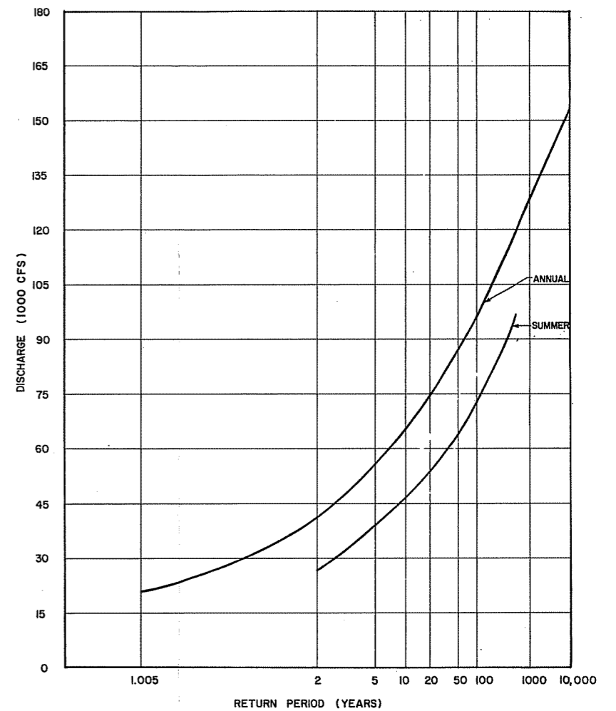
INFLOW FLOOD FREQUENCY
