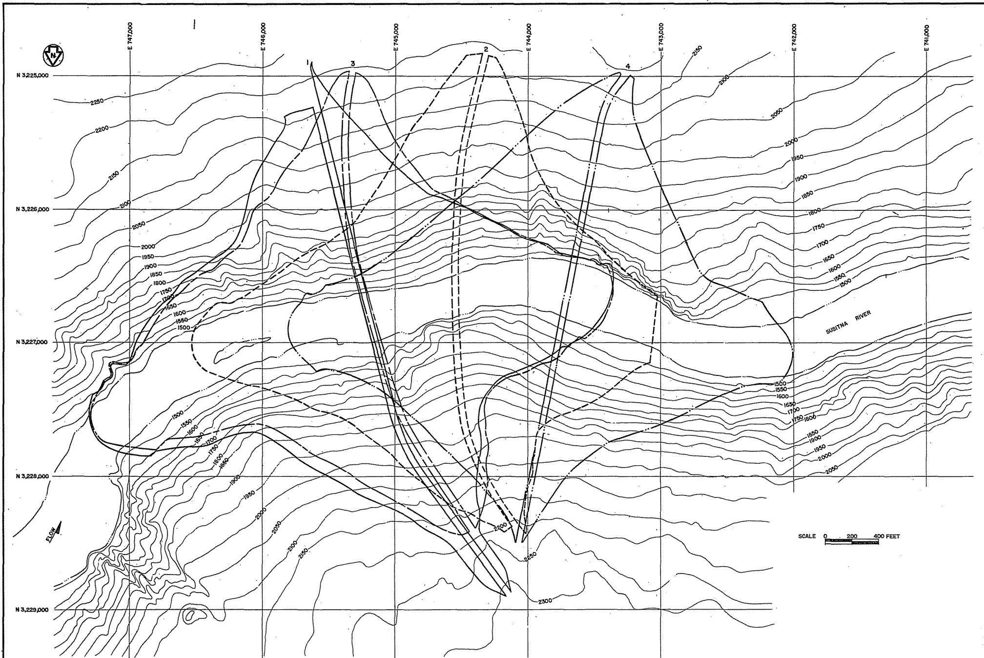
WATANA ALTERNATIVE DAM AXES
