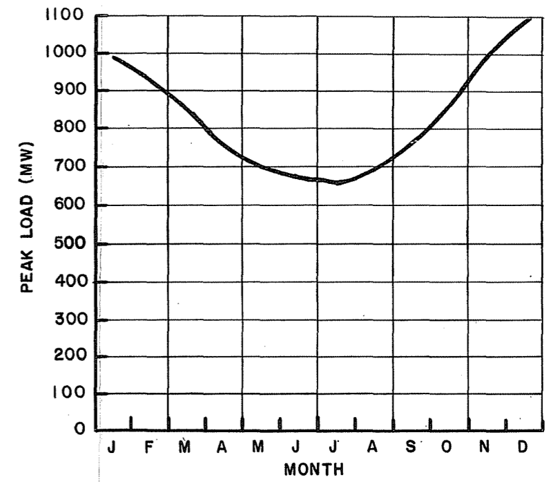
LOAD VARIATION IN YEAR 2000
