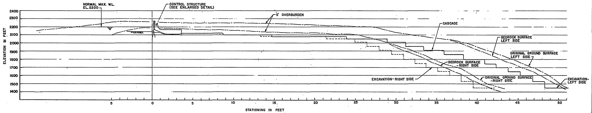
SPILLWAY PROFILE
