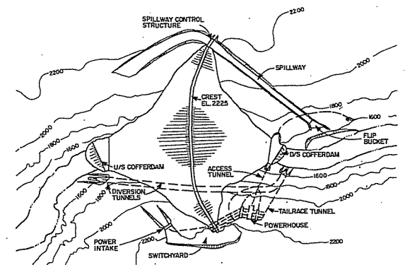
ALTERNATIVE 2D
