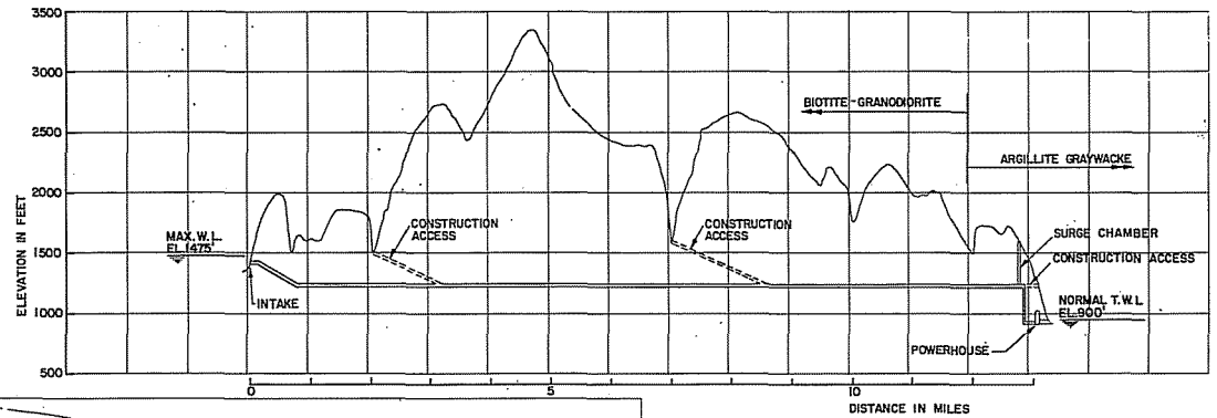
TUNNEL ALIGNMENT
