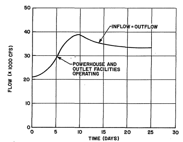
RESERVOIR ROUTING 1:50 YR. SUMMER FLOOD
