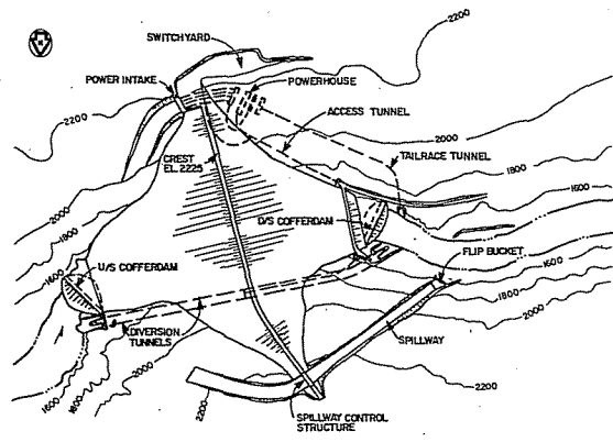
ALTERNATIVE 1
