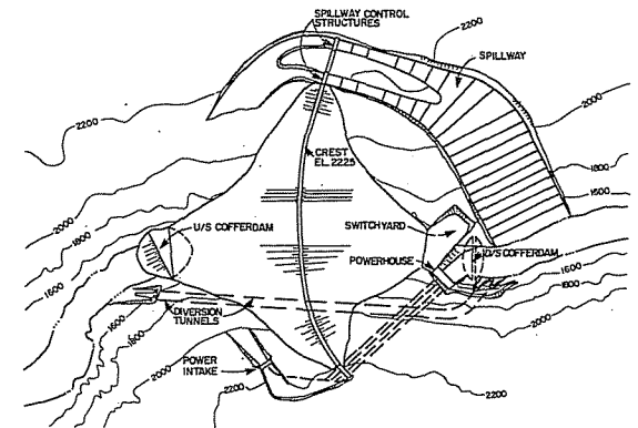
ALTERNATIVE 2A
