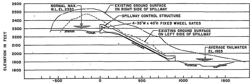
SPILLWAY PROFILE SCALE B
