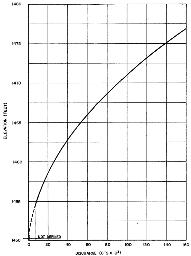
TAILWATER RATING
