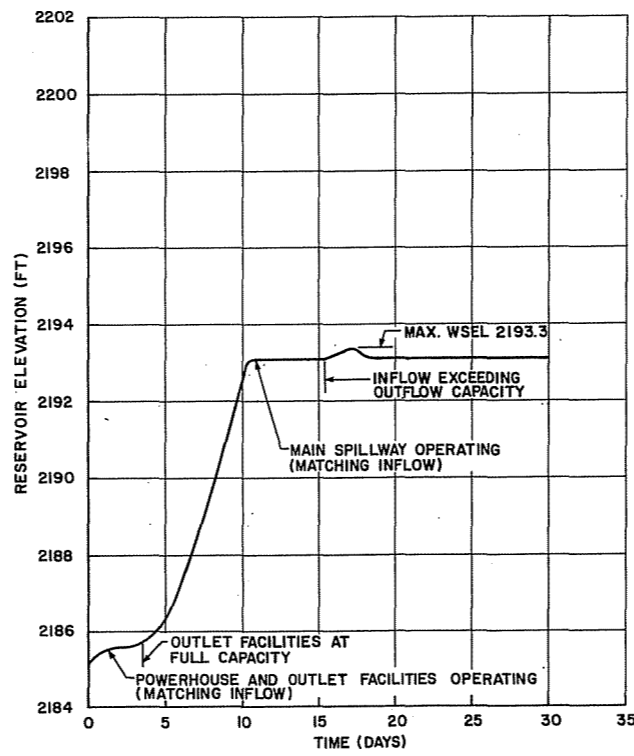
1:10,000 YEAR FLOOD
