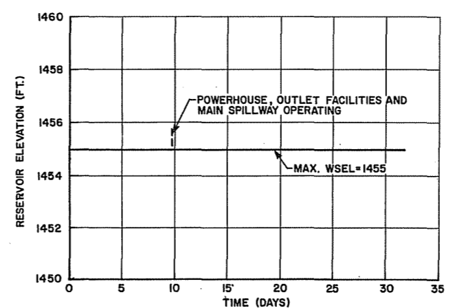
RESERVOIR ROUTING 1:10,000 YR. FLOOD
