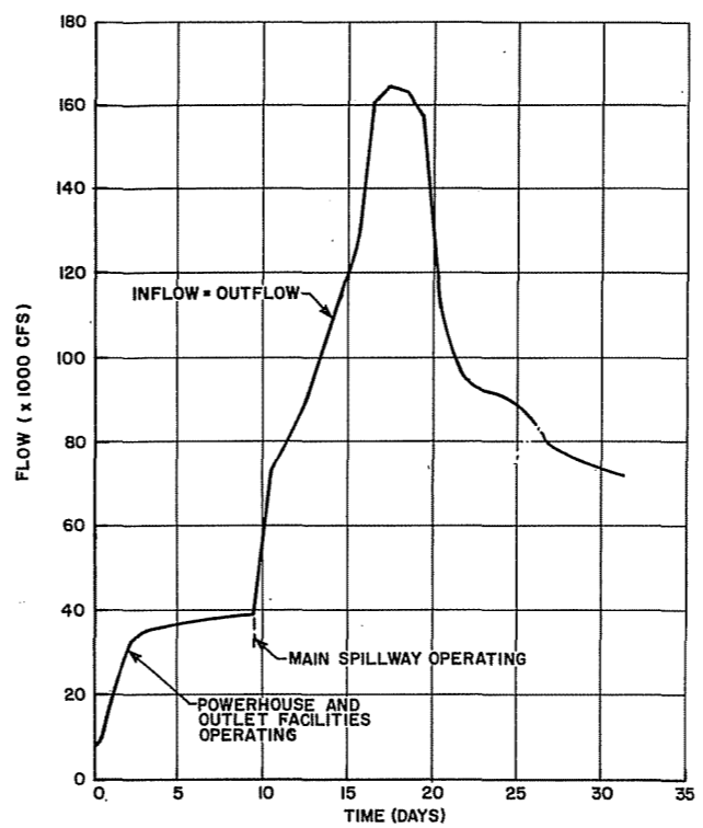
RESERVOIR ROUTING 1:10,000 YR. FLOOD
