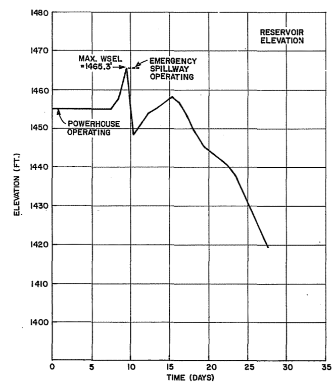
PROBABLE MAXIMUM FLOOD
