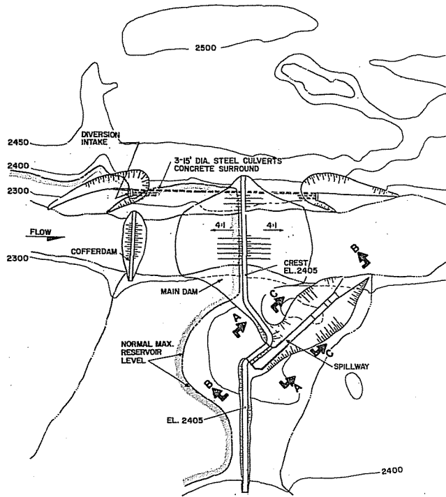
MACLAREN GENERAL ARRANGEMENT SCALE: A
