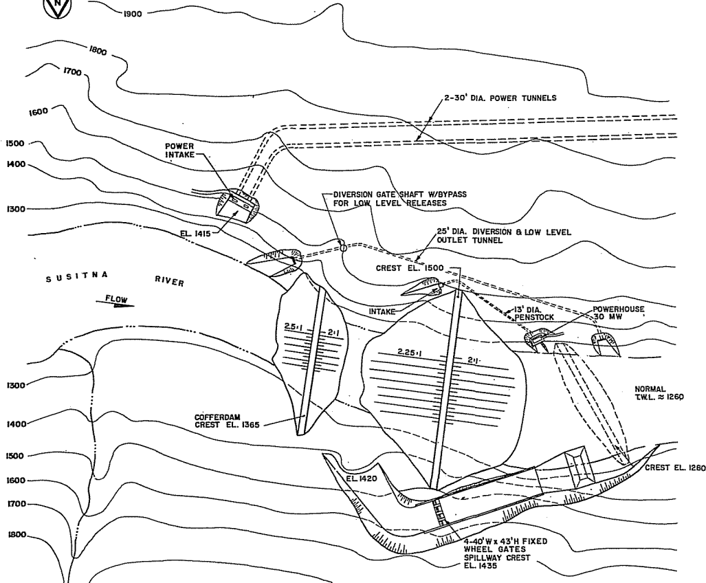
PREFERRED TUNNEL SCHEME 3 PLAN VIEW
