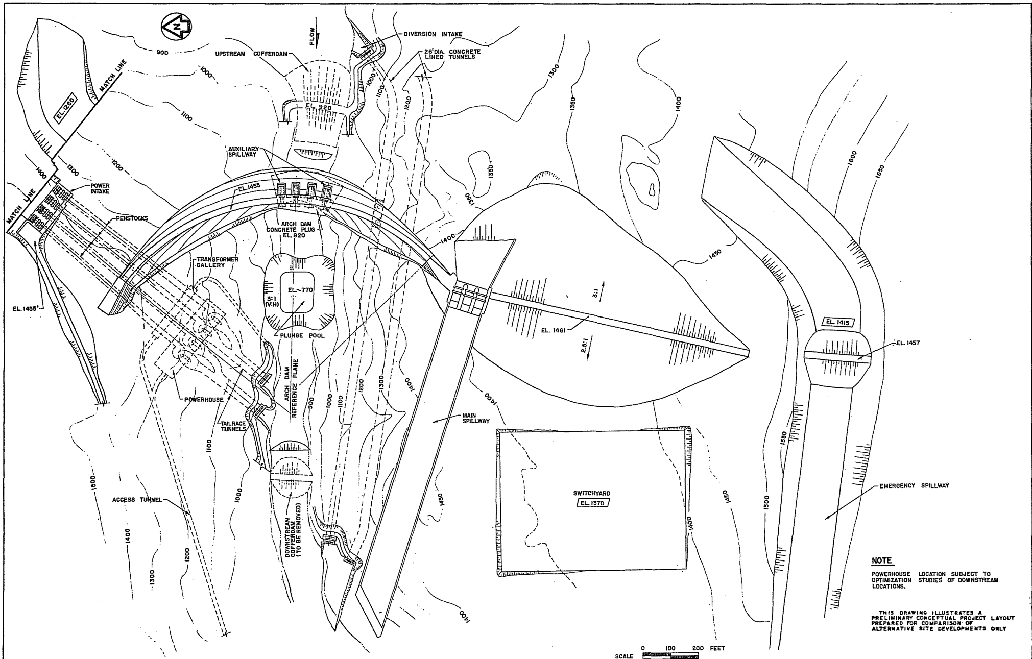
GENERAL ARRANGEMENT
