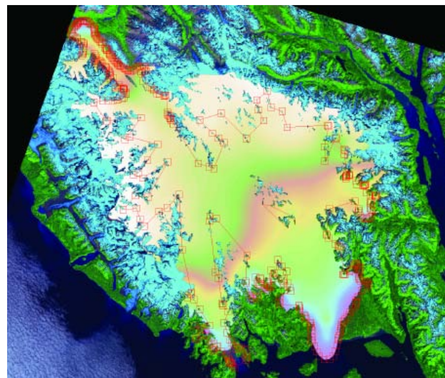
Figure 7. Reconstruction of LIA maximum glacier surface in Glacier Bay (~1750 AD) (modified from Larsen et al. 2005). The LIA maximum ice surface was determined by mapping geomorphic markers shown as squares (trimlines, lateral moraines and terminal moraines). These markers were identified through aerial inspection, vertical airphoto analysis, high resolution digital elevation model (DEM) analysis, and field observations. Modern-day glacier analogues were used to construct the Glacier Bay LIA icefield surface from the geomorphic markers. This surface was then differenced with a DEM of present-day topography to determine ice thickness change since LIA.
