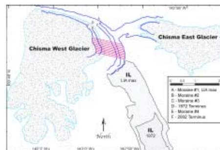
Figure 7. Terminus positions of the Chisma Glaciers. The oldest and most extensive glacier advance, shown by terminus position A (moraine #1), demonstrates that the Chisma West and Chisma East Glaciers were connected at the height of the Little Ice Age, and terminated near a strandline that marks the LIA-maximum highstand of Iceberg Lake (IL). Subsequent glacier retreat history is marked by terminus positions B-F. The mapped outlines of Chisma West and Chisma East glaciers and of the smaller shoreline of Iceberg Lake are derived from 1972 aerial photos. The larger, LIA maximum shoreline is from Loso et al. (2004). Glacier terminus positions were measured along ten transects shown by parallel dashed red lines.
