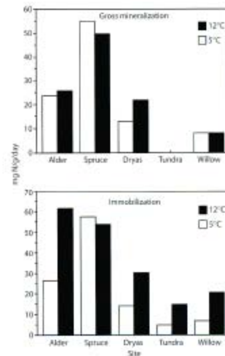
Figure 7: Results of laboratory study showing potential effects of soil warming on soil organic N mineralization rates (top plot), and soil microbial uptake of N (bottom plot) beneath major vegetation types, Asik watershed (from Binkley et al. 1994)
