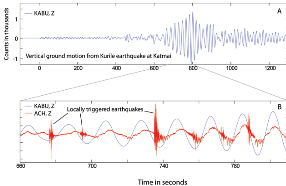
Figure 5. Dynamically triggered earthquakes at Mt. Martin Volcano following the 2007 M 8.2 Kurile earthquake: A) broadband record from seismic station KABU showing dominantly low-frequency ground motion of the Kurile earthquake in the Katmai area; B) seismic data from ACH (located near Mt. Martin) and KABU zoomed in to show how local earthquakes (spikes in red) are occurring during specific ground motion phases from the Kurile earthquake ( Prejean and Hill 2009 ).
