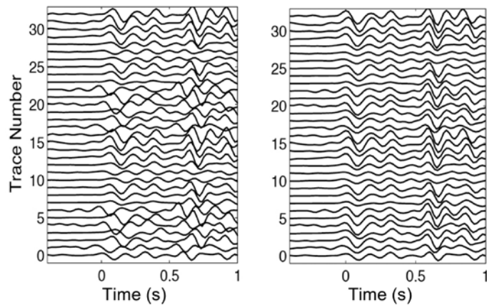
Figure 4. Comparison of seismic waveforms aligned on (left) catalog data versus (right) cross-correlation for a Katmai-area station, showing the improved alignment of the arriving waves.
