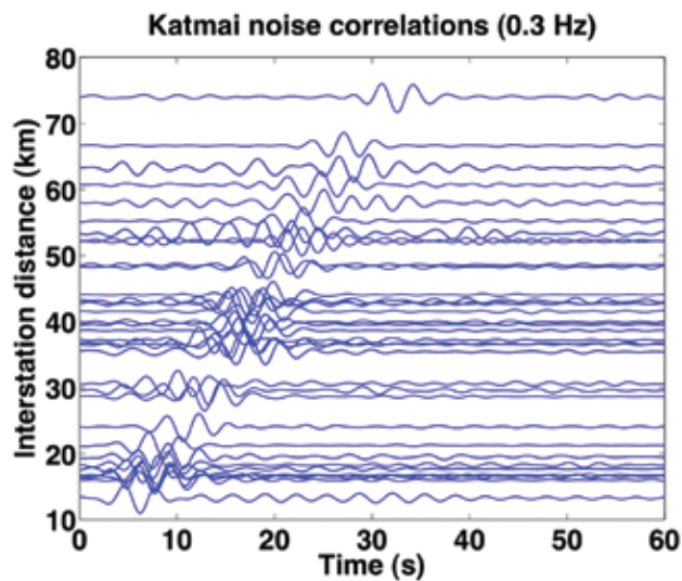
Figure 5. Ambient noise correlation results ordered by separation between the seismic stations, showing the surface waves that emerge from the method.
