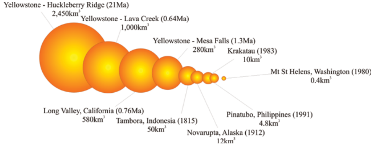
Figure 3. The relative size of the 1912 Novarupta eruption compared to several ancient and recent volcanic events.
