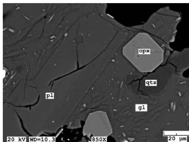
Figure 4. Scanning electron micrograph, at 850x magnification, shows groundmass in andesite lava from the final 2009 dome. Chemical compositions of the plagioclase (pl) crystals and glass (gl) allow estimates of pre-eruptive magmatic water content. Opx=orthopyroxene and qtz=quartz crystals. Scale bar is 20 micrometers (0.001 inch).
