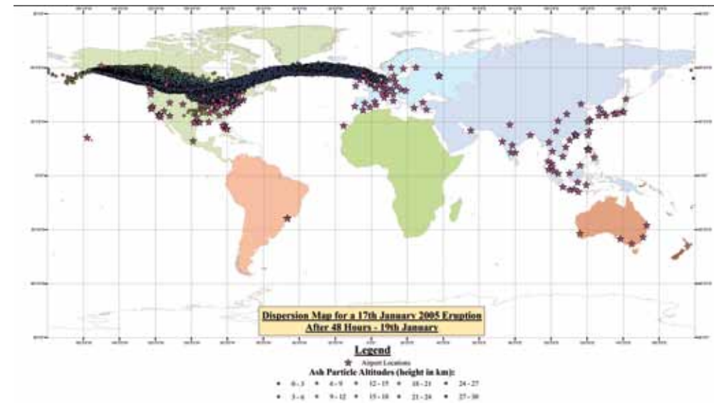
Figure 7. Dispersion of Ash Cloud from a simulated eruption on 17th January 2005 – after 48 hours.
