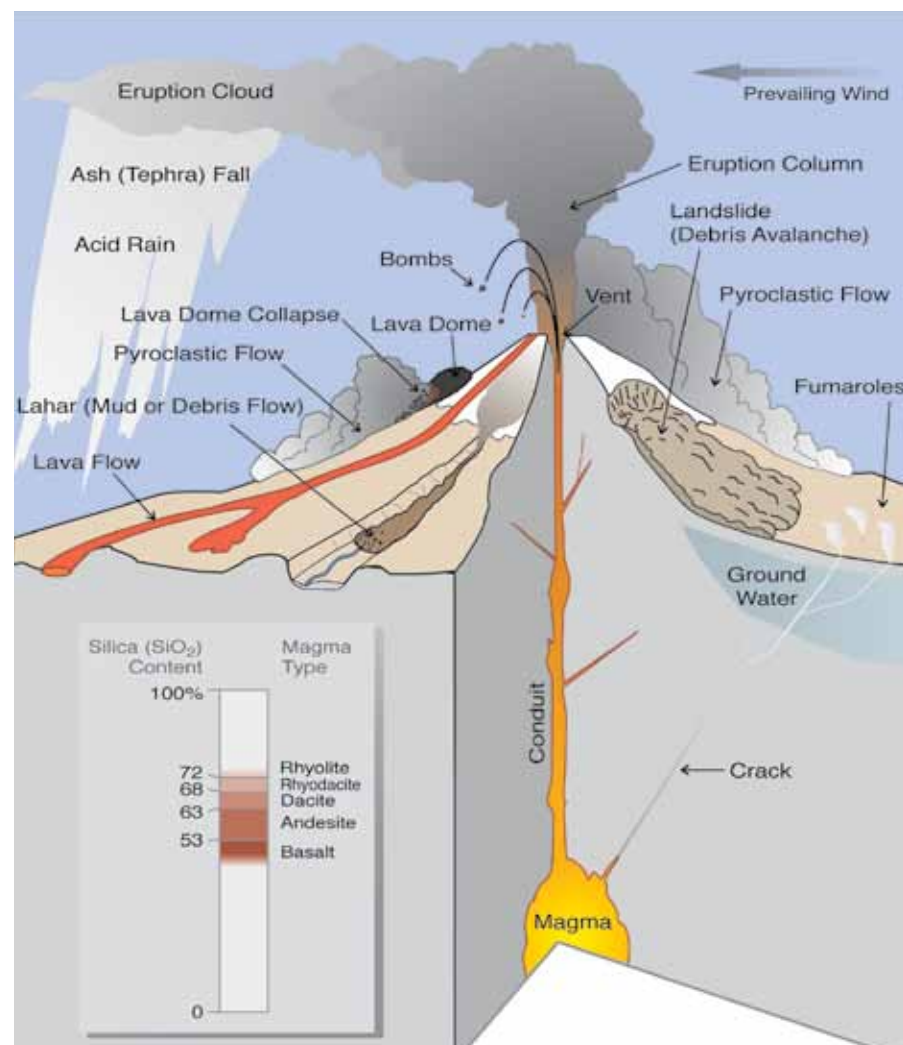
Figure 3. Hazardous phenomena associated with active volcanoes. Small eruptions typically pose hazards only within several kilometers of a volcano, whereas larger eruptions can endanger people and property at tens to hundreds of kilometers distant. Ash clouds can travel thousands of kilometers from a volcano and pose hazards to aircraft far downwind. Silicic magmas (rhyolite, rhyodacite, dacite) tend to erupt more explosively than mafic (andesite and basalt) magmas.
