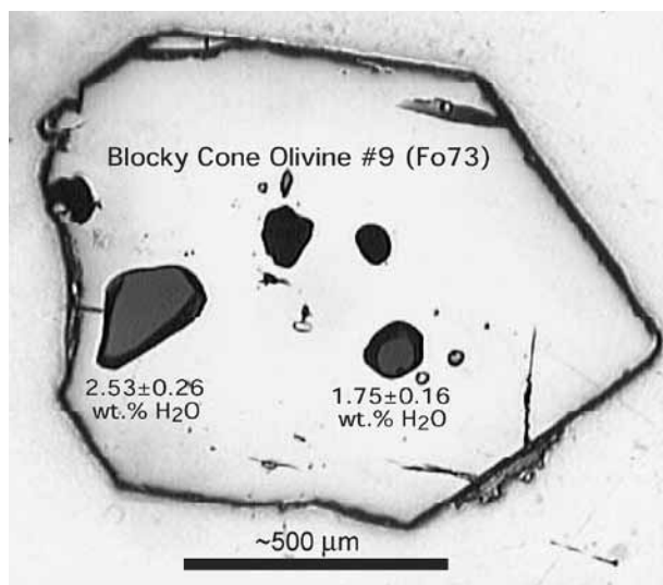
Figure 8. A polished slice of an Aniakchak olivine crystal from intracaldera Blocky Cone, showing melt inclusions. Water content, in weight percent, is shown for two of the melt inclusions as measured by FTIR. Fo73 refers to the forsterite ( \text{Mg}_2\text{SiO}_4 ) percentage in olivine.
