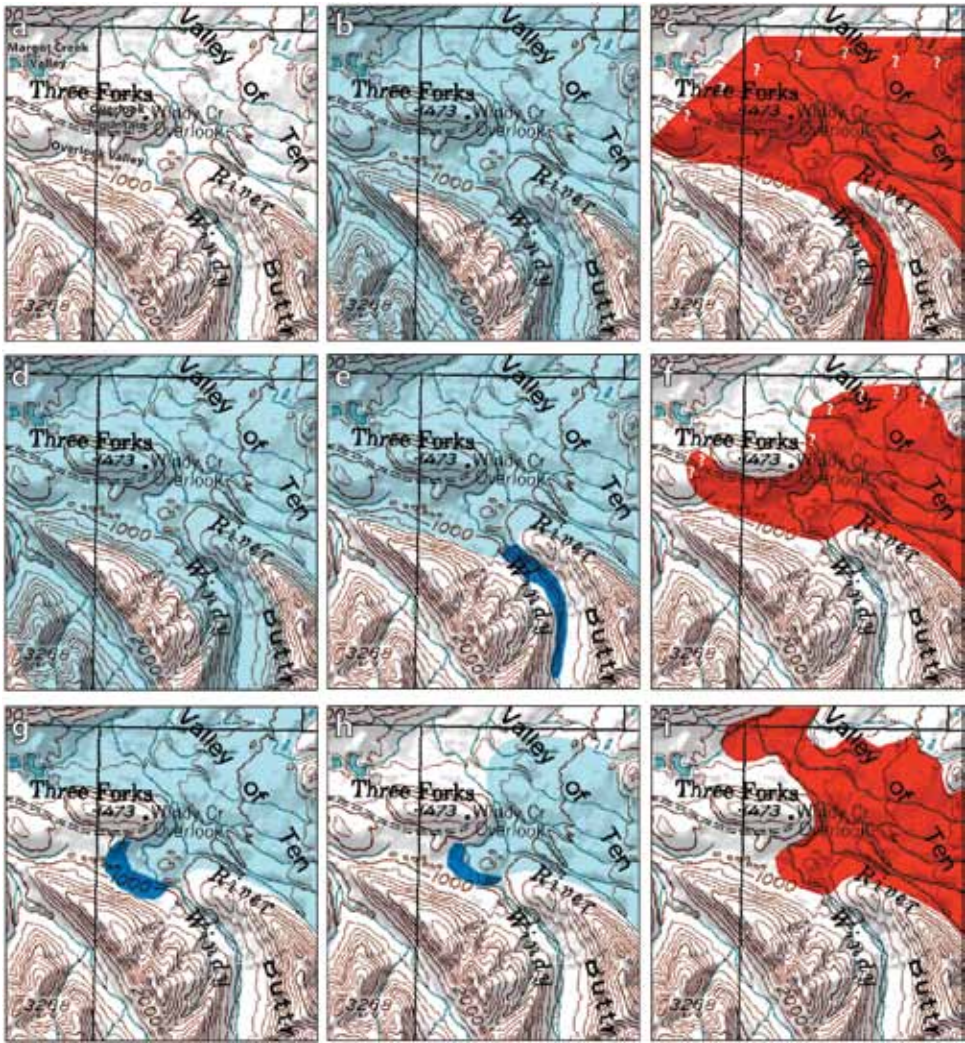
Figure 6. Late Quaternary paleogeography of the Windy Creek area. Light blue – glacial ice; dark blue – glacially dammed lakes; red – volcanic deposits. a) location map with key geographic features; b) Late Wisconsin Iliamna stadi glacial advance; c) Windy Creek ashflow eruption ca. 19,240 RC yr B.P.; d) Newhalen stadi glacial advance; e) Iliuk stadi glacial advance dams glacial lake in lower Windy Creek; f) Lethe volcanic eruption ca. 14,000-16,000 RC yr B.P.; g) Ukak glacial readvance dams small lake in Overlook valley ca. 10,000-12,000 RC yr B.P.; h) Katolinat glacial readvance dams small lake in Overlook valley ca. 8,500-10,000 RC yr B.P.; i) 1912 cataclysmic eruption forms Valley of Ten Thousand Smokes.
