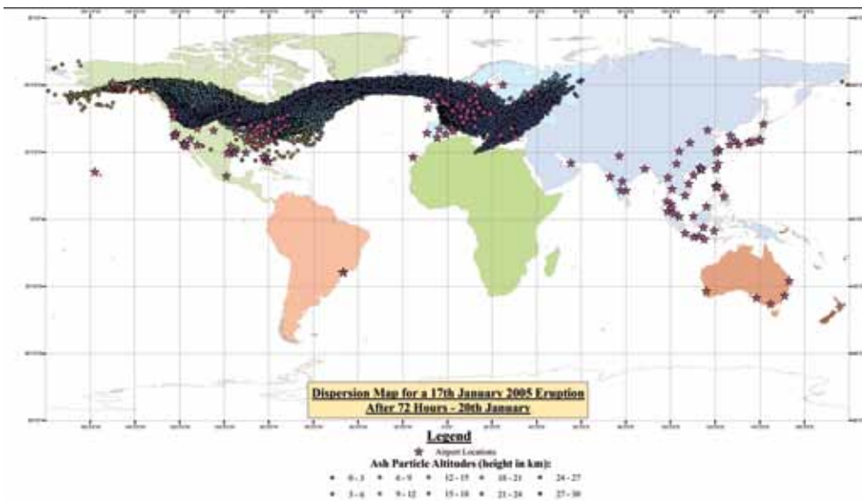
Figure 8. Dispersion of Ash Cloud from a simulated eruption on 17th January 2005 – after 72 hours.
