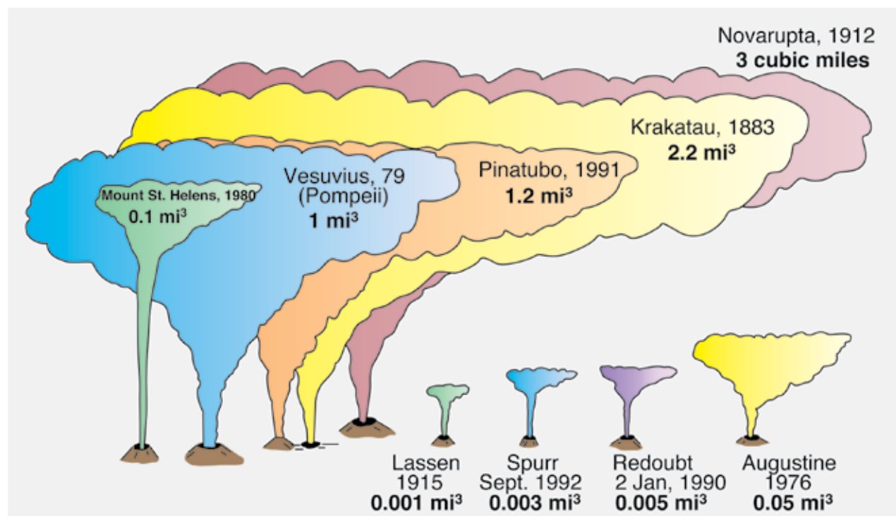
Figure 2. Comparisons of erupted magma volumes. The magnitude and volume of the eruption at Novarupta in 1912 were exceptional.
