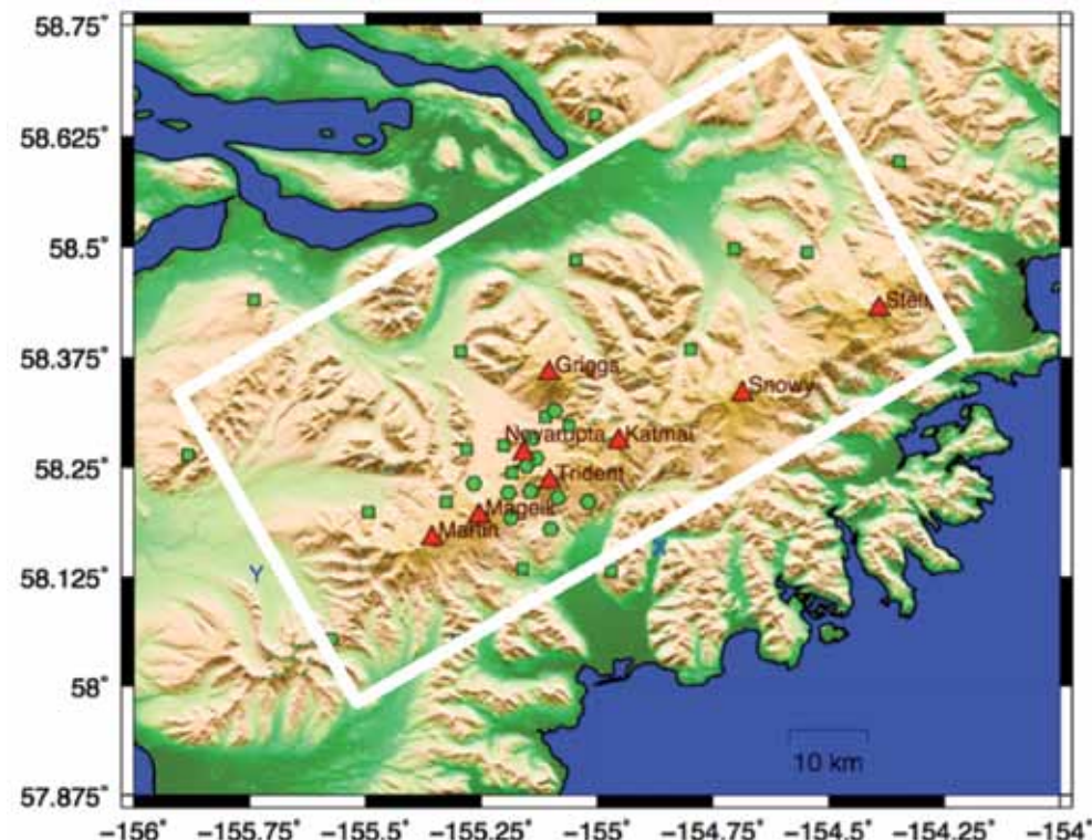
Figure 3. Map of seismic stations in the Katmai area. Green squares represent AVO permanent stations; green circles are AVO/UWM temporary stations. Red triangles are volcanoes with names indicated. The white rectangle is the outer edge of the body-wave seismic velocity model.
