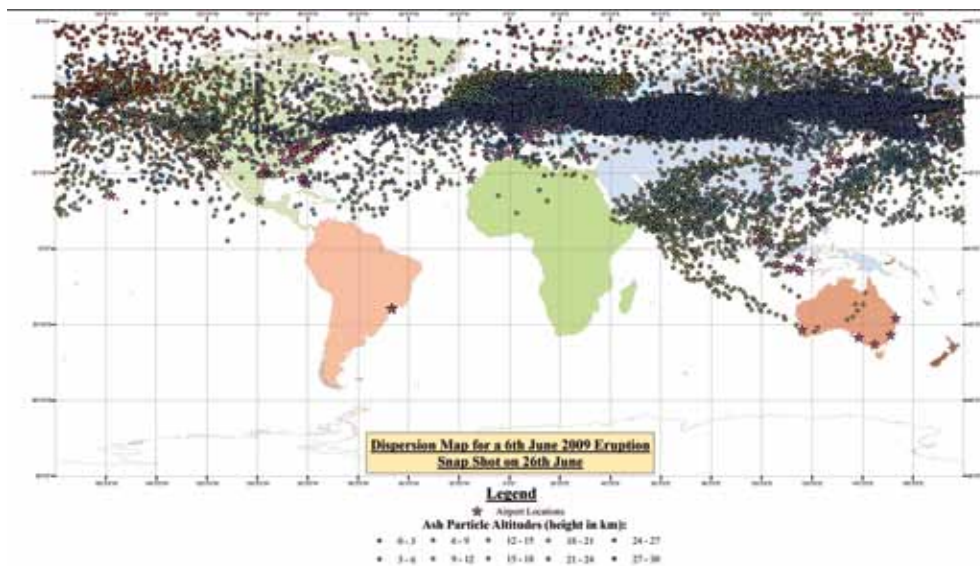
Figure 12. Ash from a simulated eruption starting 6th June 2009 after 20 days.
