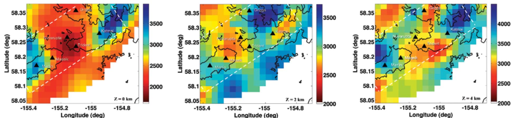
Figure 7. S-wave velocity image from ambient noise tomography in horizontal slices at 0, 2, and 4 km depth (relative to sea level), with the partial dashed white box indicating the area of the P-wave model in Figure 5. The structure deeper than 4 km is not adequately resolved by the ambient noise data, so is not shown. Velocities are in meters per second. This model is represented mathematically as cubes 2 km in size of constant seismic velocity.
