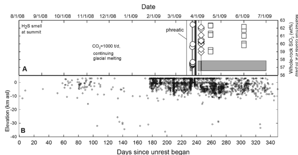
Figure 3. Silicon dioxide content of erupted andesite (A) and depths of located earthquakes (B) charted during the 2009 eruption of Redoubt. In (A), vertical lines are explosions, grey bars indicate periods of lava effusion, circles represent tephra from explosions, diamonds are samples from April 4 explosion, and squares are lavas from the final dome. Timing of hydrogen sulfide (H 2 S) smell and rates of carbon dioxide (CO 2 ) are noted. Initial explosion on March 15 was gas-rich (phreatic); no new magma was ejected. Note that eruptive products become more SiO 2 -rich with time.
