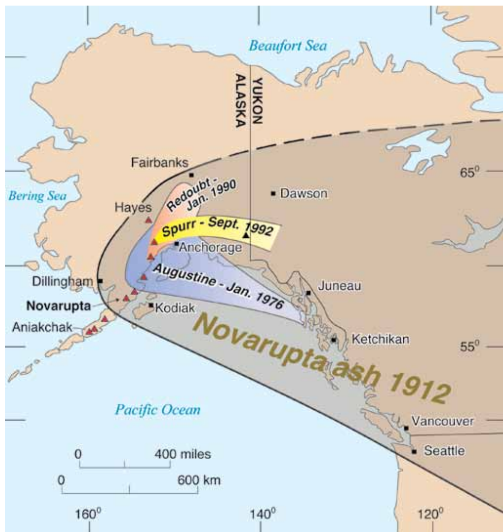
Figure 2. Alaska Peninsula map of volcanoes with Novarupta ash fall compared to that from recent eruptions. The volume of volcanic ash from Novarupta was more than from all other historical Alaska eruptions combined. Ash from seven prehistoric eruptions, all younger than 6,000 years and approaching the volume of the 1912 event, are found within 500 miles (800 km) of Anchorage, including ash from Hayes volcano.
