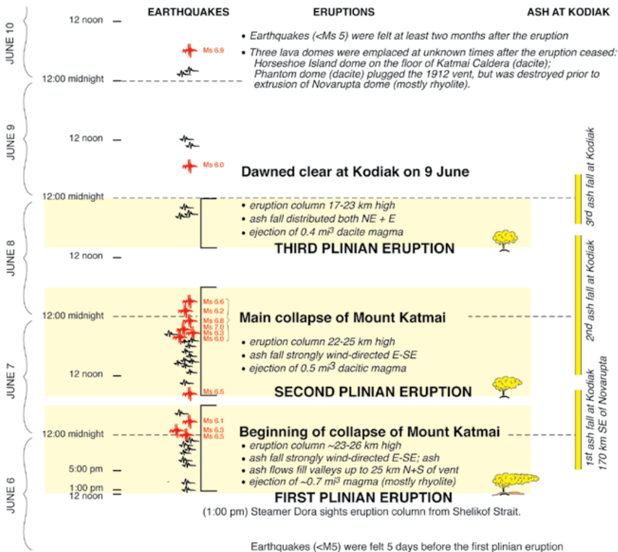
Figure 5. Chronology of 1912 eruption of Novarupta. Earthquakes felt by local residents during preceding 5 days prompted evacuation to what they hoped were safer havens. Ms=earthquake surface-wave magnitude as measured on Richter scale. Although only one seismograph was operating in Alaska at the time of the eruption, many of the earthquakes were big enough to be recorded by instruments in Europe, Asia, Japan, Hawaii, North Africa and North America (Abe 1992).
