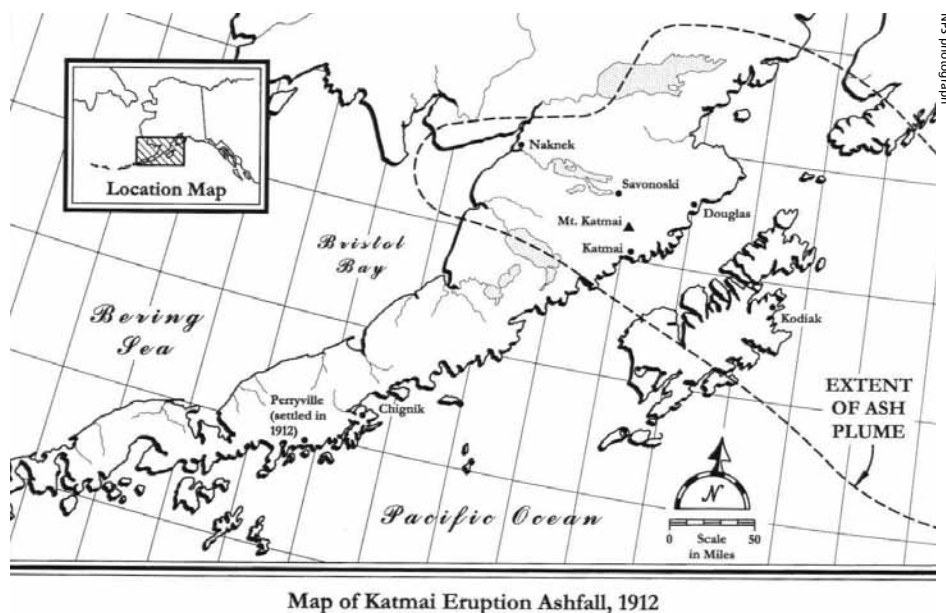
Figure 2. Map of the Alaska Peninsula with the effects of the 1912 eruption.
