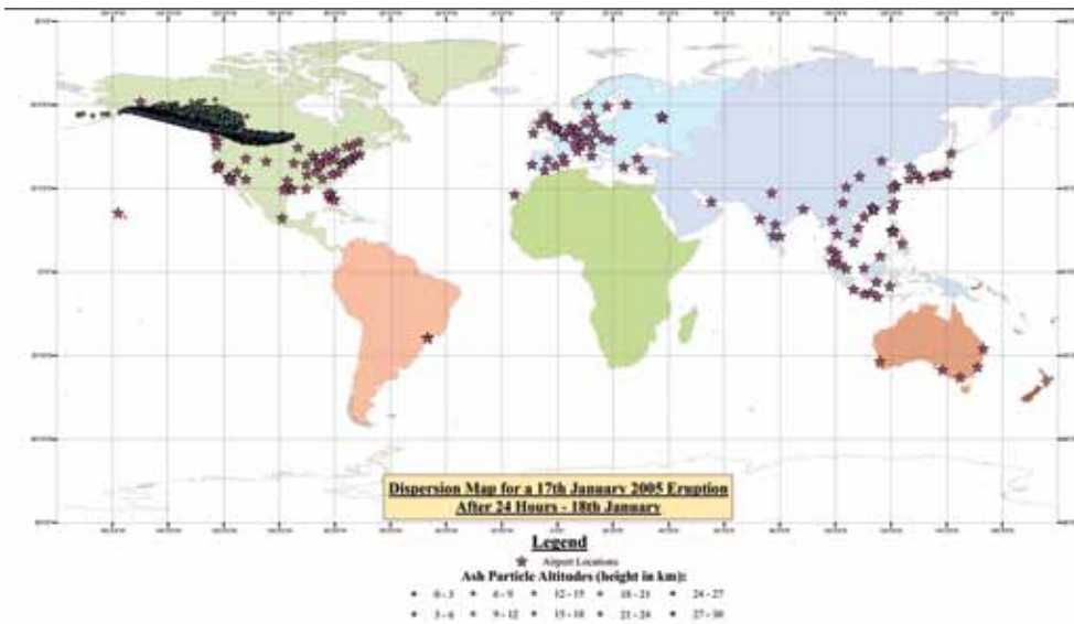
Figure 6. Dispersion of ash cloud from a simulated eruption on 17th January 2005 – after 24 hours.
