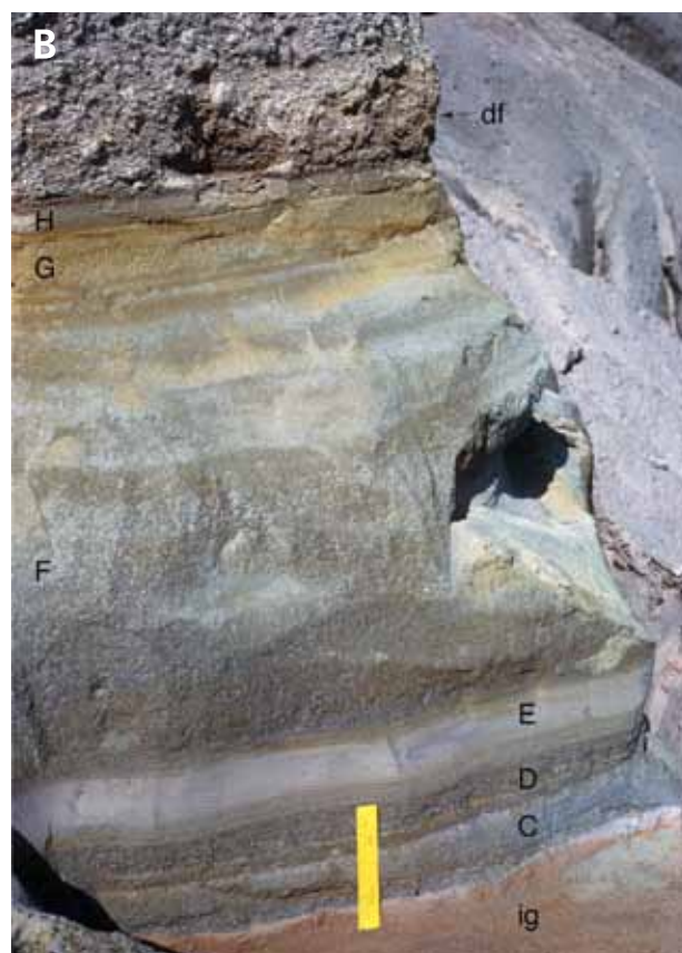
Figure 9. Fall deposits at different distances from vent. Deposits are coarsest and thickest closest to vent, and get thinner and finer with distance. (A) Coarse dacite pumice fall deposits of Episodes II and III are about 36 feet (12 m) thick, 2.5 miles (4 km) northeast of Novarupta. Fall layers are labeled C-G. (B) Complete section of dacite fall deposits of Episodes II and III are 3 feet (1 m) thick, about 7 miles (11 km) upwind northwest of Novarupta. Fall layers are labeled C-H. Debris flow (df) on top is a flood deposit that covered the 1912 fall soon after the eruption. (C) Structureless white fine ash, about 8 inches (20 cm) thick, at Brooks Camp, which is about 30 miles (50 km) upwind northwest of Novarupta. This layer includes ash contributions from all three eruptive episodes. (D) Large block about 0.6 miles (1 km) from Novarupta dome that never went into the high eruption column. Instead, it was ejected ballistically at lower angles. The block is made up of rhyolite, dacite, and andesite pumice clasts welded together by heat inside the vent, then subsequently ejected.
