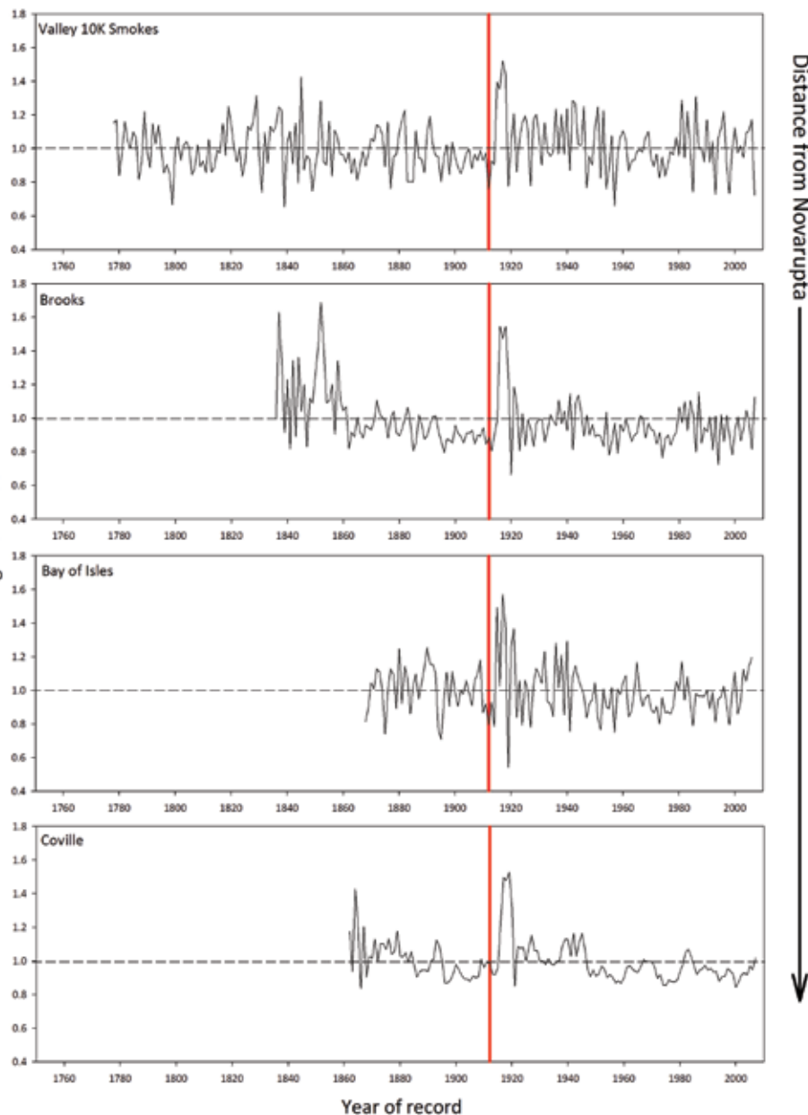
Figure 2. Tree-ring chronologies from forested sites in Katmai, sorted by increasing distance from the 1912 eruption site. Ring-width index shows growth trends averaged across all trees at a site, with values <1.0 indicating slower than average annual growth, and values >1.0 indicating greater than average growth. The 1912 eruption is indicated by the red line.
