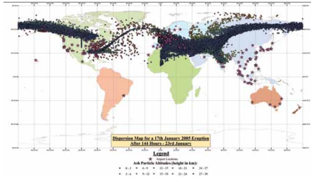
Figure 11. Dispersion of Ash Cloud from a simulated eruption on 17th January 2005 – after 144 hours.
