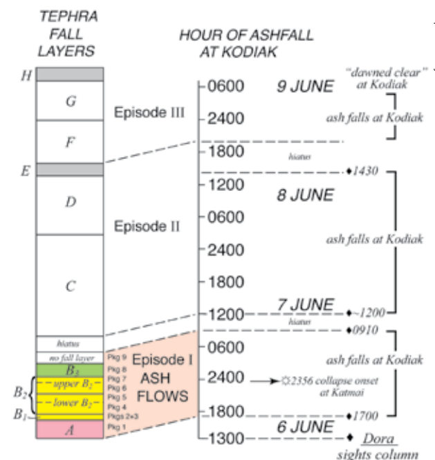
Figure 6. Generalized 1912 eruptive sequence and chronology of ashfall recorded at Kodiak village, about 100 miles (170 km) downwind. Four-hour offset at base represents time between initial sighting of eruption column by S.S. Dora and the beginning of ash fall at Kodiak.
