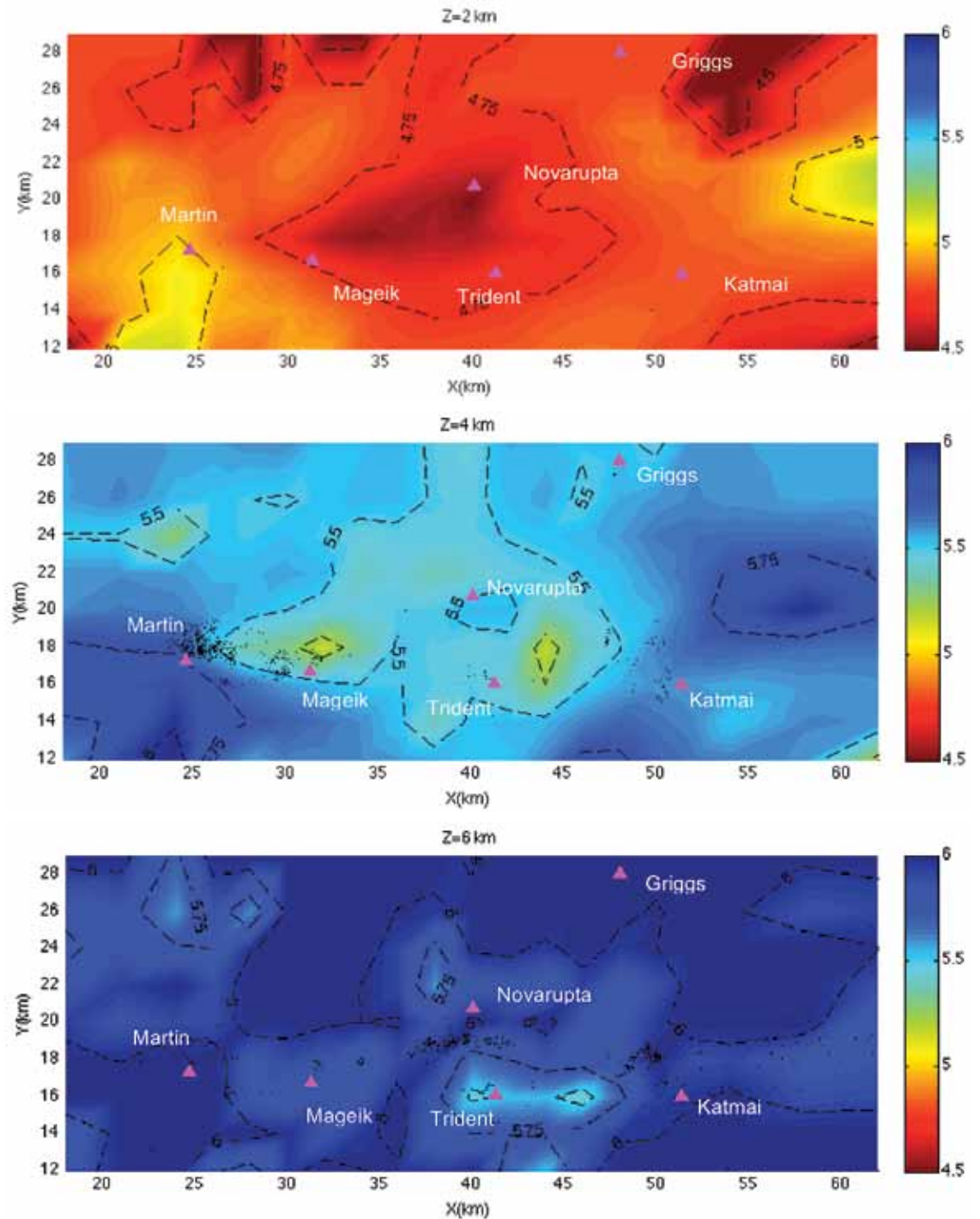
Figure 6. (Right) P-wave velocity image from body-wave tomography in horizontal slices at 2, 4, and 6 km depth (relative to sea level) for the boxed area in Figure 2. The structure shallower than 2 km is not adequately resolved by the body-wave data, so is not shown. Velocities are in kilometers per second. This model is represented mathematically as smoothly varying between points spaced 2 km apart where the seismic velocity value is defined.
