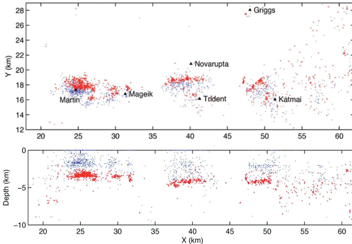
Figure 8. Comparison of catalog (blue) to relocated (red) earthquakes, (a. Top) map view and (b. Bottom) northeast-southwest cross-section. Note the greater degree of clustering in both views and the greater depths evident in (b) for the relocated earthquakes.
