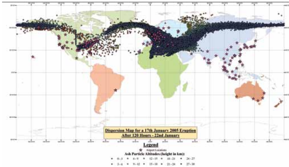
Figure 10. Dispersion of Ash Cloud from a simulated eruption on 17th January 2005 – after 120 hours.
