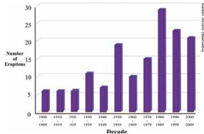
Figure 2. Number of eruptions per decade of Alaska volcanoes.
