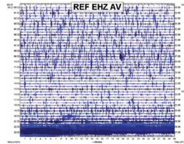
Figure 3. ‘Webicorder’ plot showing 24 hours of seismic data from station REF on Redoubt Volcano, March 21 and 22, 2009. Time goes forward from top to bottom and left to right; each horizontal line represents 30 minutes. Spikes in first 21 hours are individual earthquakes often occurring at a rate of two to three per minute. Large amplitude seismic waves at bottom of figure result from eruption onset.
