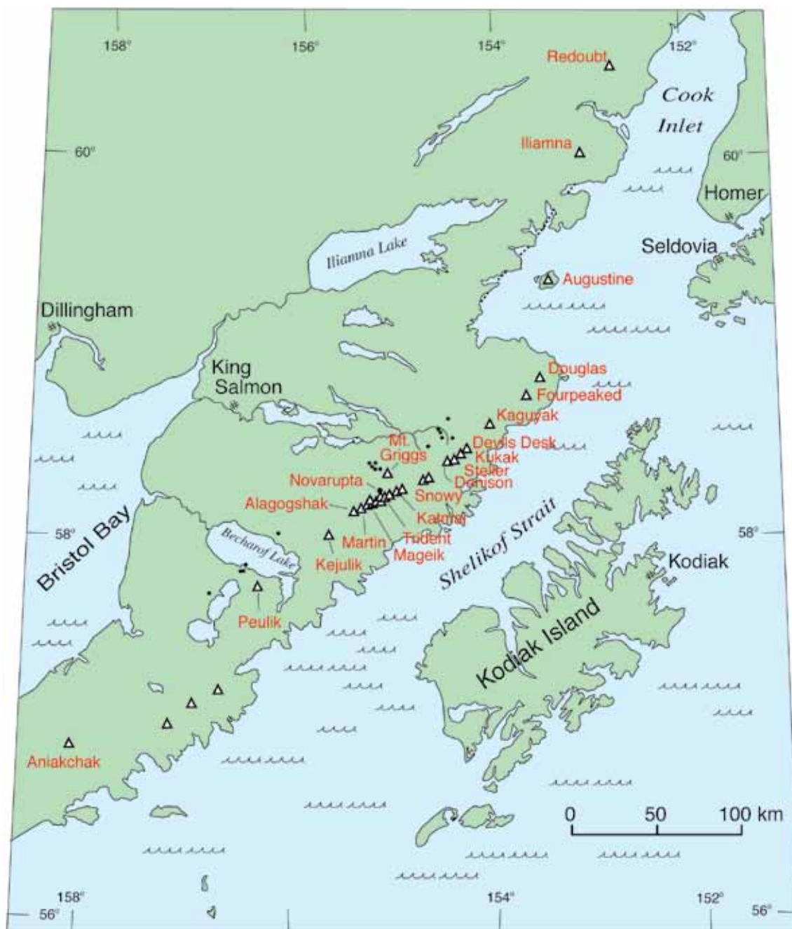
Figure 2. Map of upper Alaska Peninsula and Kodiak Island group, showing names of volcanoes (triangles) along part of Aleutian arc.
