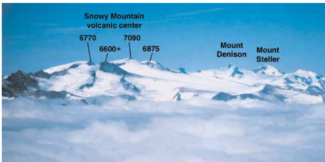
Figure 9. Aerial view northeastward over clouds to multiple summits of Snowy Mountain volcanic center. Highest summit (7,090 ft; 2,161 m) is a remnant of the west flank of Northeast Snowy, and the 6,875-foot (2,096-m) peak is a young lava dome, filling the summit crater of that edifice.
