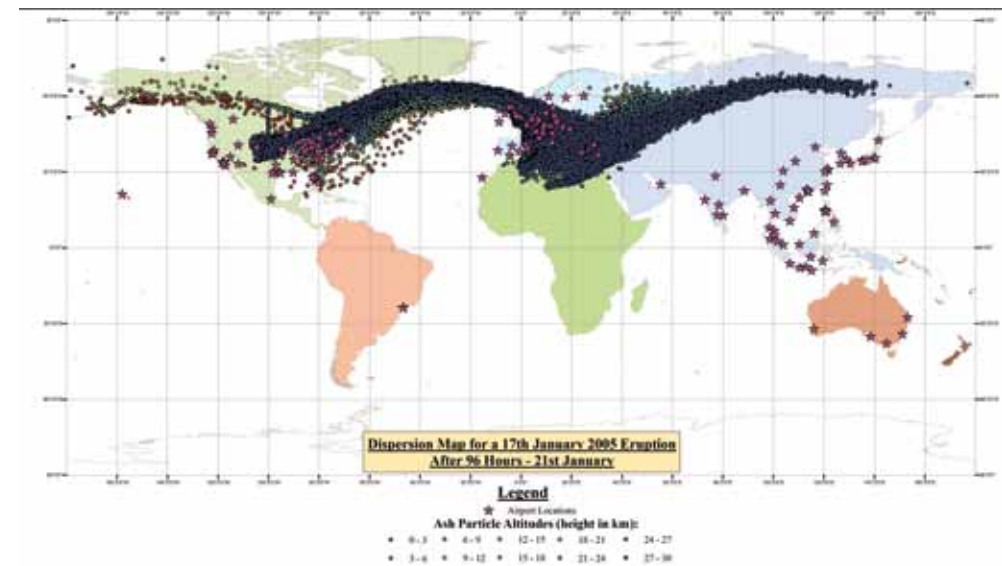
Figure 9. Dispersion of Ash Cloud from a simulated eruption on 17th January 2005 – after 96 hours.
