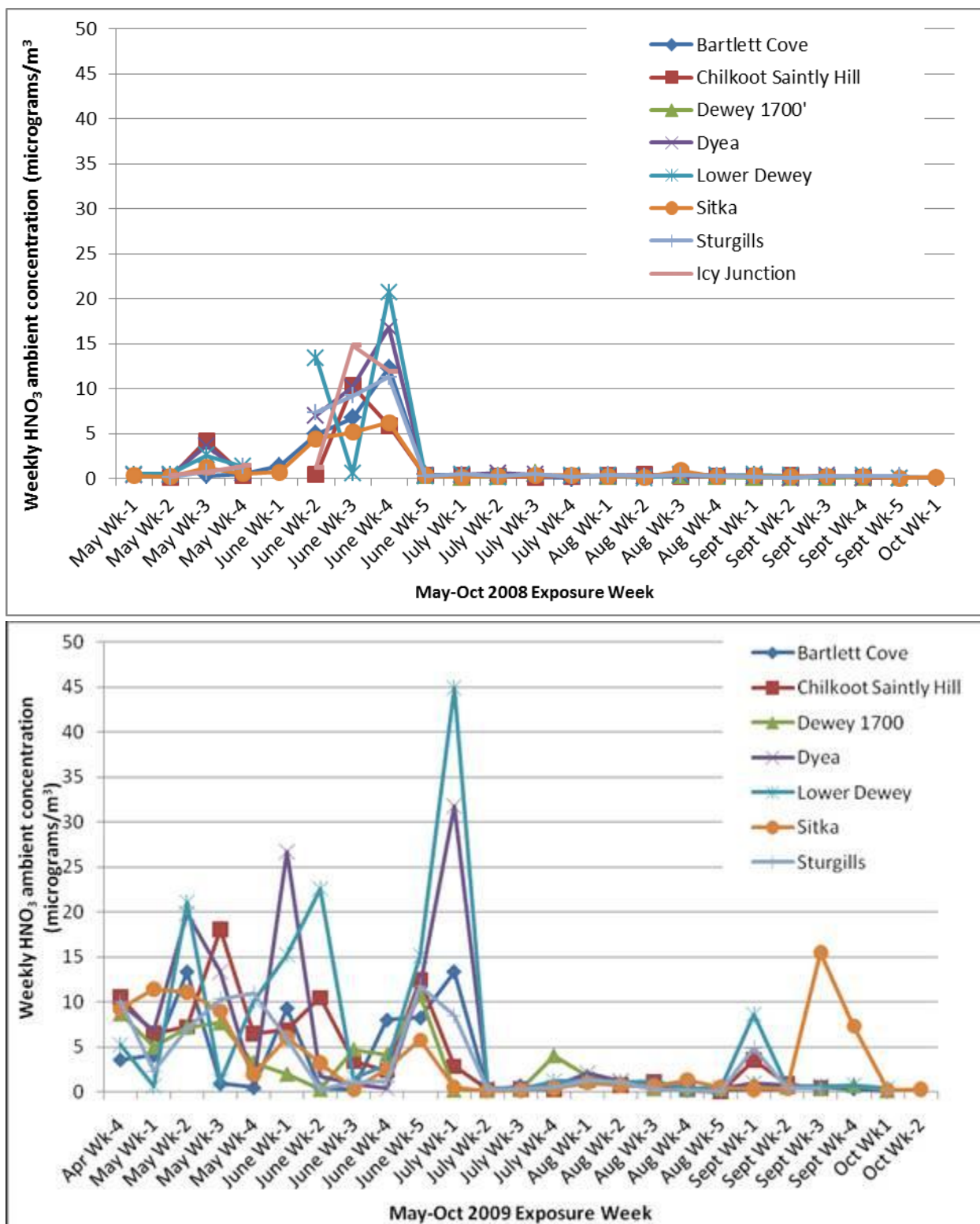
Figure 13. Weekly \text{HNO}_3 ambient concentrations during May-Oct sampler exposure weeks in (a) 2008 and (b) 2009 for Glacier Bay NPP, Sitka NHP, and Klondike Gold Rush NHP study sites.
