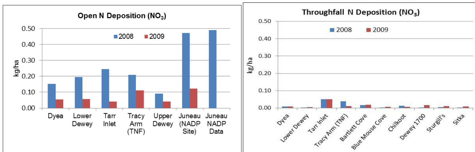
Figure 16. Open and canopy throughfall deposition of \text{NO}_3^- in 2008 and 2009.
