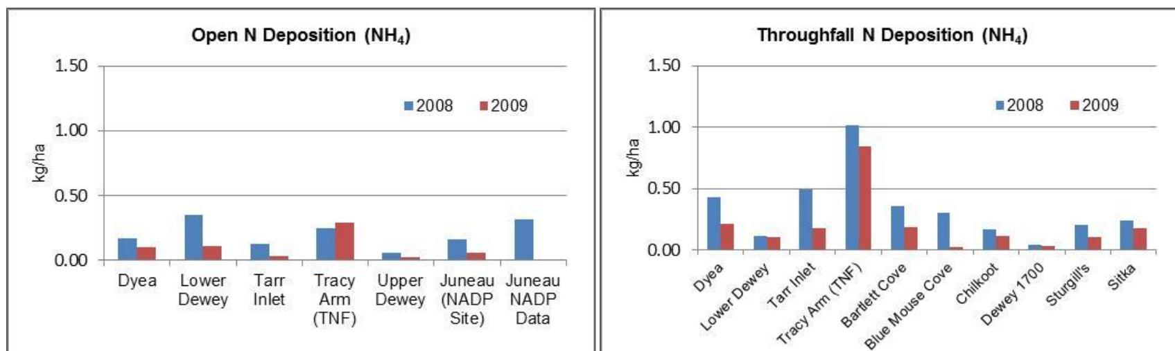
Figure 15. Open and throughfall deposition of \text{NH}_4^+ in 2008 and 2009. Note the Tracy Arm site's throughfall sampler was probably contaminated by bird droppings during the 2008 season.
