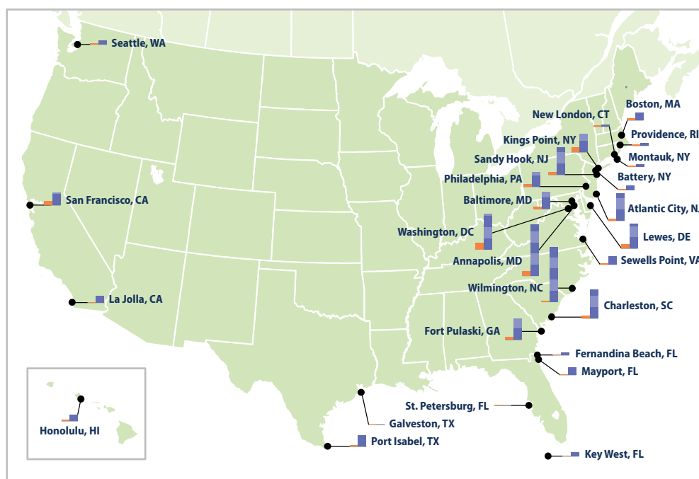
Frequency of Flooding Along U.S. Coasts, 2010–2015 Versus 1950–1959
