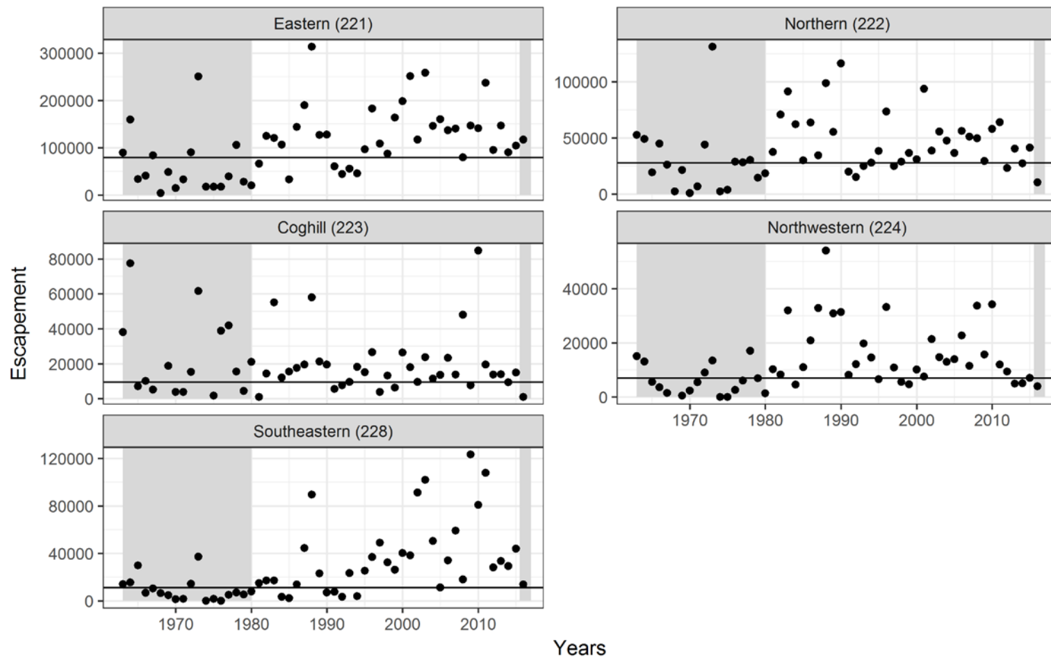
Figure 4.—Annual escapement estimates (dots) for PWS wild chum salmon and 20th percentile (line) of escapements (1963–2016) for districts; district numbers in parentheses.
