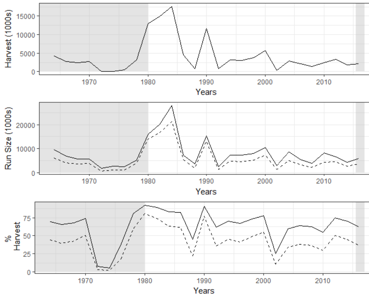
Figure 5.—Estimated harvest, high and low estimates of run size, and high and low estimates of harvest rate (% harvest of run) for even year wild pink salmon in PWS.
