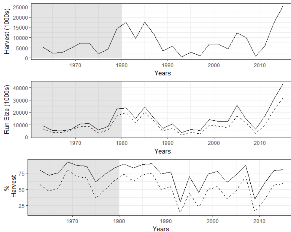
Figure 7.—Estimated harvest, high and low estimates of run size, and high and low estimates of harvest rate (% harvest of run) for odd year wild pink salmon in PWS.
