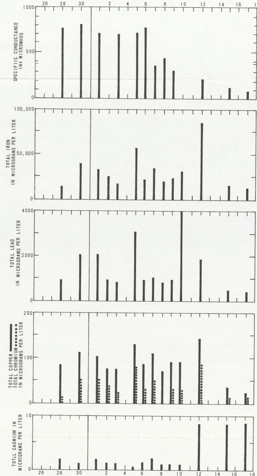
Concentration of Selected Chemical Constituents in Snowmelt Runoff from Brentwood Subdivision, 1975
