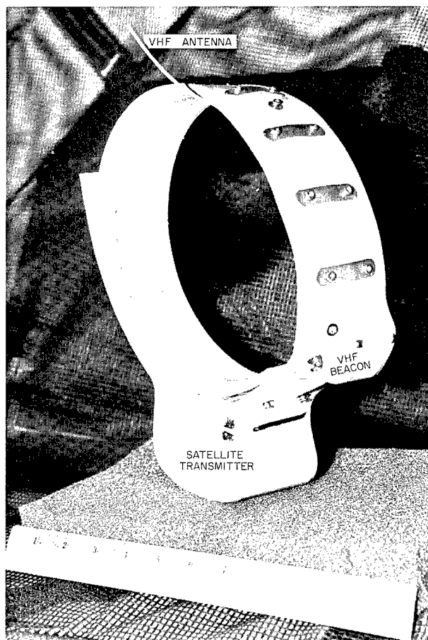
Fig. 24. Third-generation transmitter built by Telonics, Inc. This particular platform transmitter terminal (PTT) is configured for a polar bear and weighs 2 kg.
