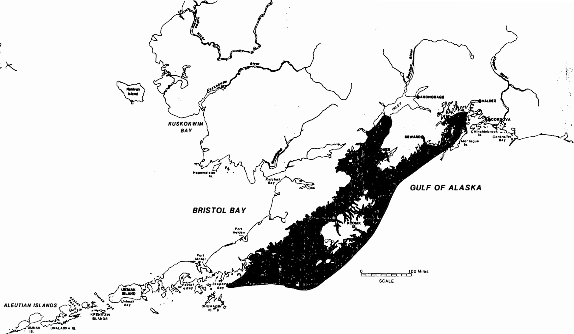
Outer Limits of Observed Sheens, Tar Balls, And Mousse Suspected To Be From The Exxon Valdez As Of August 10
