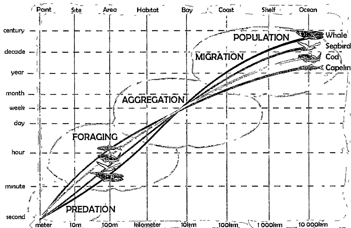
Figure 4.6 Scales of time and space corresponding to key elements and processes in ecosystems of the GOA. Illustration provided by John Platt
