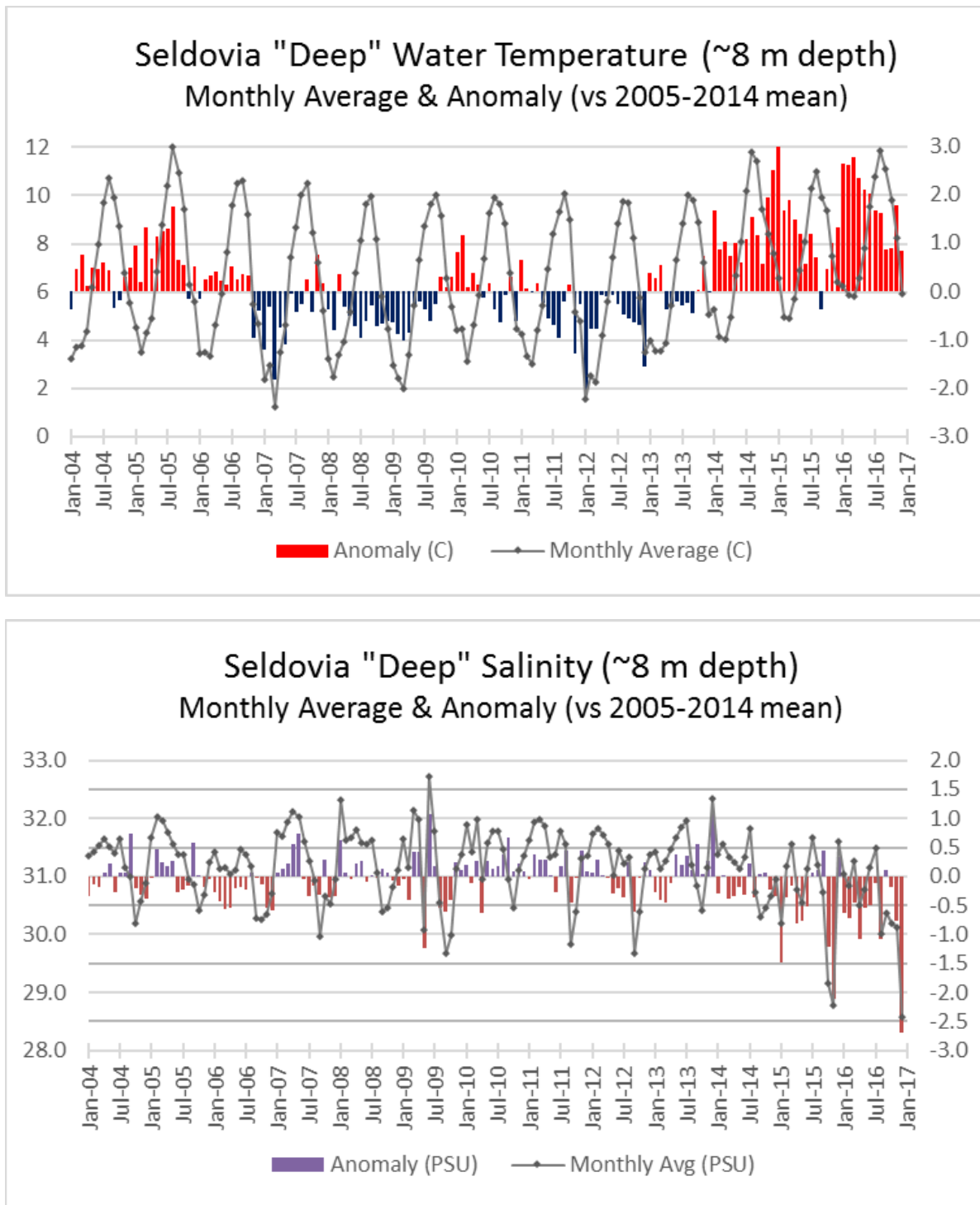
Figure 4. Monthly average (lines) and monthly anomaly (colored bars) for temperature (top) and salinity (bottom) calculated from near-bottom sensor data collected at the Seldovia SWMP water quality station during 2004 – 2016. The monthly anomalies were calculated against a 2005-2014 monthly climatology for comparison with other GWA datasets. Positive/negative anomalies are shown for temperature (red/blue) and salinity (purple/maroon).
