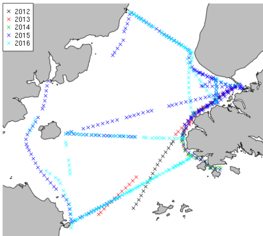
Figure 15. Marine bird and mammal transects, 2012–2016, conducted by USFWS observers on NOAA KBL/KBNER shipboard surveys in lower Cook Inlet and Kachemak Bay.
