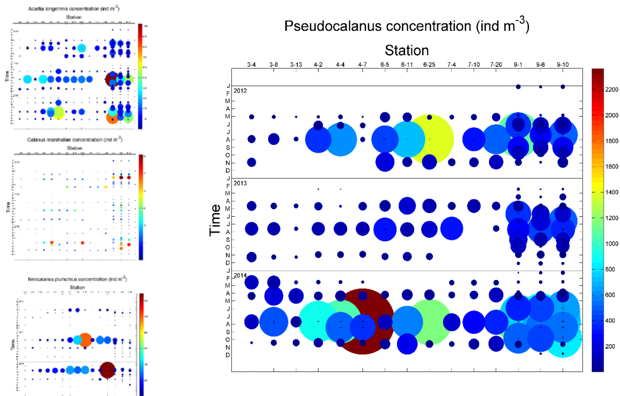
Figure 11. Proportional copepod abundance for species of interest in the Gulf of Alaska Pseudocalanus spp. Acartia longiermis , Calanus marshallae and Neocalanus plumchrus concentrations (individuals m^{-3} ) observed during 2012-2014 at stations (numbers on x-axis) across the study area. Both the size and color of the dots are proportional to copepod abundance. Station numbers identify transects in Kachemak Bay (Transects 4 and 9) and lower Cook Inlet (Transects 3, 6, and 7), with plankton sampled at three stations on each transect. Mid-Kachemak Bay stations (Transect 9) are sampled monthly, while other transects are sampled quarterly.
