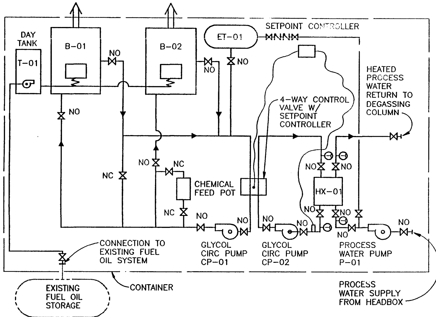
PROCESS FLOW SCHEMATIC
