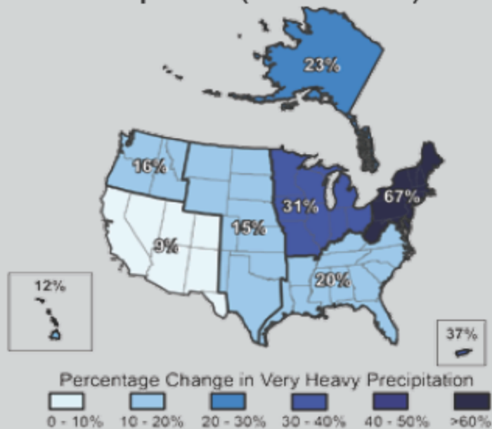
Increases in Amounts of Very Heavy Precipitation (1958 to 2007)
