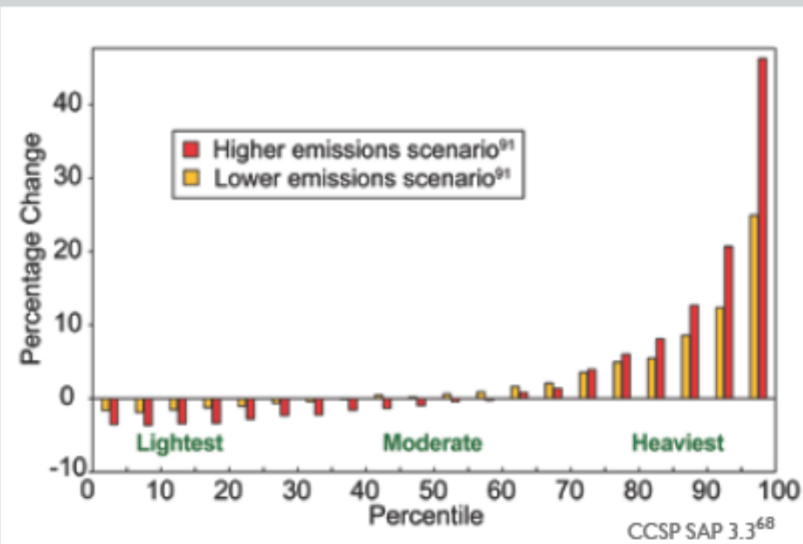
Projected Changes in Light, Moderate, and Heavy Precipitation (by 2090s)
