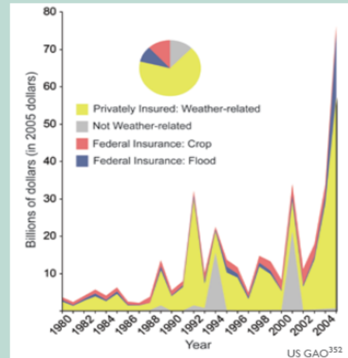
Insured Losses from Catastrophes, 1980 to 2005
