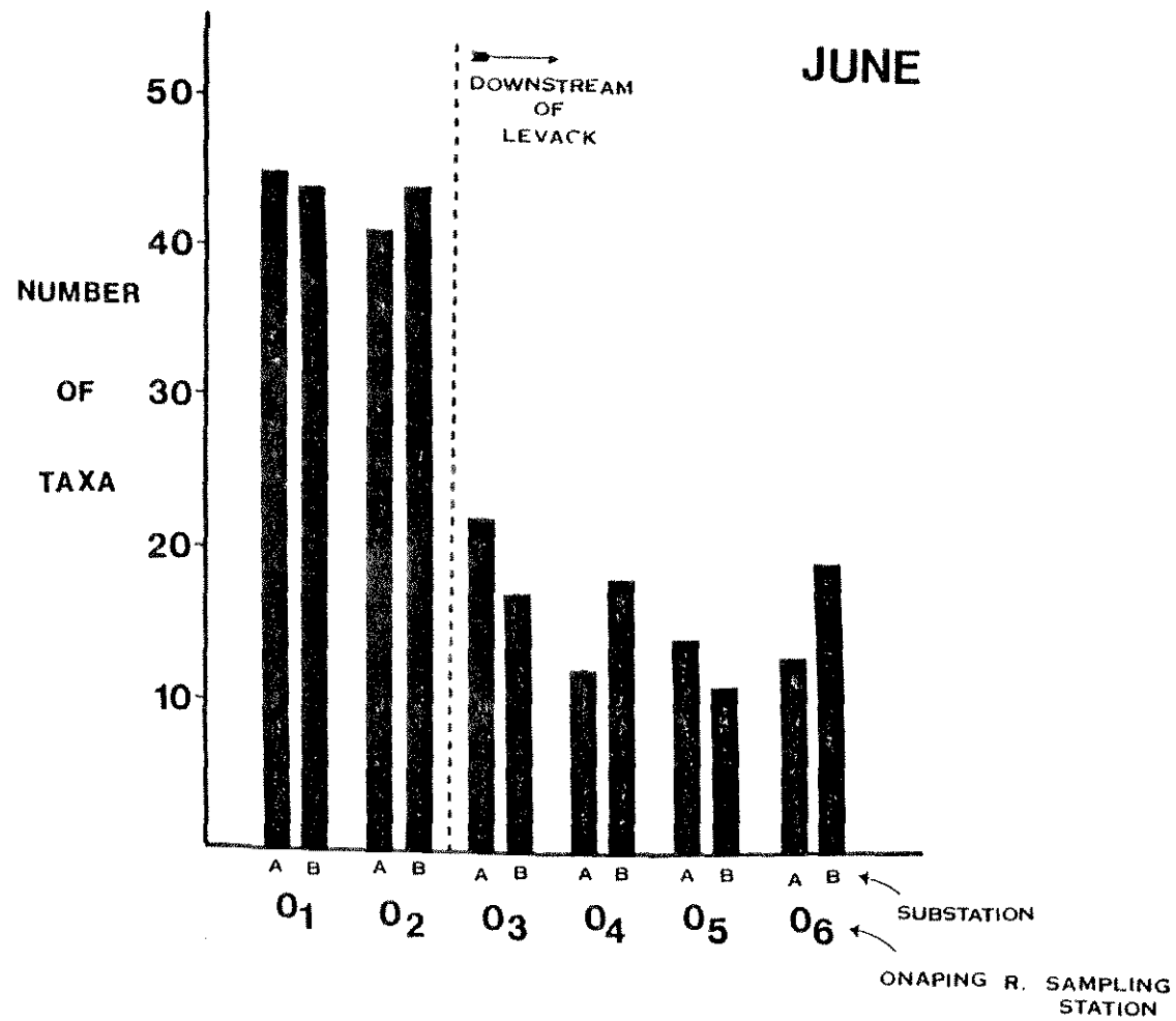
Figure 5. Total number of taxa of benthic macroinvertebrates found in the Onaping River during June of 1977. (Results are from 3 Surber samples and 1 grab sample/substation.)
