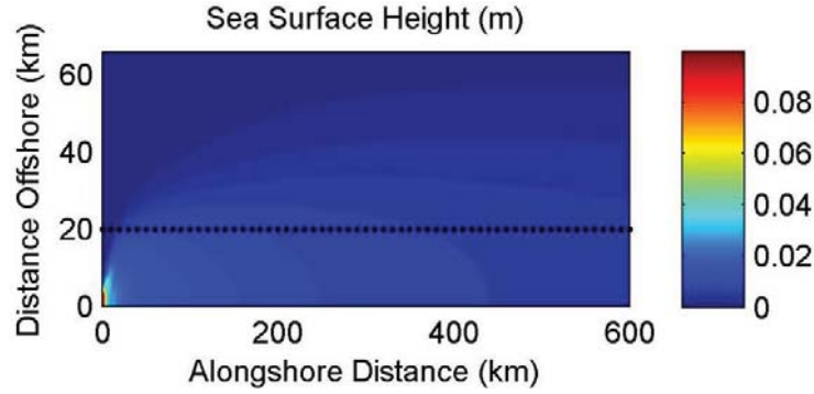
Figure 4. Analytical landfast ice covered model solution. The dotted line at ~20 km offshore marks the edge of the landfast ice. Inshore of the ice edge the ice is modeled as a constant (in space) surface friction. Offshore of the ice edge the surface friction coefficient is 0.
