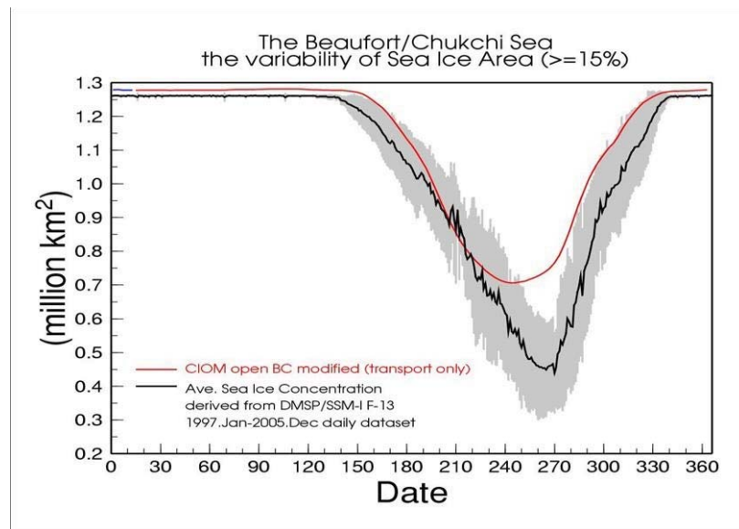
Figure 5. Model-data comparison: Satellite-measured (black) and model-simulated (red) sea ice cover; For more details of the satellite products prepared for validation of CIOM, please go to: http://www.frontier.iarc.uaf.edu/~jwang/SatelliteProducts .
