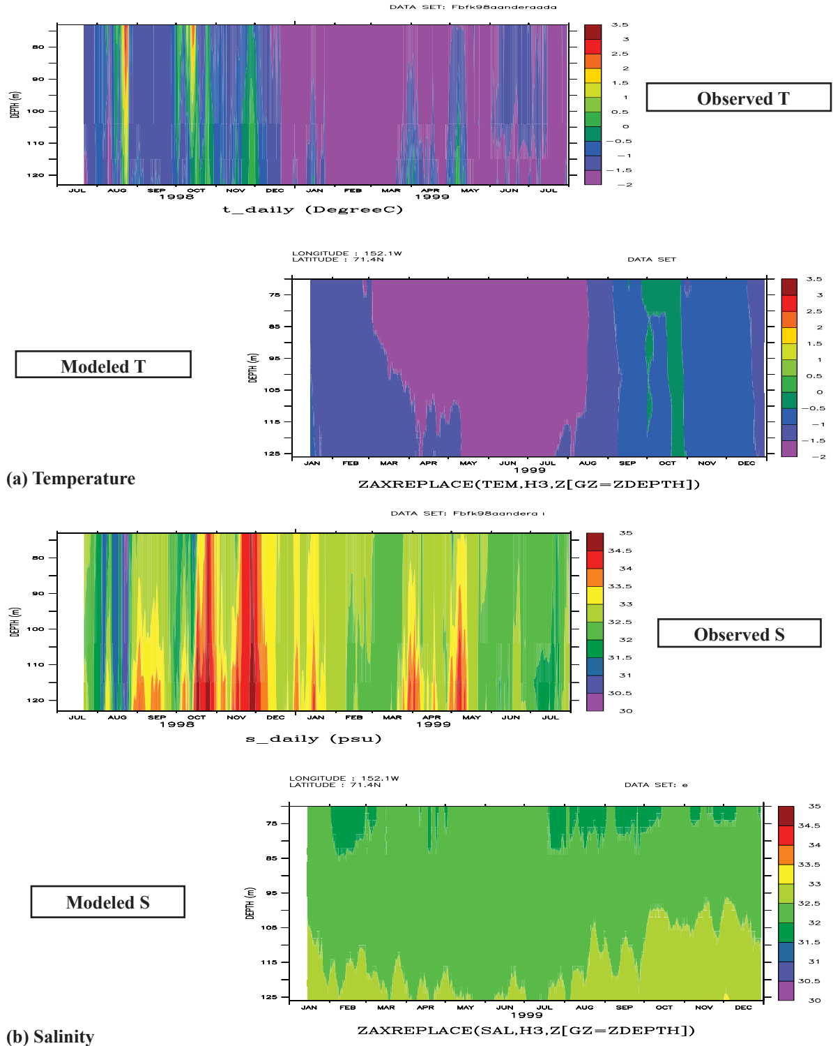
Figure 7. Time-depth comparison of observed (upper) and modeled (lower) temperature (a), salinity (b), and velocity, u and v (c) at BFK98 (station 10). The model captures the mean state, with less variability for all the variables.
