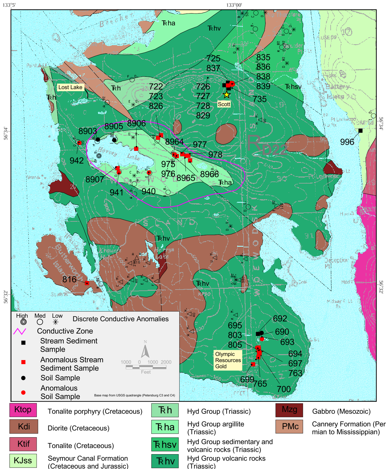
Figure 40. Anomalous Area 8 with stream sediment and soil samples, geology (Karl and others, 1999), conductive zones (Pritchard, 1997), and discrete anomalies (ADGGS and others, 1997).
