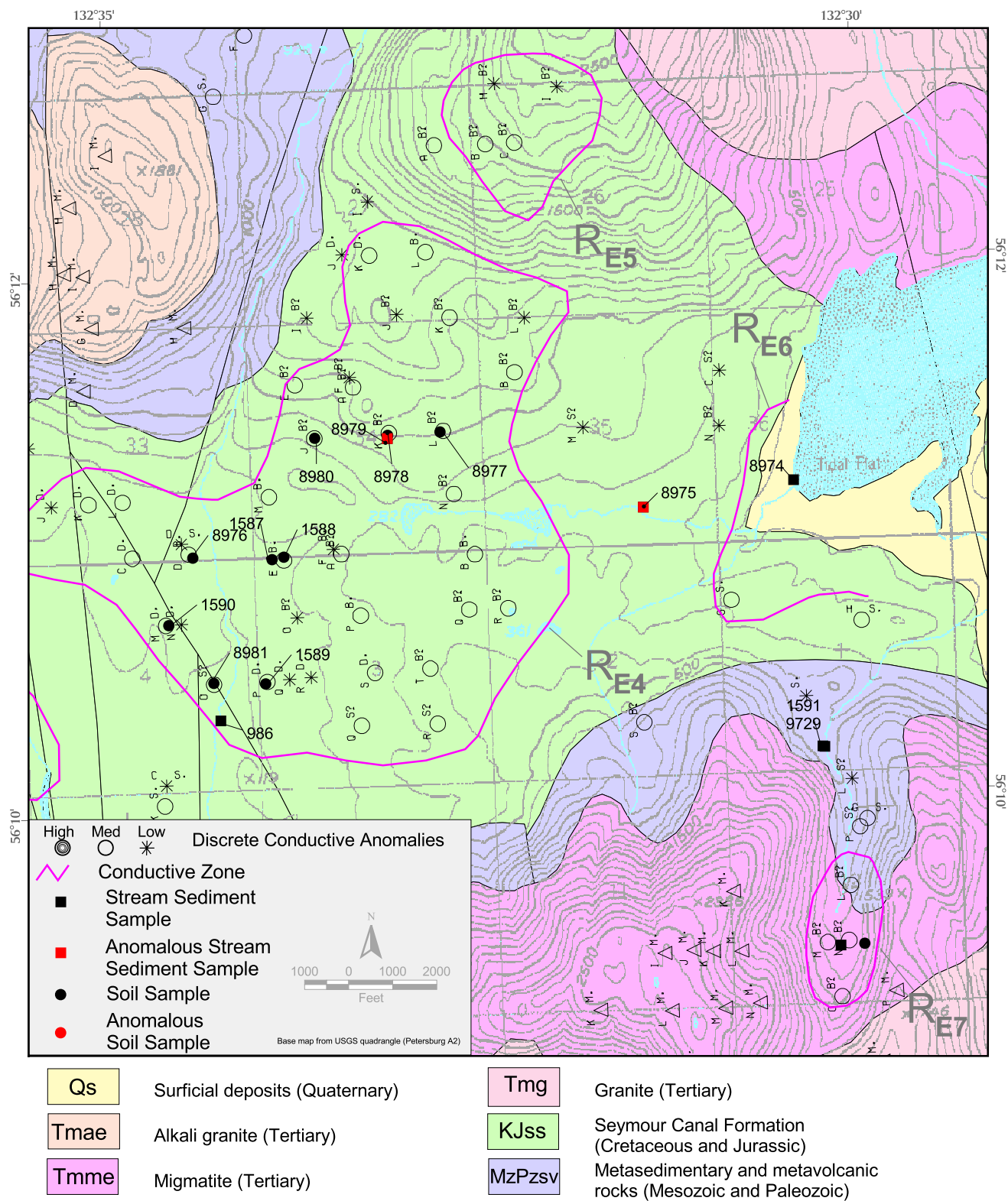
Figure 42. Anomalous Area 10 with stream sediment and soil samples, geology (Karl and others, 1999), conductive zones (Pritchard, 1997), and discrete anomalies (ADGGS and others, 1997).
