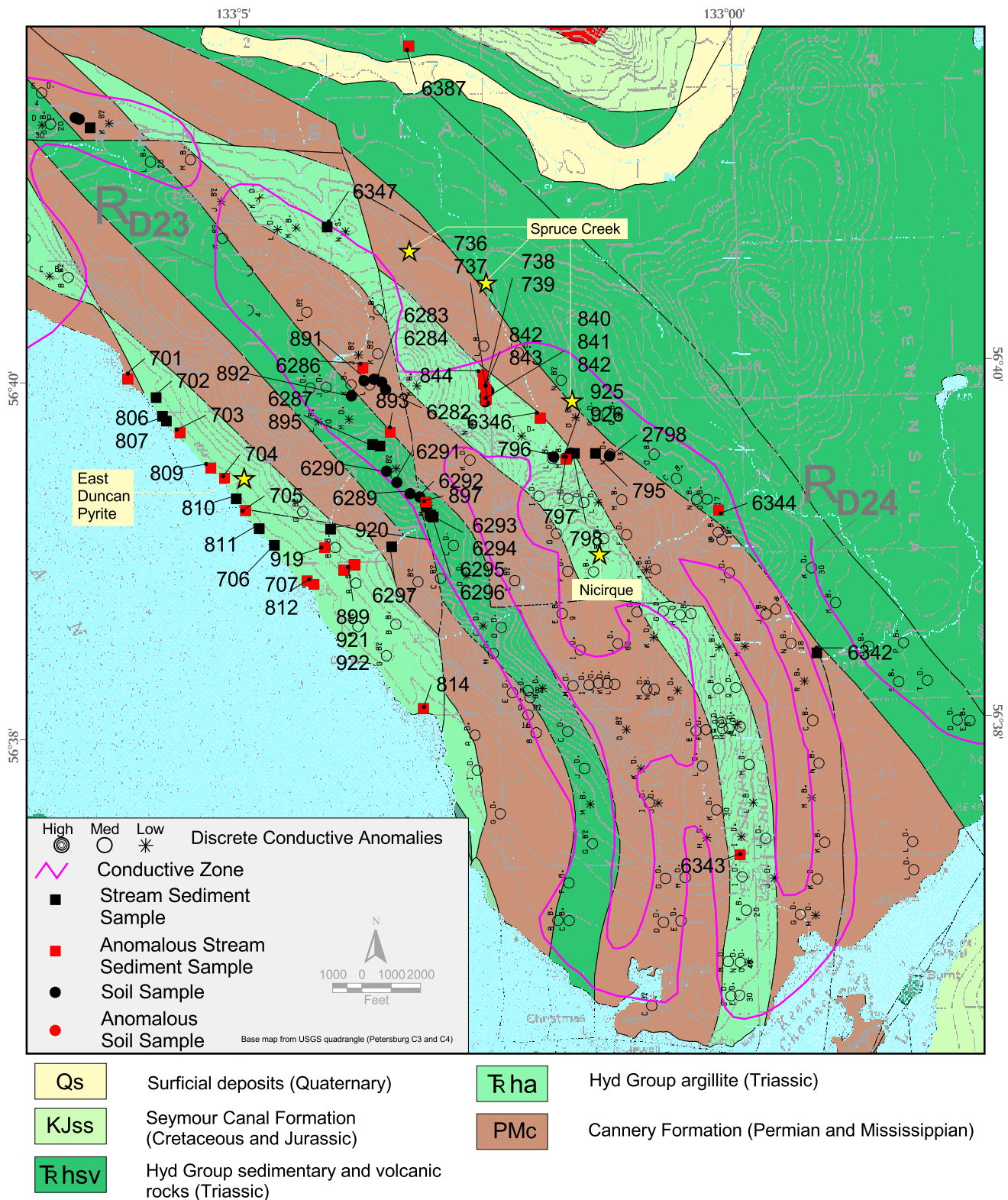
Figure 37. Anomalous Area 5 with stream sediment and soil samples, geology (Karl and others, 1999), conductive zones (Pritchard, 1997), and discrete anomalies (ADGGS and others, 1997).
