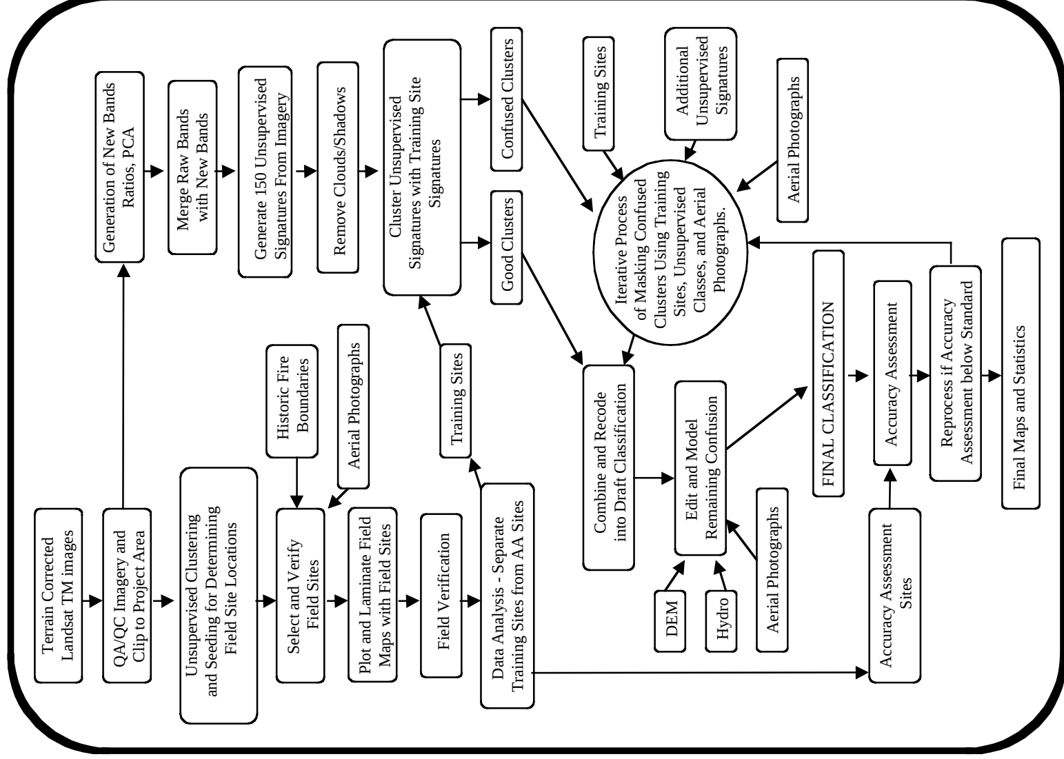
Figure 7. The image processing flow diagram
