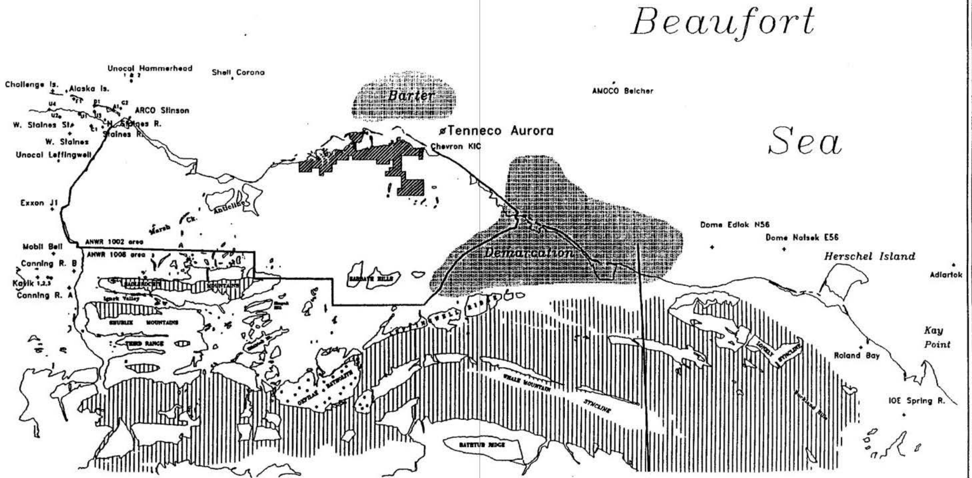
Figure 2 Aurora well location, outcrops and major geographic features including ANWR 1002 area and nearest exploration wells
