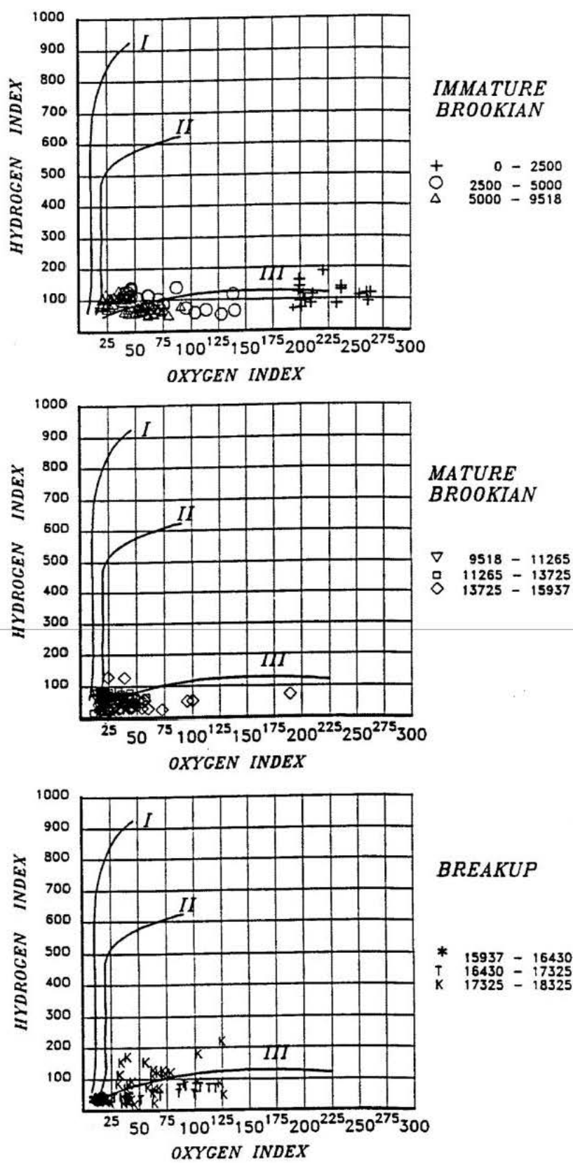
Figure 5 Modified van Krevelen diagrams showing kerogens from the three major stratigraphic divisions at Aurora well
