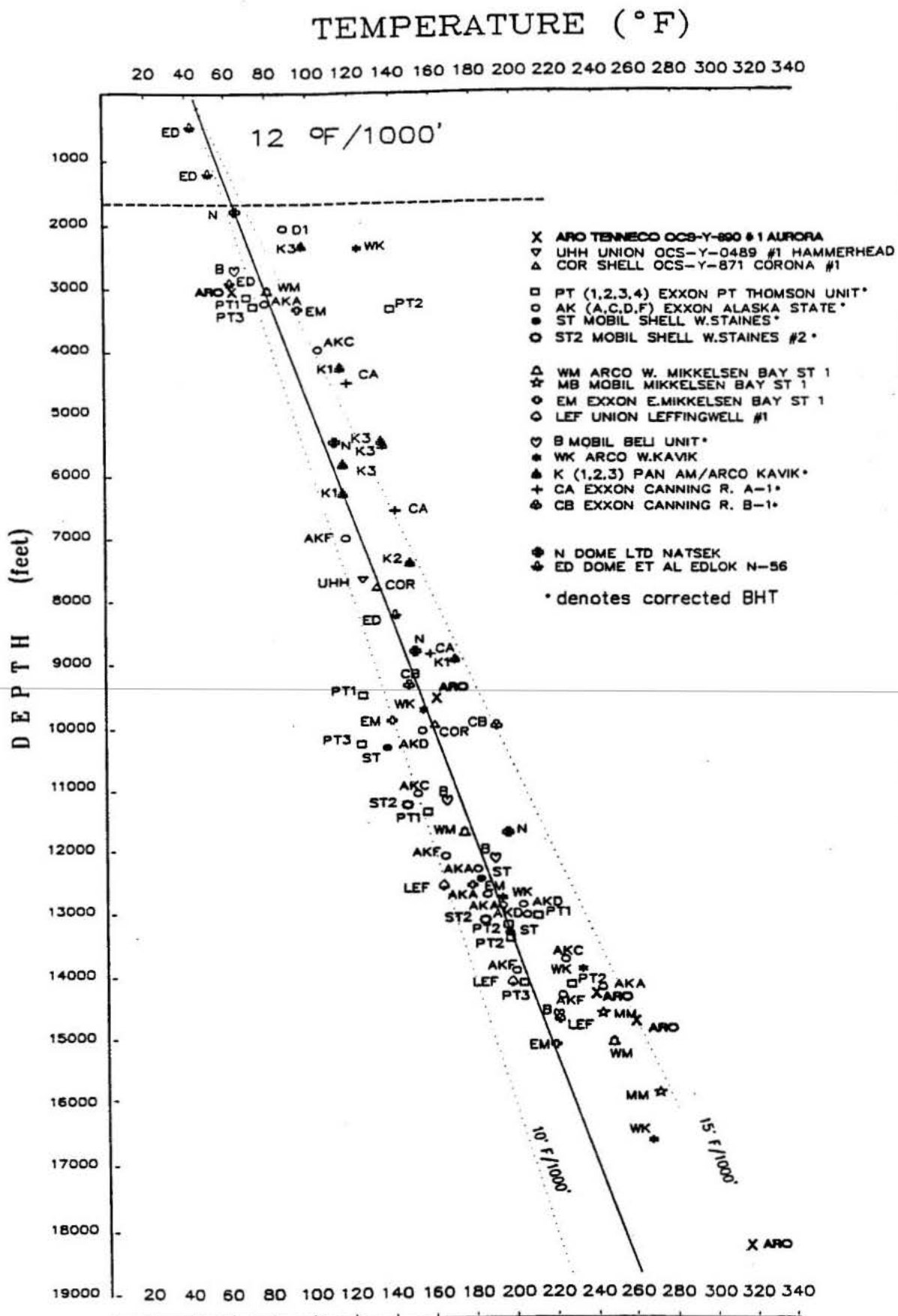
Figure 7 Temperature gradients from Aurora and nearby wells
