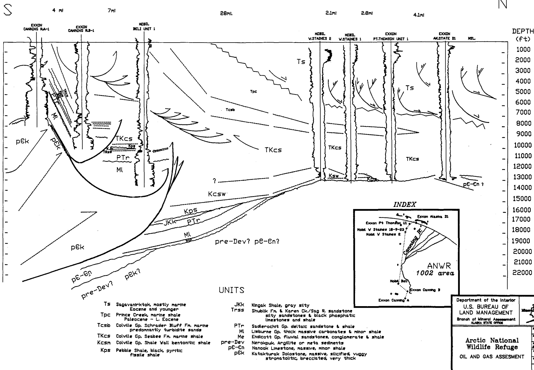
PLATE 1 GENERALIZED GEOLOGIC CROSS SECTION SHOWING STRAGITRAPHY, PREDDOMINANT FAULTING STYLES AND MAJOR UNCONFORMITIES PROJECTED FROM WELLS WEST OF ANWR
