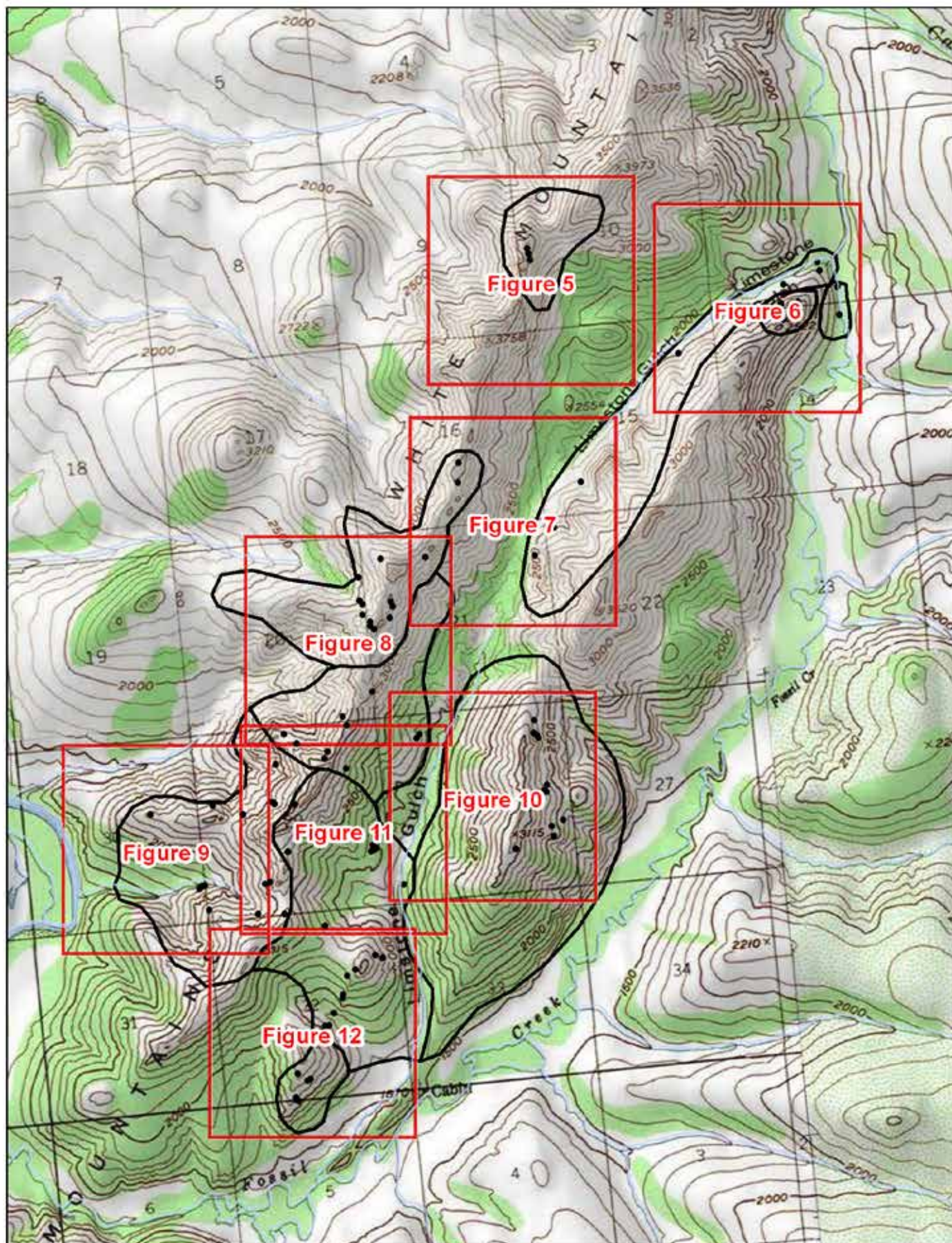
Figure 3. Boundary extents of the eight surveys in the White Mountains National Recreation Area, plus all karst feature locations. (1) 5/23/03 – 5/25/03; (2) 6/06/03 – 6/09/03; (3) 7/03/03 – 7/04/03; (4) 8/02/03 – 8/04/03; (5) 6/05/04 – 6/07/04; (6) 7/16/05 – 7/18/05; (7) 8/27/05 – 8/29/05; (8) 7/22/02 – 7/23/02.
