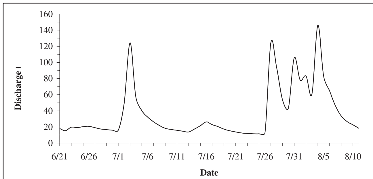
Figure 2. Daily discharge ( \text{m}^3/\text{s} ) for the period 21 June – 11 August 2003, Tozitna River, Alaska.
