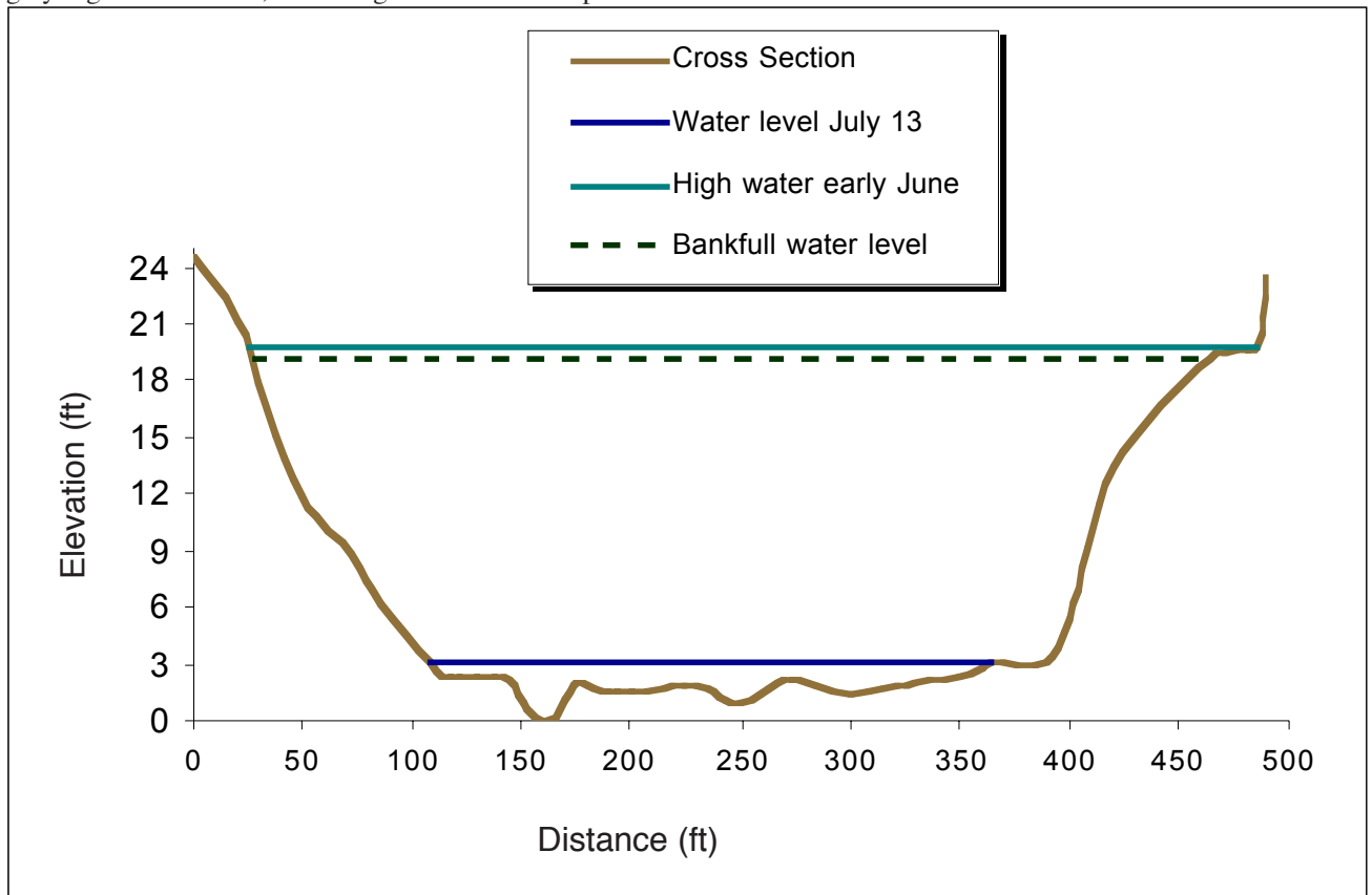
Figure A-29. Channel cross section for the Awuna River near the mouth.
