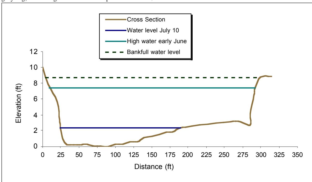
Figure A-19. Channel cross section for the Ipnarik River.
