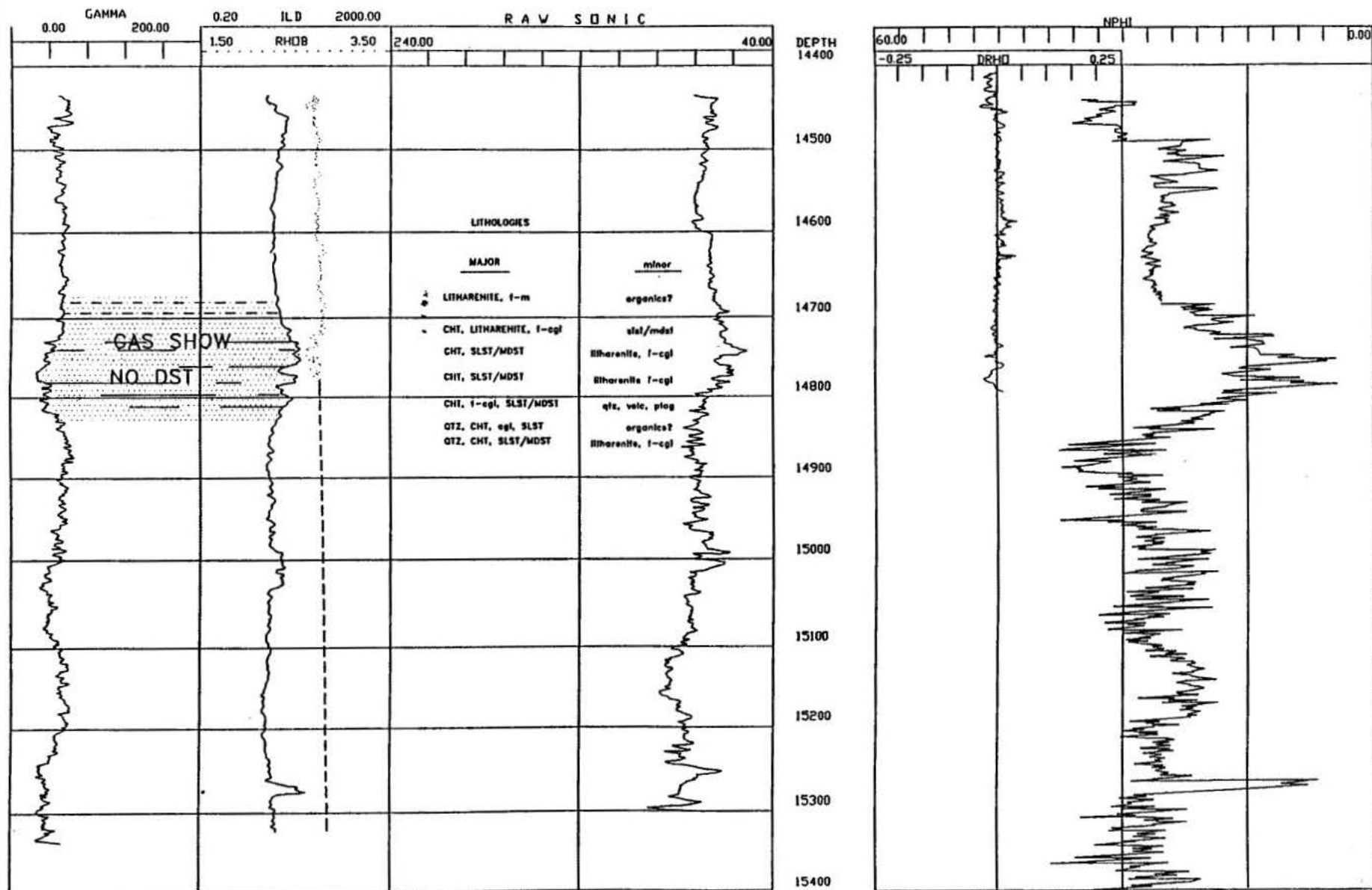
Figure 6. Geophysical logs through the Oruktalik unit and sample descriptions.
