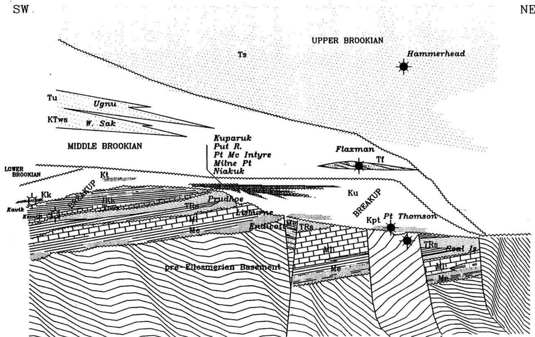
Figure 5. Generalized SW-NE cross section, superimposing major North Slope petroleum traps.
