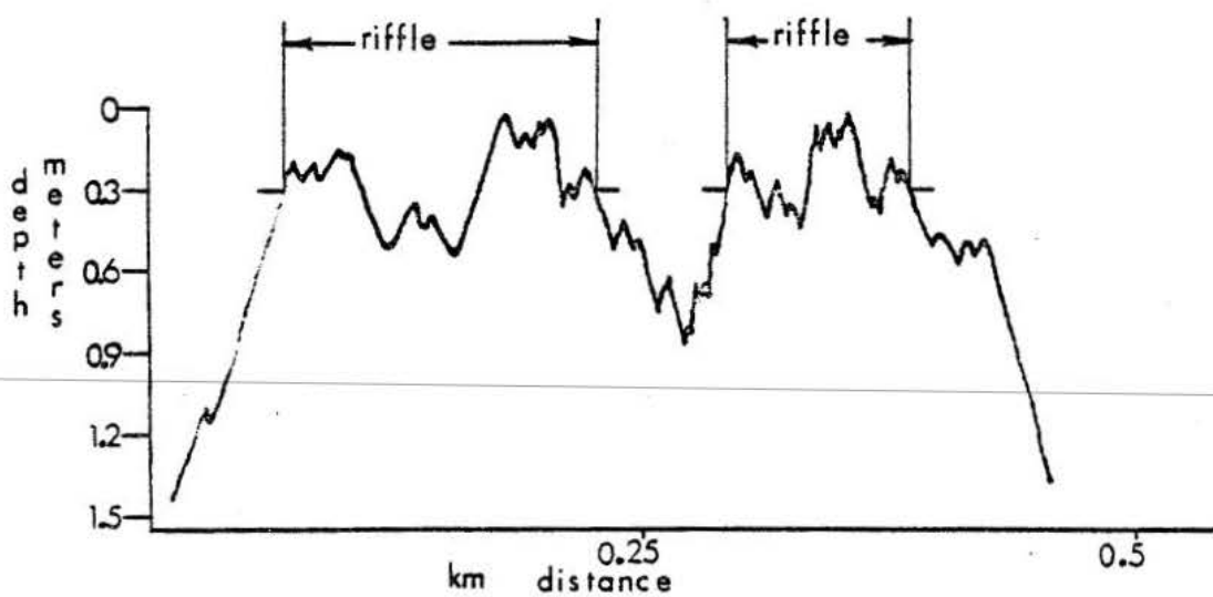
Figure 3. Illustration of fathometer record analysis / interpretation for riffles.
