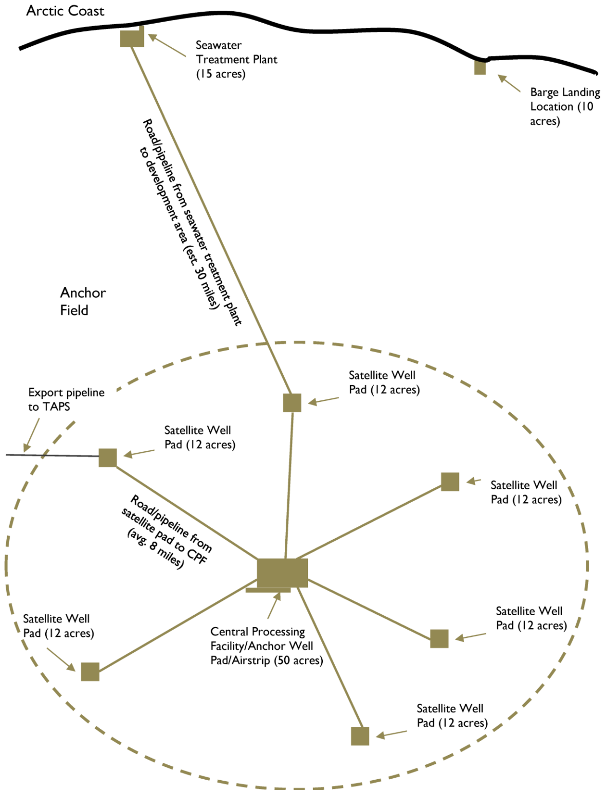
Figure B-I. Conceptual Layout of a Stand-Alone Oil Development Facility*
