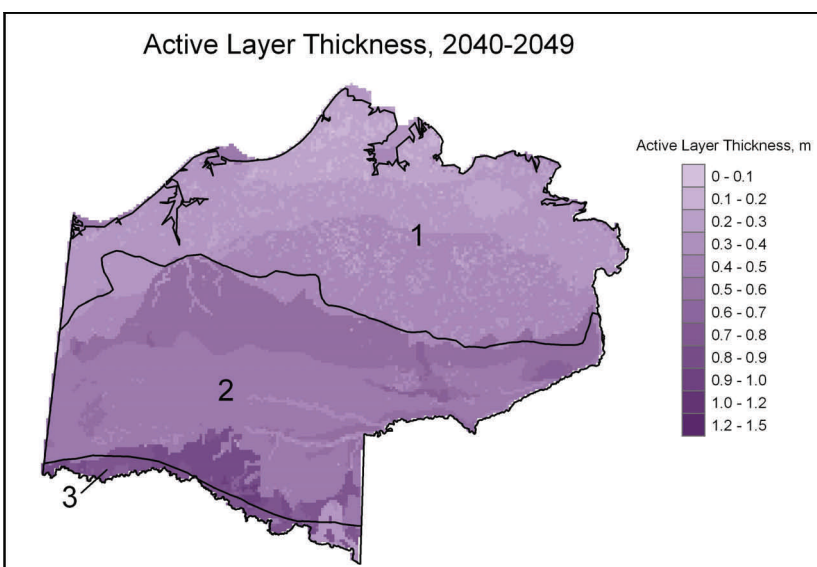
Figure 9 –Projections for depth of active layer, 2040-2049. Modest increases in summer thaw depths are projected by the middle of this century. Such changes may trigger shifts in hydrology and vegetation. Region 1 is the Coastal Plains, Region 2 is the Foothills, and Region 3 is the Mountains.
