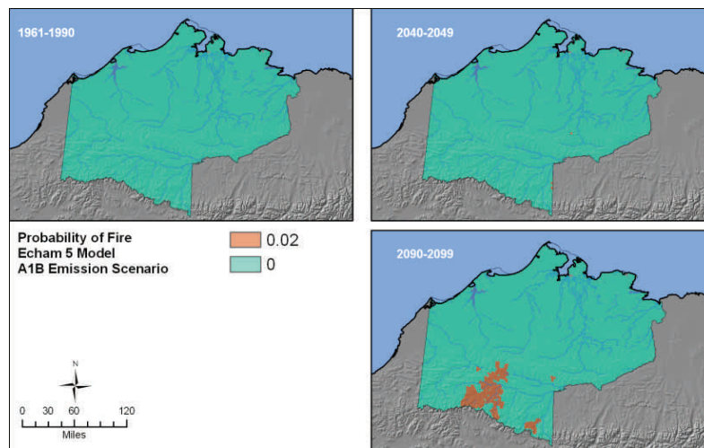
Figure 11 – Probability of fire, per year, based on the ALFRESCO spatially explicit fire model.
