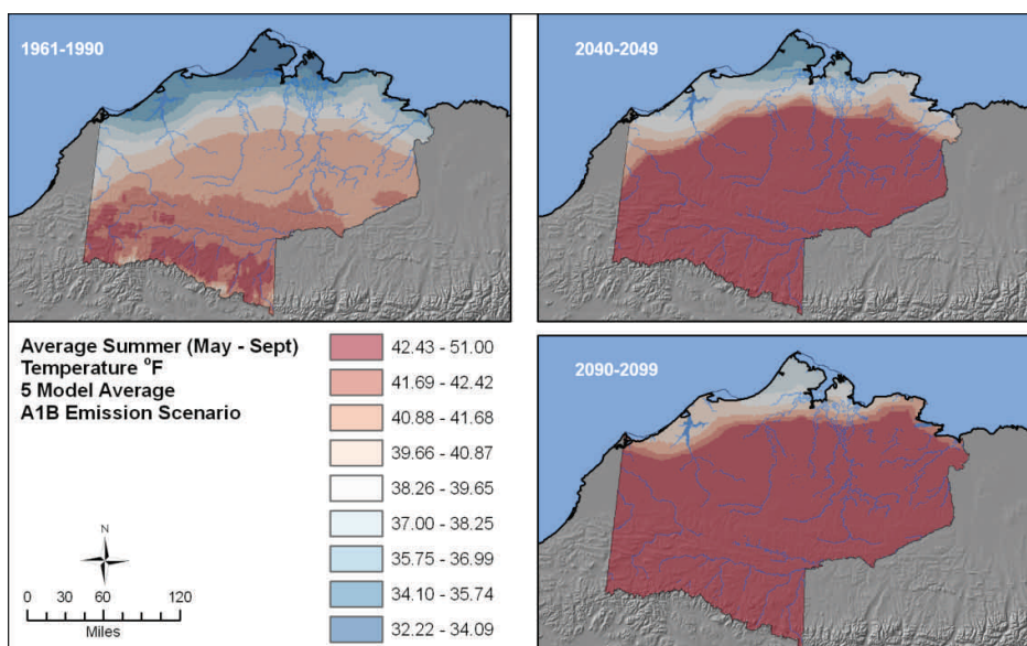
Figure 2: Summer Temperature Projections. “Summer” refers to averages for May through September.
