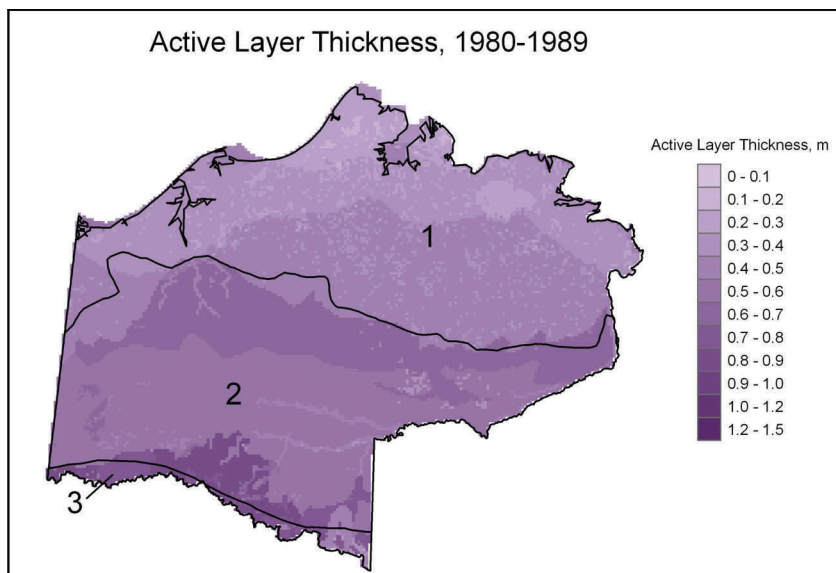
Figure 8 – Historic estimates of depth of active layer, 1980-1989. Active layer represents maximum thaw depths at the end of the summer season, and affects hydrology and vegetation. Region 1 is the Coastal Plains, Region 2 is the Foothills, and Region 3 is the Mountains.
