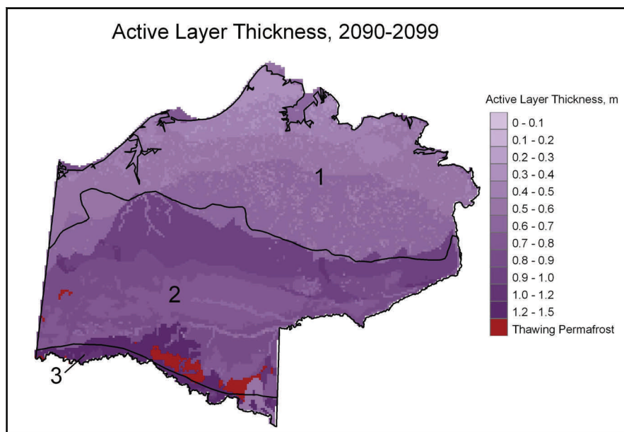
Figure 10 –Projections for depth of active layer, 2090-2099. In some mountainous regions of the NPR-A, loss of shallow permafrost is possible by the end of the century. Region 1 is the Coastal Plains, Region 2 is the Foothills, and Region 3 is the Mountains.
