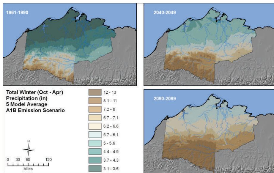
Figure 5: Winter Precipitation Projections. “Winter” refers to averages for October through April
