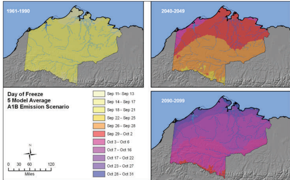
Figure 7: Autumn freeze-up projections. Day of freeze is defined, for the purposes of this analysis, as the day at which the running mean temperature crossed the freezing point of fresh water.
