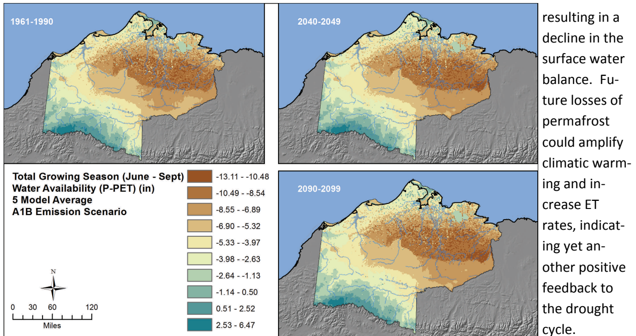
Figure 13: Predicted difference between Precipitation (P) and Potential Evapotranspiration (PET) during the growing season. P-PET is expected to remain negative throughout the century for much of the NPR-A, with the exception of the mountains to the south.
