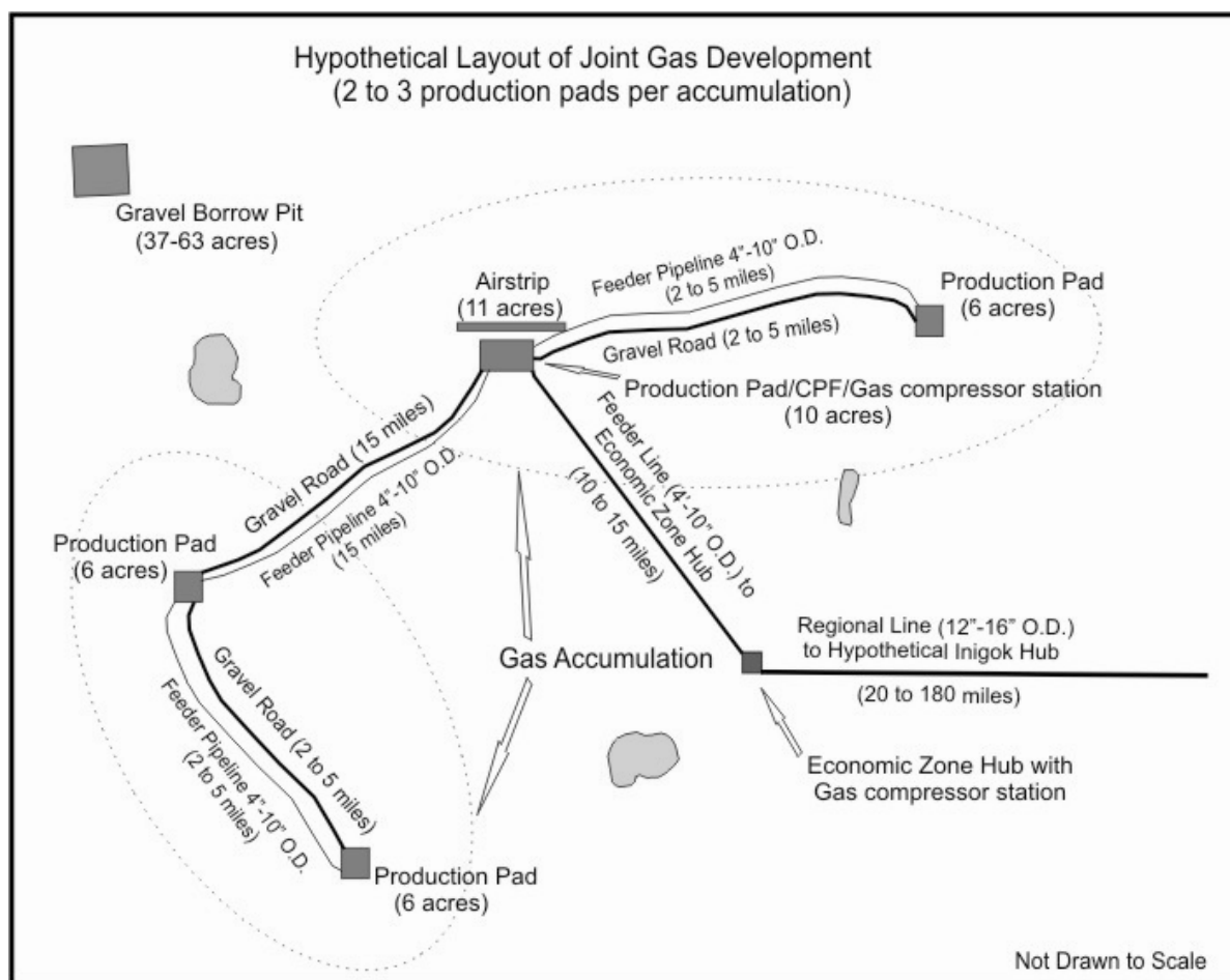
Figure 4—6. Hypothetical layout of joint gas development
