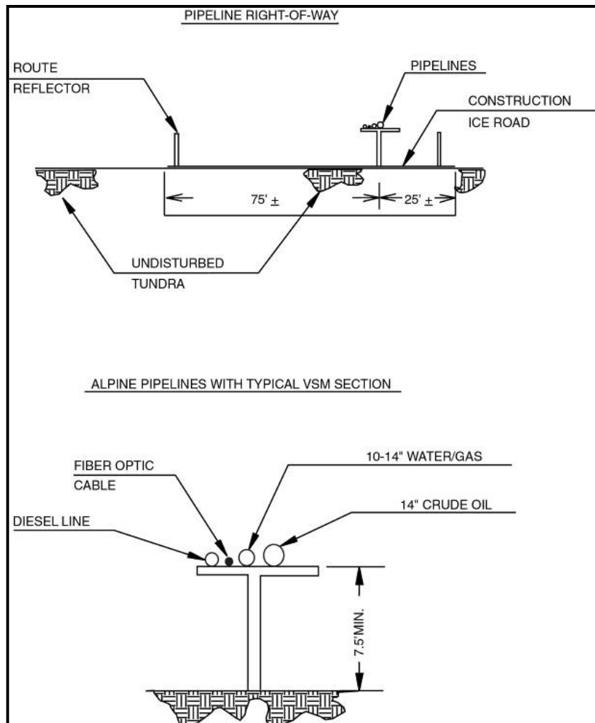
Figure 4—8. Sample oil pipeline layout
