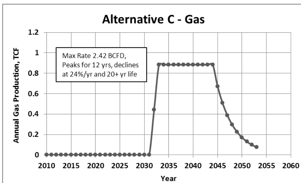
Figure 4—20. Assumed annual undiscovered nonassociated gas production rate for Alternative C
