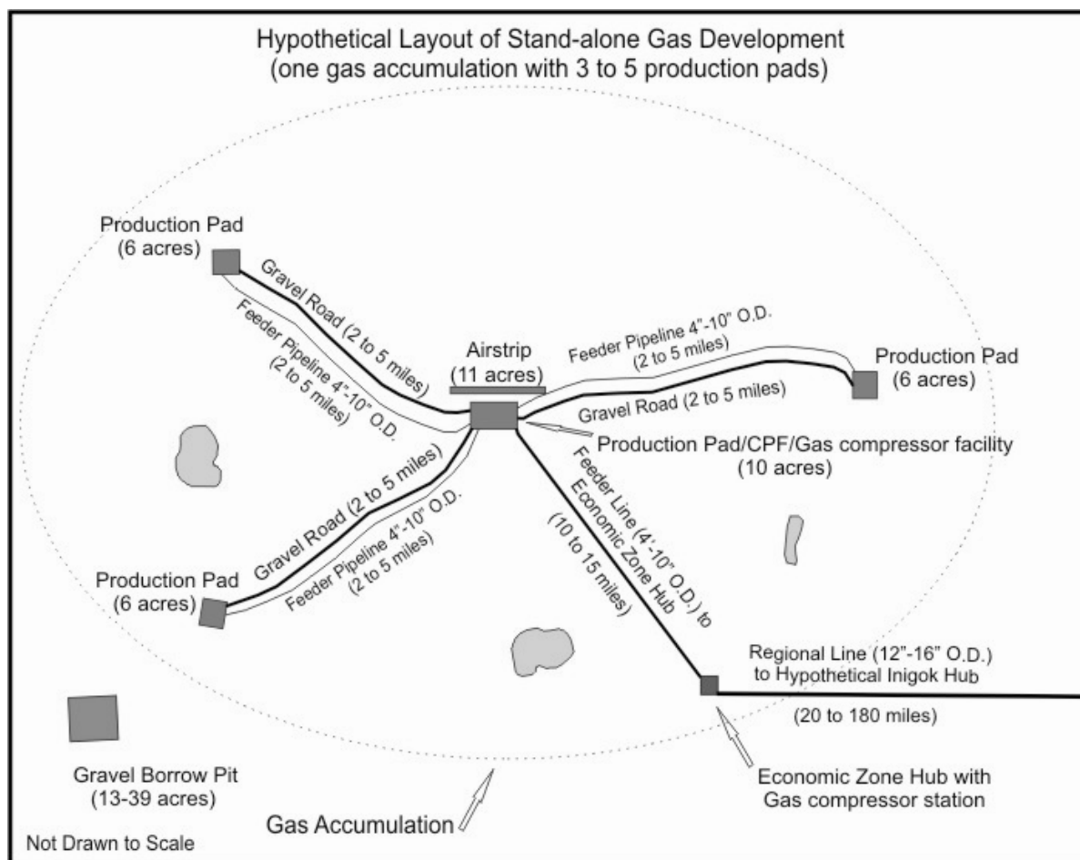
Figure 4—7. Hypothetical layout of stand-alone gas development
