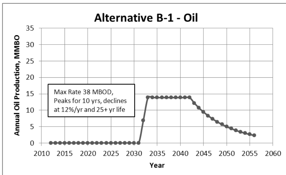
Figure 4—15. Assumed annual undiscovered oil production rate for Alternative B-1
