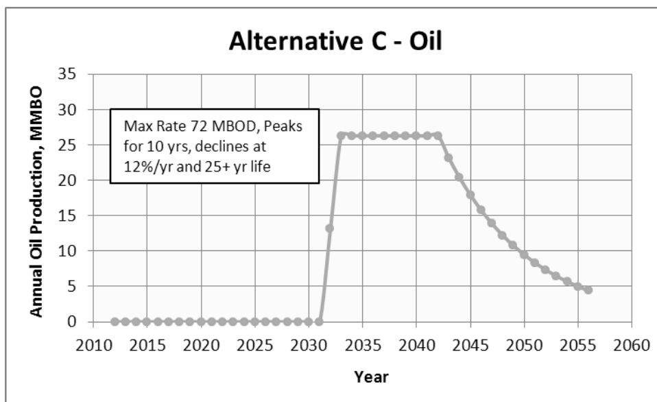
Figure 4—19. Assumed annual undiscovered oil production rate for Alternative C
