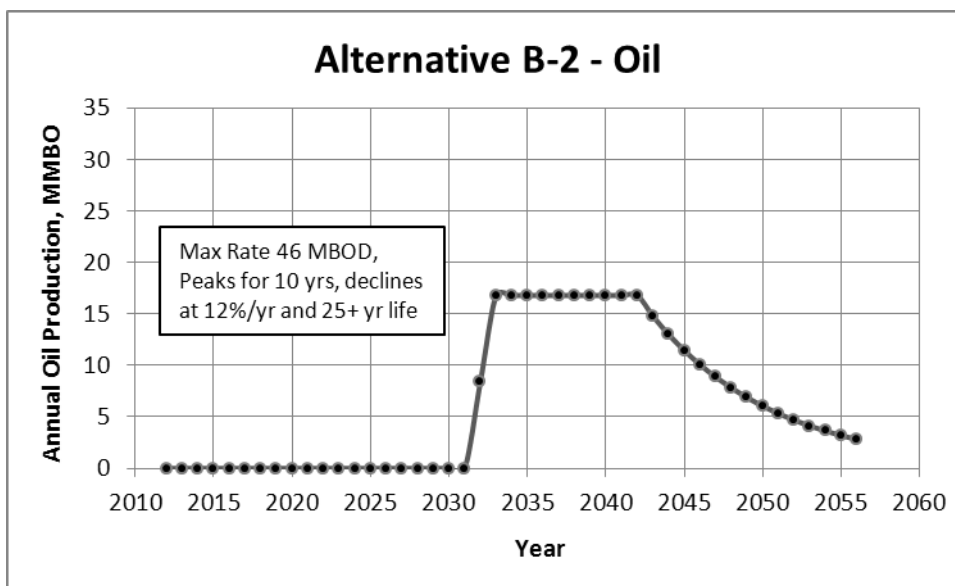
Figure 4—17. Assumed annual undiscovered oil production rate for Alternative B-2
