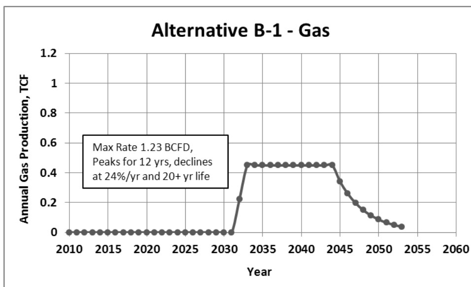
Figure 4—16. Assumed annual undiscovered nonassociated gas production rate for Alternative B-1
