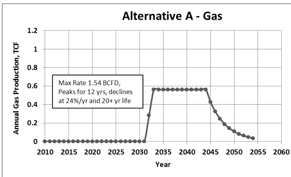
Figure 4—14. Assumed annual undiscovered nonassociated gas production rate in Alternative A
