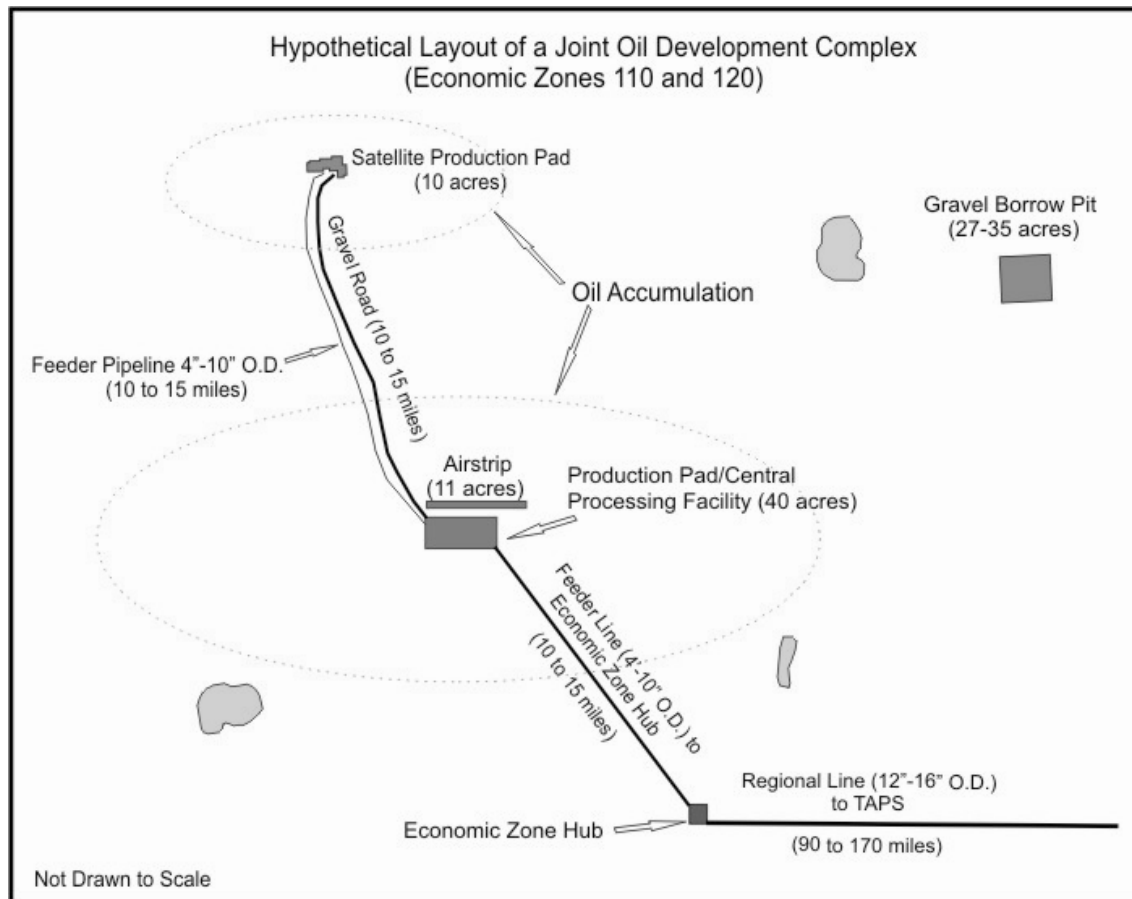
Figure 4—4. Hypothetical layout of a joint oil development complex
