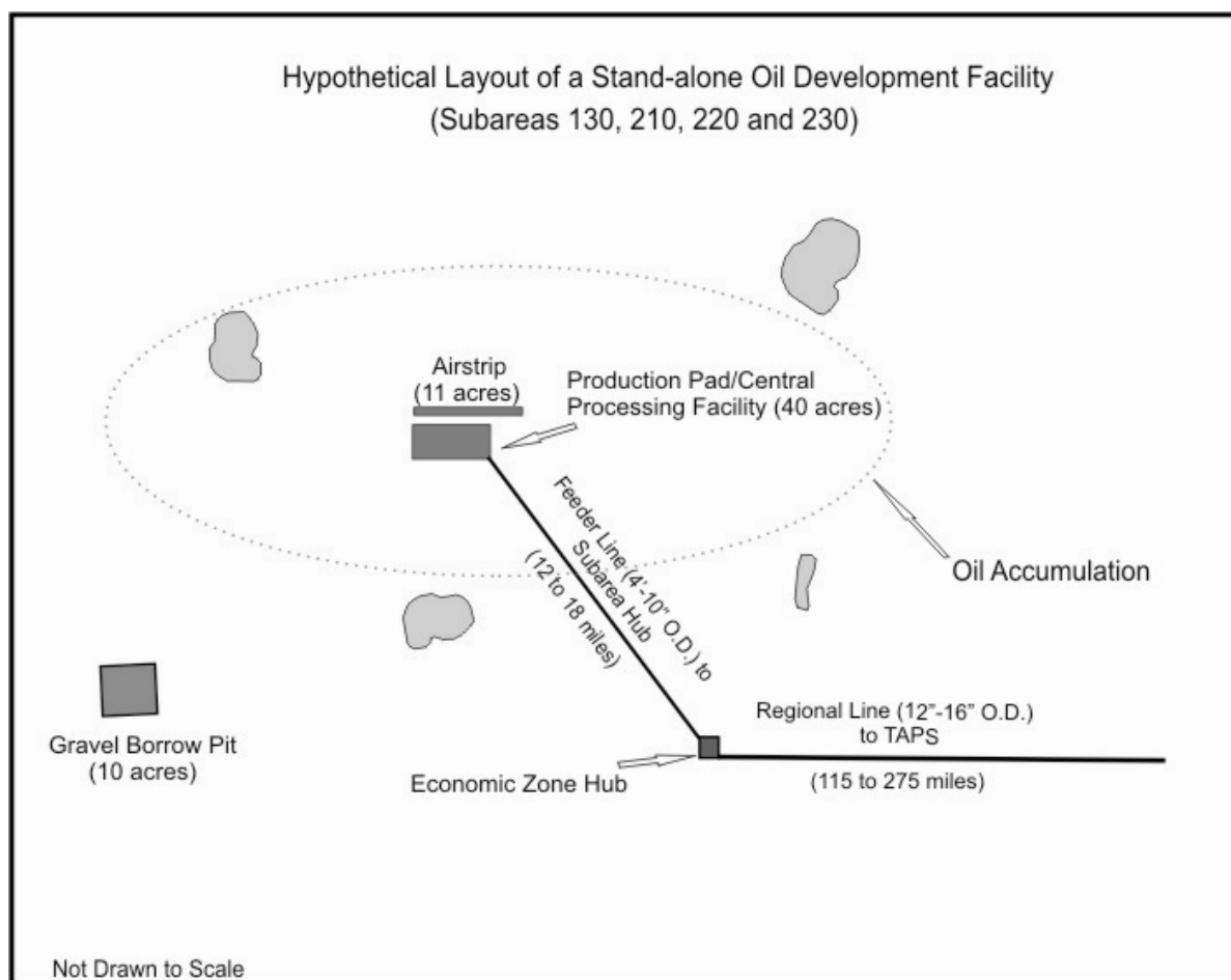
Figure 4—5. Hypothetical layout of a stand-alone oil development facility (TAPS = Trans-Alaska Pipeline System)
