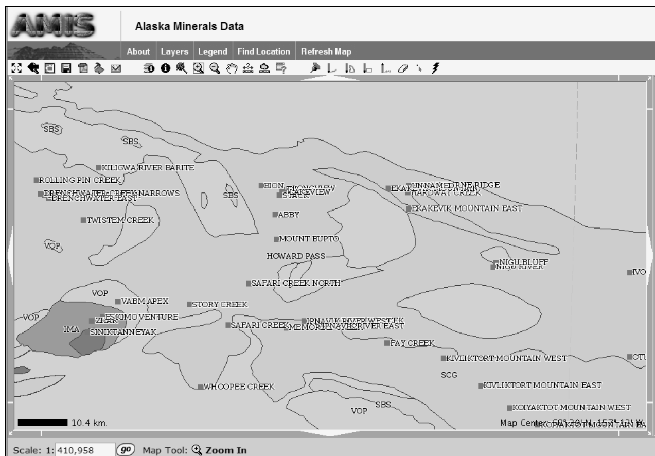
Figure 3-7. Screen capture map from the BLM's Alaska Minerals Information System site showing mineral terranes and Alaska Minerals Information System locations in the Howard Pass Quadrangle
