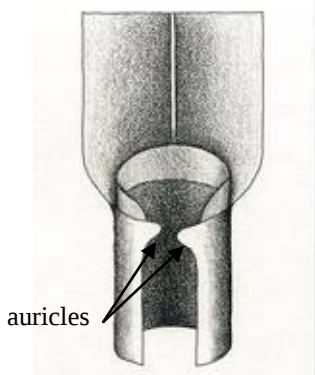
Figure 16: Schematic drawing of auricles; small, clasping outgrowths that may or may not be present on the leaf collar. © 2009 The Regents of the University of California
