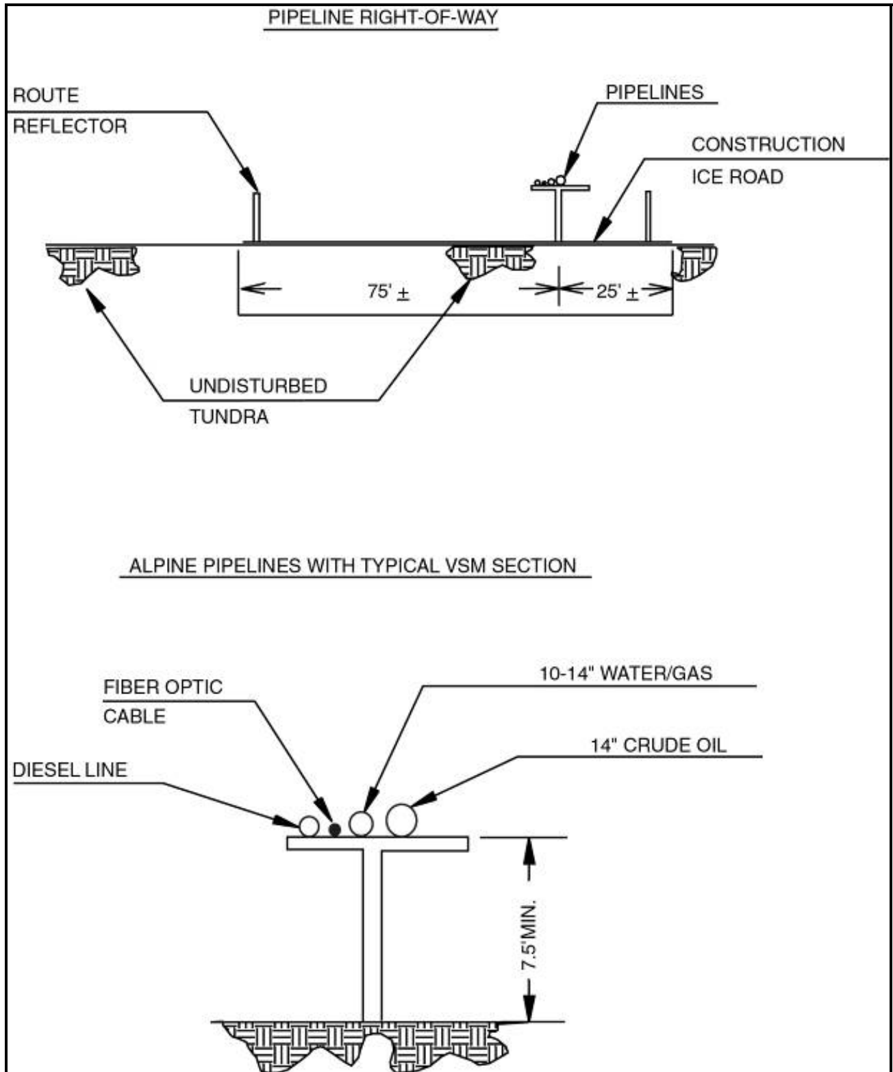
Figure 4-3. Sample Pipeline Layout
