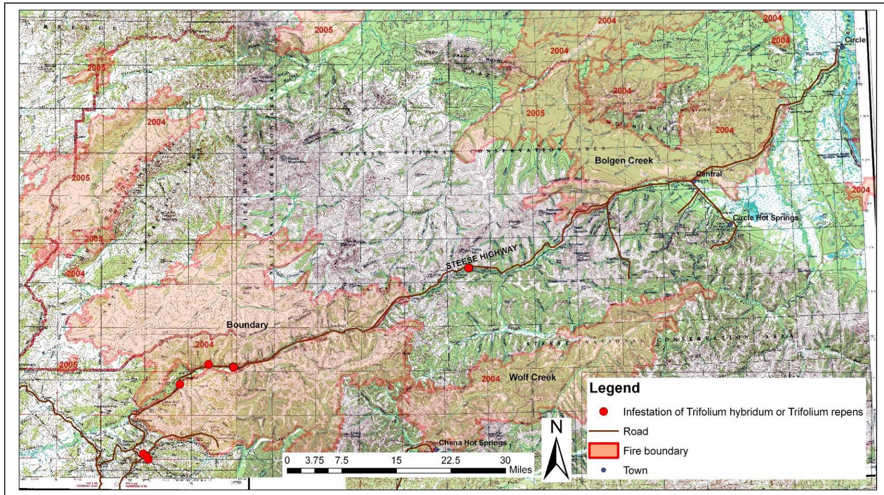
2006 infestations of white ( Trifolium repens ) and alsike clover ( T. hybridum ) along the Steese Highway.
