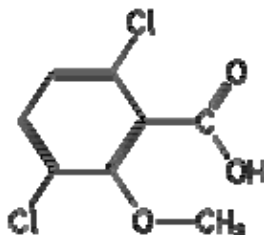
Dicamba Chemical Structure
