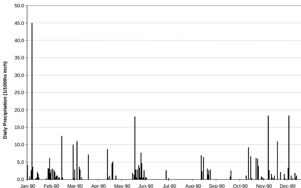
Figure D-1 Daily Rainfall Totals for 1990 at Medford, Oregon
