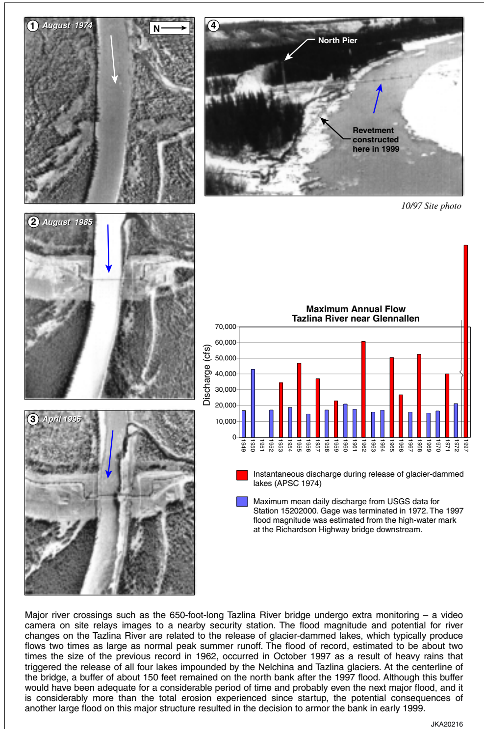
FIGURE 4.1-9 Tazlina River Bridge, MP 686, Where Monitoring Led to Bank Armoring to Prevent Further Erosion (Source: TAPS Owners 2001a, Figure 4.2-13)
