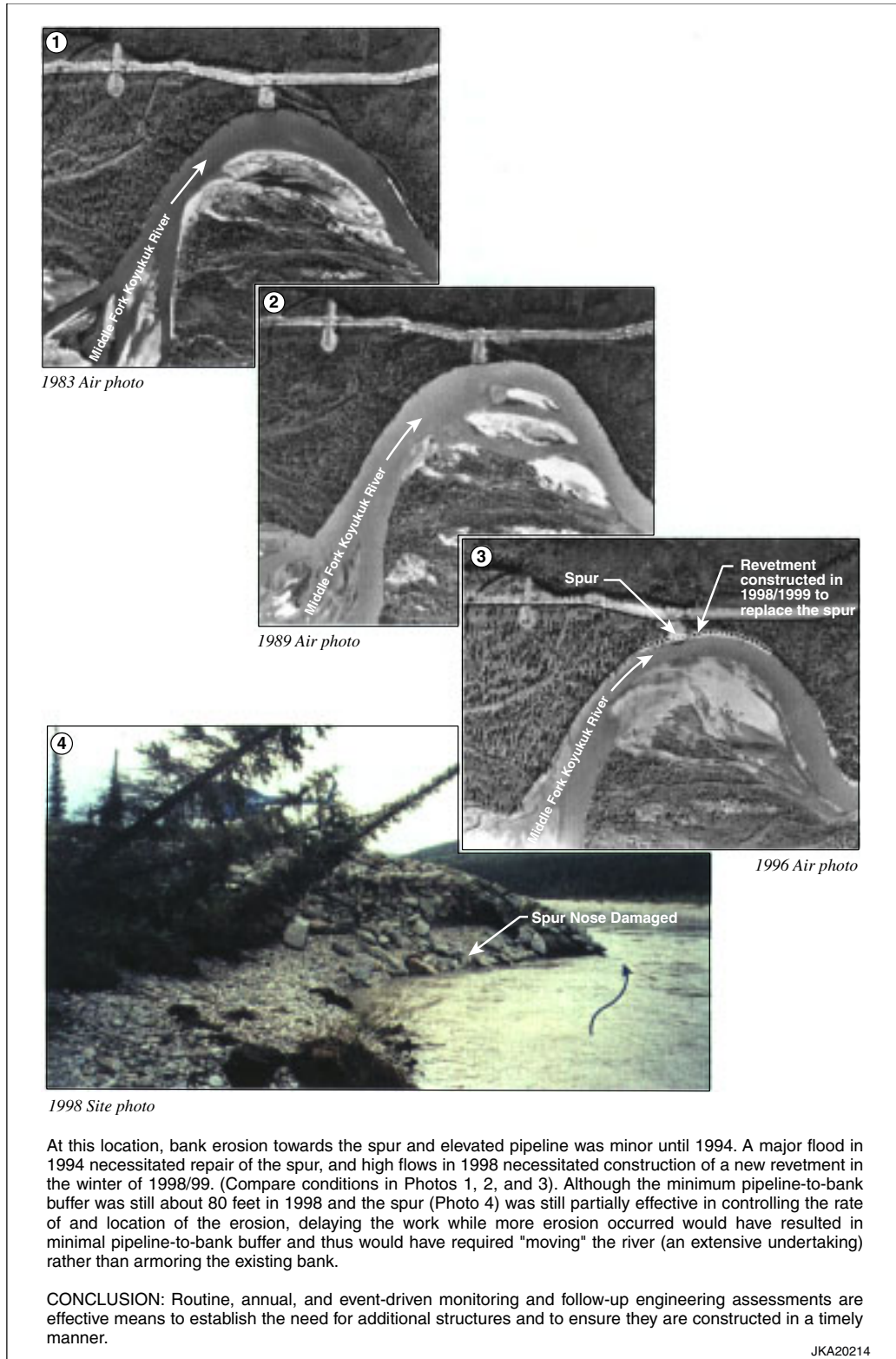
FIGURE 4.1-7 Middle Fork Koyukuk River, MP 218, Where Monitoring Led to Follow-up Remedial Action Consisting of Bank Armoring (Source: TAPS Owners 2001a, Figure 4.2-11)
