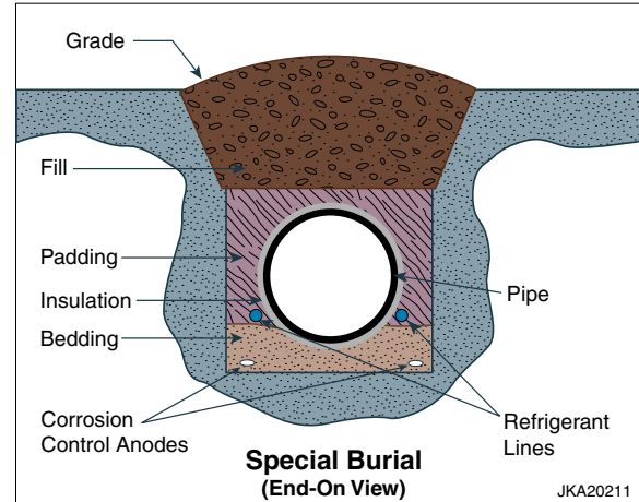
FIGURE 4.1-2 Typical Pipeline Details for Special Burial (Source: TAPS Owners 2001a, Figure 4.2-3)
