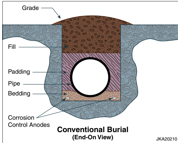
FIGURE 4.1-1 Typical Pipeline Details for Conventional Burial (Source: TAPS Owners 2001a, Figure 4.2-2)
