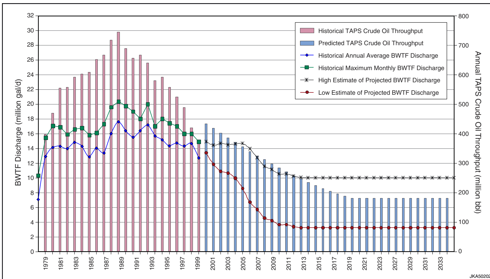
FIGURE 4.3-1 Historical and Projected Flows from the Ballast Water Treatment Facility Discharge and TAPS Throughput (Source: TAPS Owners 2001a, Figure 4.3-15)
