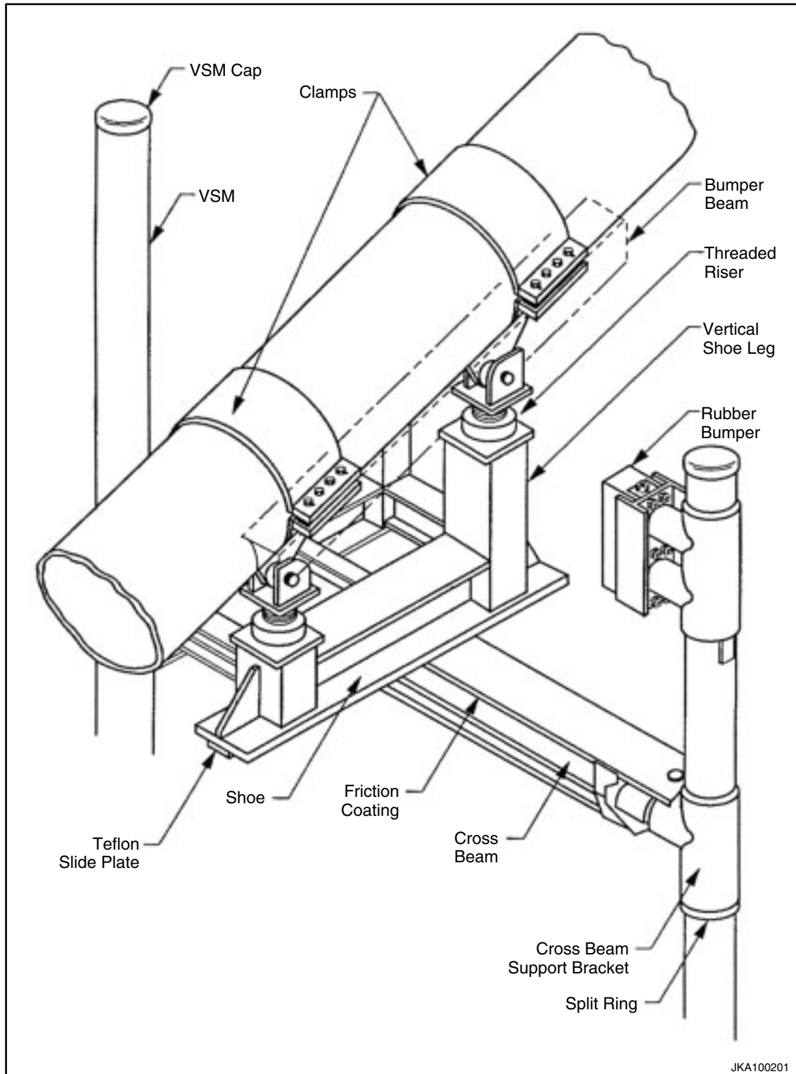
FIGURE 4.1-6 Typical Intermediate Support Assembly (Shown is a support installed on sloped terrain.) (Source: Modified from APSC 2001j)
