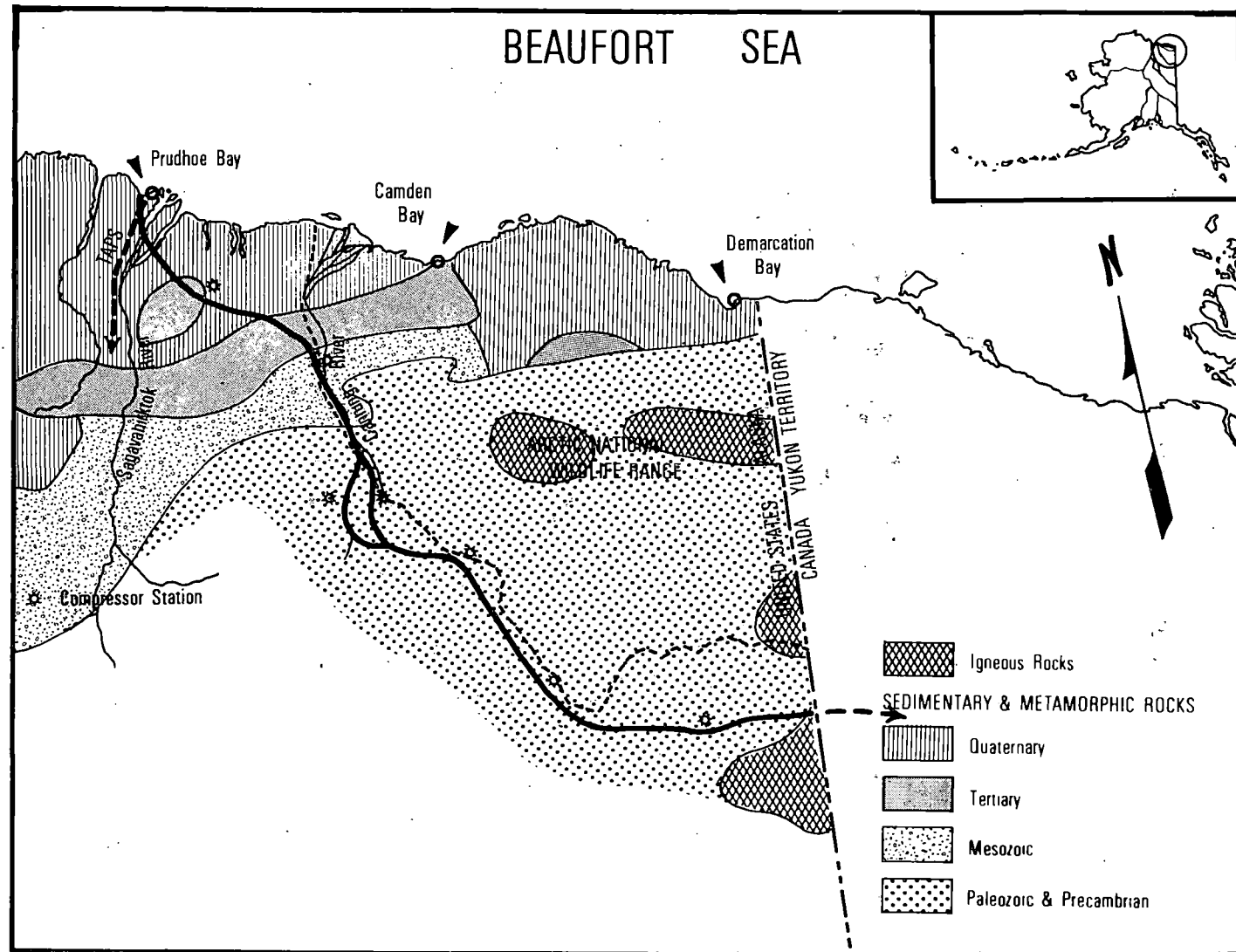
Figure 8.1.1.3-12 Geology of the interior alternative pipeline route
