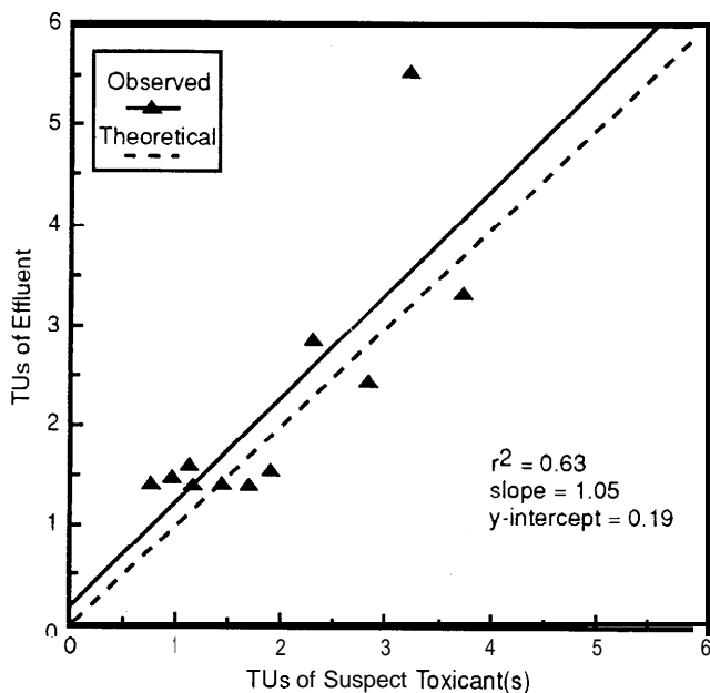
Figure 2-1. Correlation of toxic units (TUs) for an effluent and one suspect toxicant in POTW effluent.
