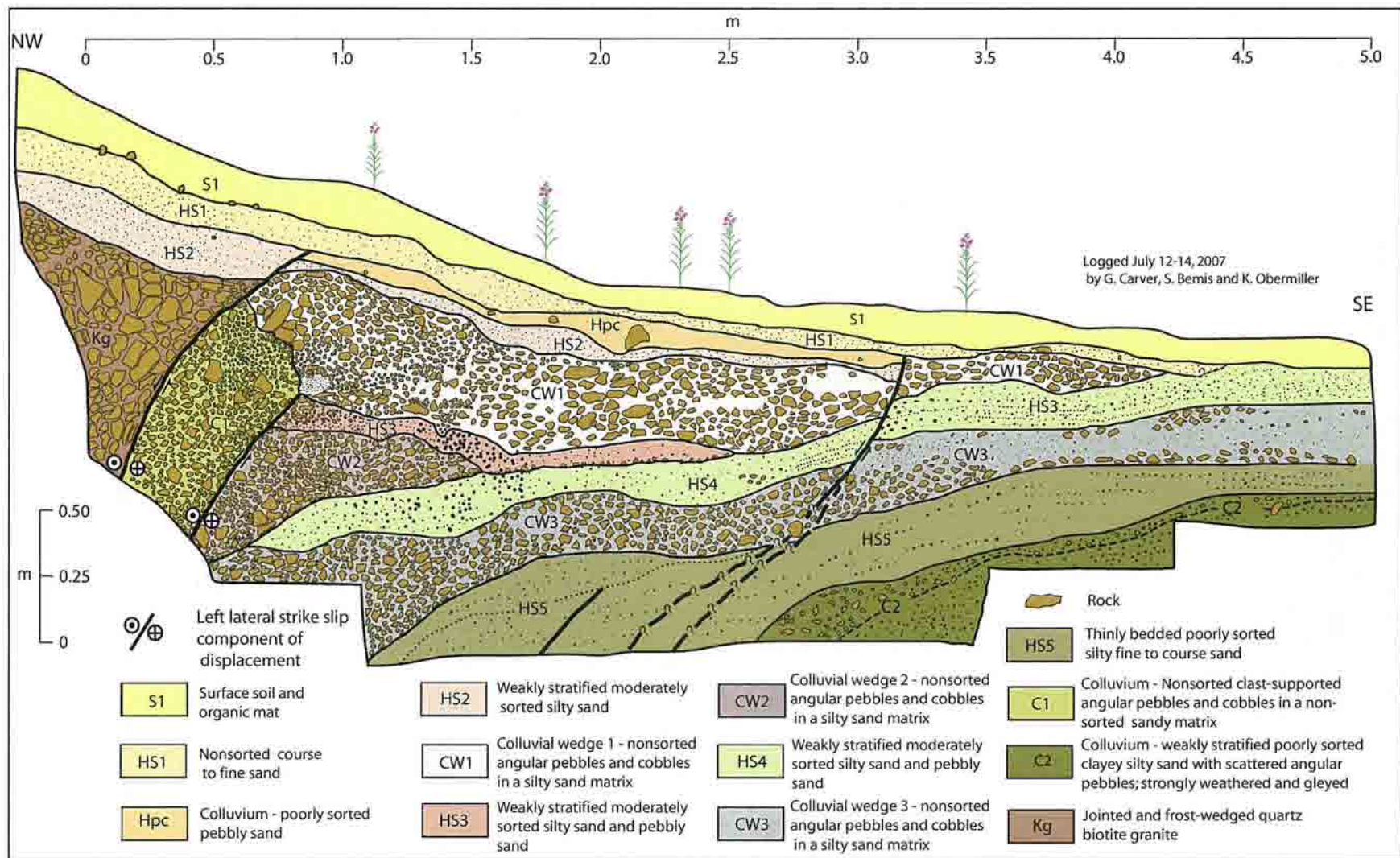
Figure 7. Billy Creek Trench log: A trench across the Billy Creek fault exposed several high-angle faults that offset cobble-rich colluvium and interbedded fine-grained eolian and slopewash sediments. The cobble-rich colluvium forms three distinct colluvial wedges that lack soil development and evidence of periglacial reworking, which are common in Pleistocene sediments in the nonglaciated region north of the Alaska Range. The lack of soils and periglacial reworking indicates a latest Pleistocene or Holocene age for the faulting. Units: HS1 = upper sand; Hpc = pebbly colluvium; HS2 = intermediate sand; CW1 = upper colluvial wedge; HS3 = lower sand; CW2 = lower colluvial wedge; HS4 = lowest sand (gley); CW3 = lowest colluvium; Kg = granitic bedrock.
