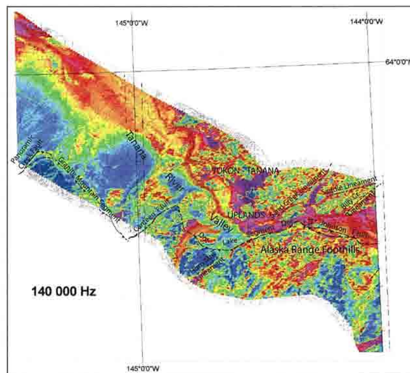
Figure 12. Electromagnetic map (EM), 140,000 Hz, of the corridor with the Dot "T" Johnson, Panoramic, and Canteen faults and the Sand Creek, Horn Mountain, Saddle, and Billy Creek lineaments (Burns and others, 2006). Image shows that sections of the Dot "T" Johnson fault coincide with boundaries between areas with different resistivity signatures, especially along the Dot Lake segment.
