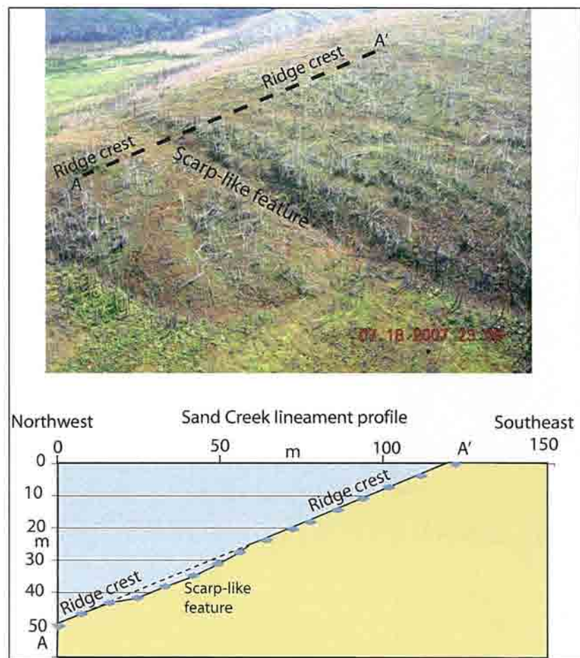
Figure 24. Oblique air photo (upper) and surveyed profile (lower) across a scarp-like feature on the nose of a spur ridge in the upper part of Sand Creek valley along the Sand Creek lineament. The view is from the southwest looking northeast. The profile along the crest of the ridge shows no offset across the scarp-like feature.
