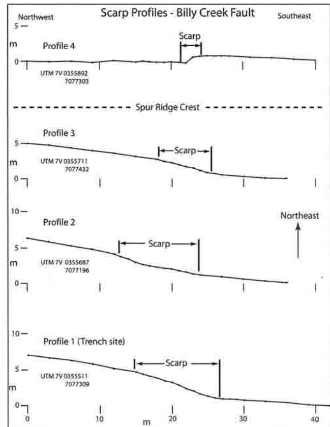
Figure 6. Scarp profiles on the Billy Creek fault at the trench site. Profiles 1, 2, and 3 are on the southwest side of a broad, rounded, northwest-trending spur ridge and have southeast-facing scarps. Profile 4 on the northeast flank of the ridge has a northwest-facing scarp. Scarp aspects reflect left-lateral offset of the ridge.
