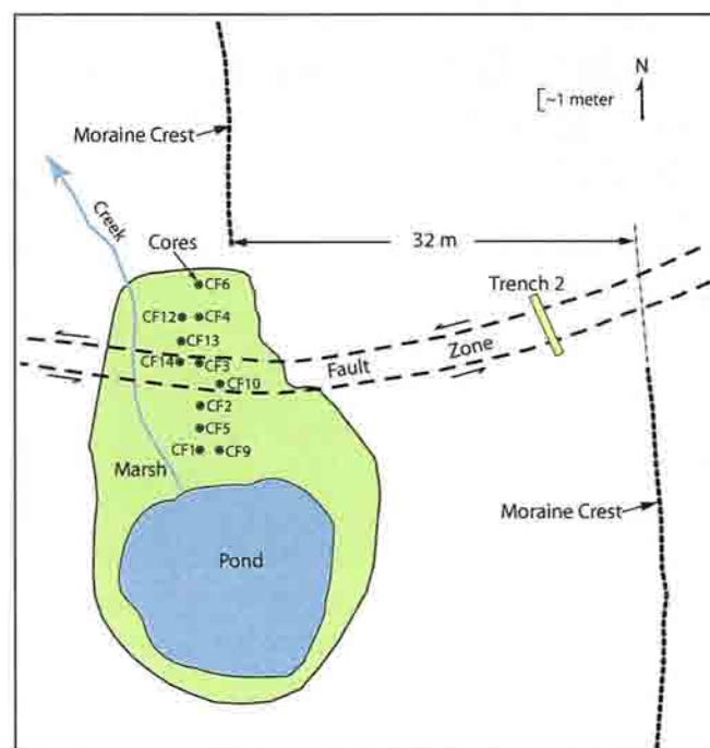
Figure 9. Sketch map showing the location of the trench and the array of cores across the Canteen fault that were obtained from the pond and adjacent marsh impounded by a shutter ridge formed by the offset Donnelly moraine.
