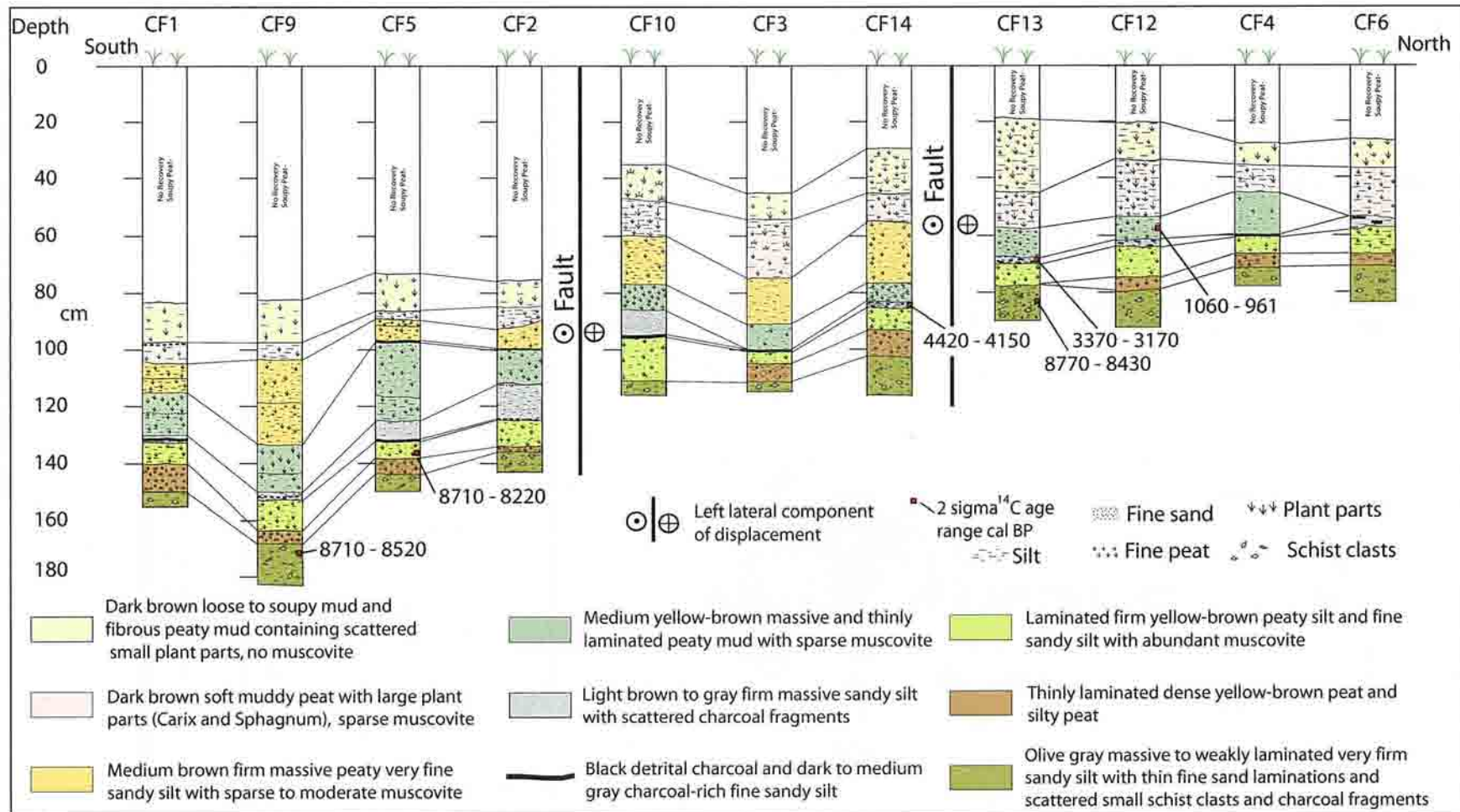
Figure 10. Stratigraphy of the marsh and pond margin across the Canteen fault at the offset Donnelly moraine. ^{14}\text{C} ages for detrital charcoal in distinctive olive-gray compact sandy silt at the bottom of the section are about 8,700 to 8,200 yBP. Ages for sediments associated with a charcoal rich marker bed higher in the section, probably resulting from a forest fire, date between 1,000 and 4,400 cal yBP. Two fault strands underlying the marsh are indicated by stratigraphic offsets. Difference in the elevation of marker beds and units in the stratigraphic sequence indicates multiple middle and late Holocene faulting events.
