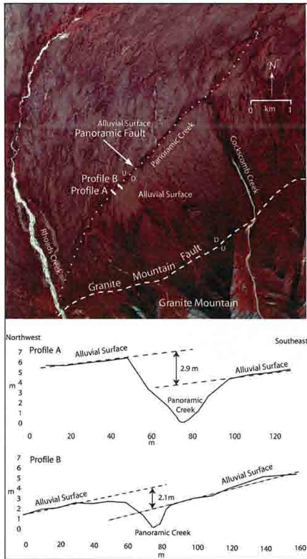
Figure 22 (left). Color infrared vertical air photo showing the trace of the Panoramic fault, which branches off of the Granite Mountain fault on the northwest flank of Granite Mountain and trends northwest across a broad alluvial surface. Two profiles of the surface across the fault show about 2 to 3 m of valley-side up displacement. The linearity of the fault and its northwest trend suggest it has a significant left lateral component.
