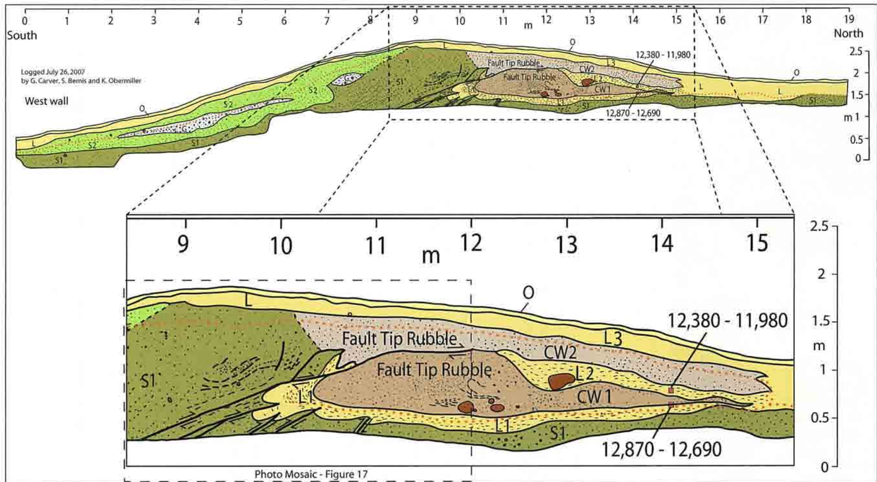
Figure 15. Log of the west wall of trench 1 across the Dot "T" Johnson fault with an enlarged section at the fault. Stratigraphy in the trench consists of stratified sand with gravel lenses overlain by loess. The trench exposed a shallow south-dipping ( \sim 20^\circ ) thrust. Two faulting events are evident in the trench, each represented by fault-tip rubble and an associated colluvial wedge, which interfinger with the loess. In the footwall of the fault, the lower finger of loess (L1) and the overlying fault-tip rubble (CW1) have been dragged along the fault and are overturned. The timing of the two faulting events is constrained by a ^{14}\text{C} age of 12,870–12,690 cal yBP for detrital charcoal at the top of the loess layer (L1) directly under the lower colluvial wedge (CW1) and a ^{14}\text{C} age of 12,380–11,980 cal yBP from charcoal in the middle of the second loess layer (L2) between the two colluvial wedges. The trench was hand-dug across the mole track ridge. Units: O = organic mat; L3 = upper loess; CW2 = upper colluvial wedge; L2 = middle loess; CW1 = lower colluvial wedge; L1 = lower loess; S2 = upper sand; S1 = lower sand.
