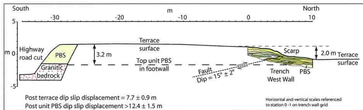
Figure 21. Cross-section showing a measured scarp profile, trench, and adjacent highway road cut at the Sears Creek trench site.
