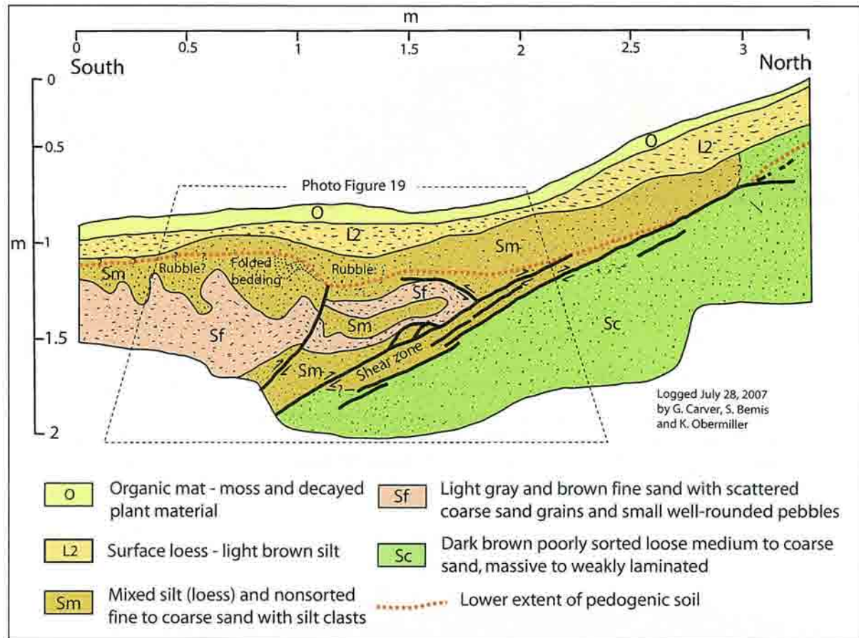
Figure 18. Log of the west wall of trench II on the Dot "T" Johnson fault. Like trench I, trench II exposed a south-dipping, low-angle thrust fault indicative of a near-surface thrust wedge. The stratigraphy in the trench consists of stratified coarse sand in the footwall, and fine to coarse poorly sorted sand and silt in the hanging wall. The sands are capped by loess. The sand and silt in the hanging wall is tightly folded and at the fault tip is overturned. No datable material was found in the trench. Strike of shear zone is N90°E and dip is between 24° and 33°S.
