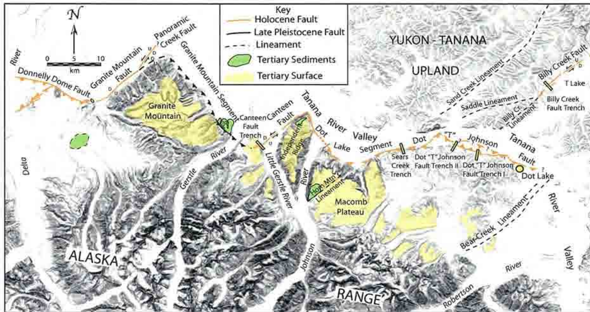
Figure 4. Middle and late Tertiary sediments of the Usibelli Group and Nenana Gravel and exhumed middle Tertiary surfaces in the study area serve as distinctive markers in interpreting post-Tertiary deformation in the study area.
