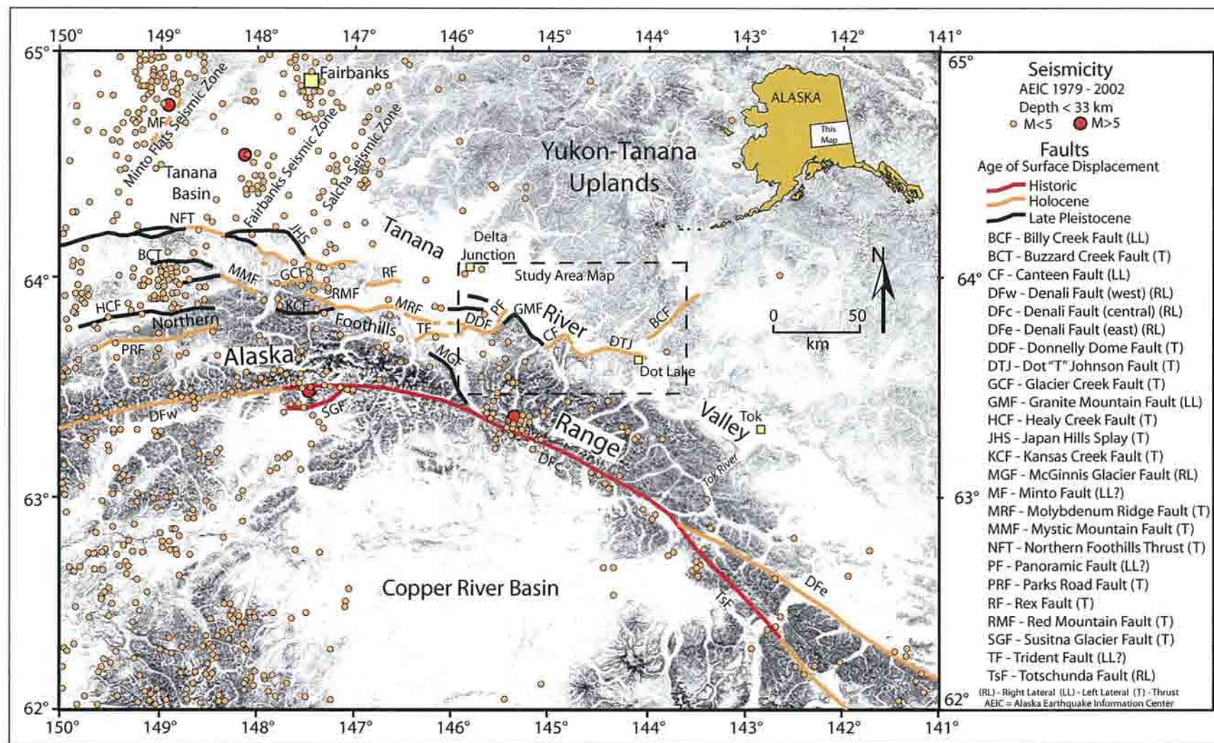
Figure 2. During the period 1979 to 2002, many upper crustal earthquakes were located in the region west of the study area, but in the vicinity of the Alaska Highway Corridor shallow seismicity was sparse with most earthquakes located in the foothills on the north flank of the Alaska Range. Principal faults in the region include the Denali fault, which is a major right-lateral fault that extends along the axis of the Alaska Range, and the thrust faults of the Northern Foothills Fold and Thrust Belt, a system of thrusts and associated fault-related folds in the foothills north of the Alaska Range west of study area. Three of the youthful faults documented in this study in and near the corridor; the Dot "T" Johnson, Canteen, and Panoramic faults, are interpreted to make up an eastern extension of the Northern Foothills Fold and Thrust Belt. Seismicity defines three prominent northeast-trending zones of predominantly left-lateral earthquakes, the Minto Flats, Fairbanks, and Salcha seismic zones. This seismicity is driven by clockwise rotation of fault-bounded crustal blocks that make up the Yukon-Tanana Upland. The Billy Creek fault is interpreted to be an active left-lateral fault kinematically related to these seismic zones.
