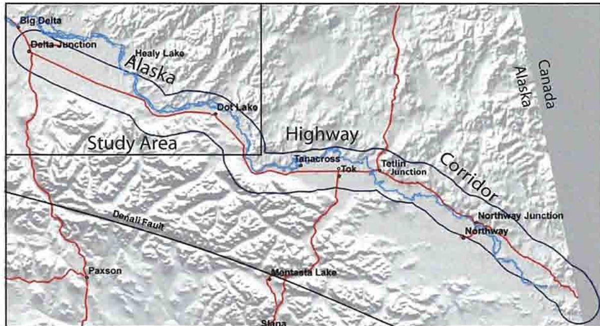
Figure 1. The Alaska Highway corridor is centered on the Alaska Highway between Delta Junction and the Canadian border. The field investigations for this study were conducted along the western part of the Alaska Highway corridor in the Tanana River valley and adjacent areas between Delta Junction and the village of Dot Lake.
