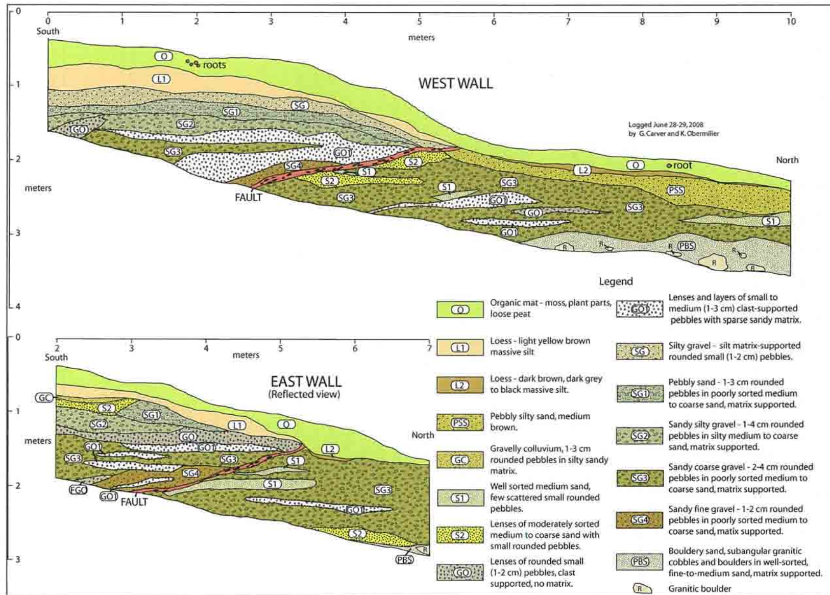
Figure 20. Logs of the Sears Creek trench on the Dot "T" Johnson fault. A low-angle ( 15^{\circ} \pm 2^{\circ} ), south-dipping thrust fault cutting coarse fluvial sediments was exposed in the trench.
