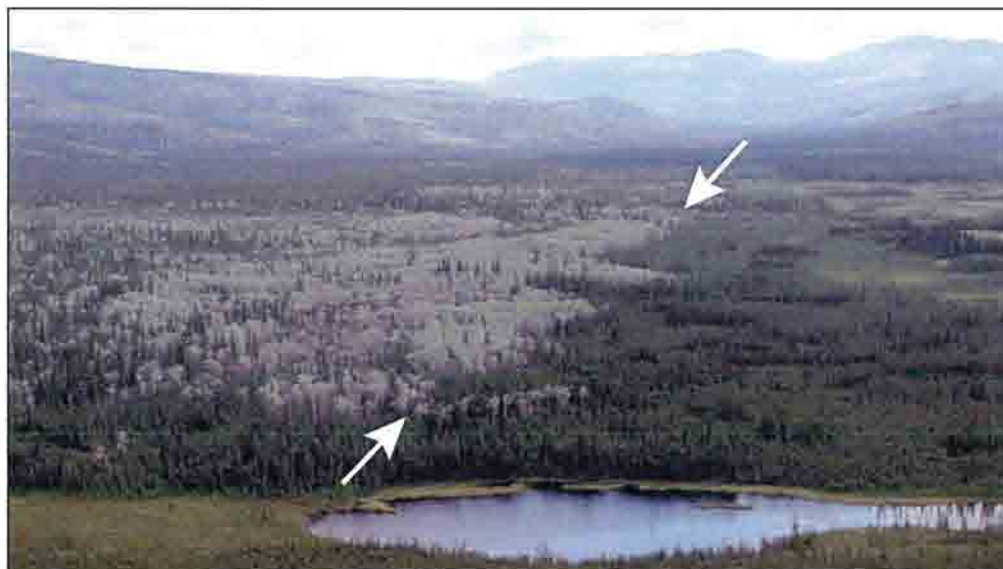
Figure 23 (below). The prominent vegetation line on the Sand Creek lineament in the central part of the Sand Creek valley viewed from the south. Field reconnaissance found no scarp or evidence of Holocene surface faulting associated with the vegetation line.
