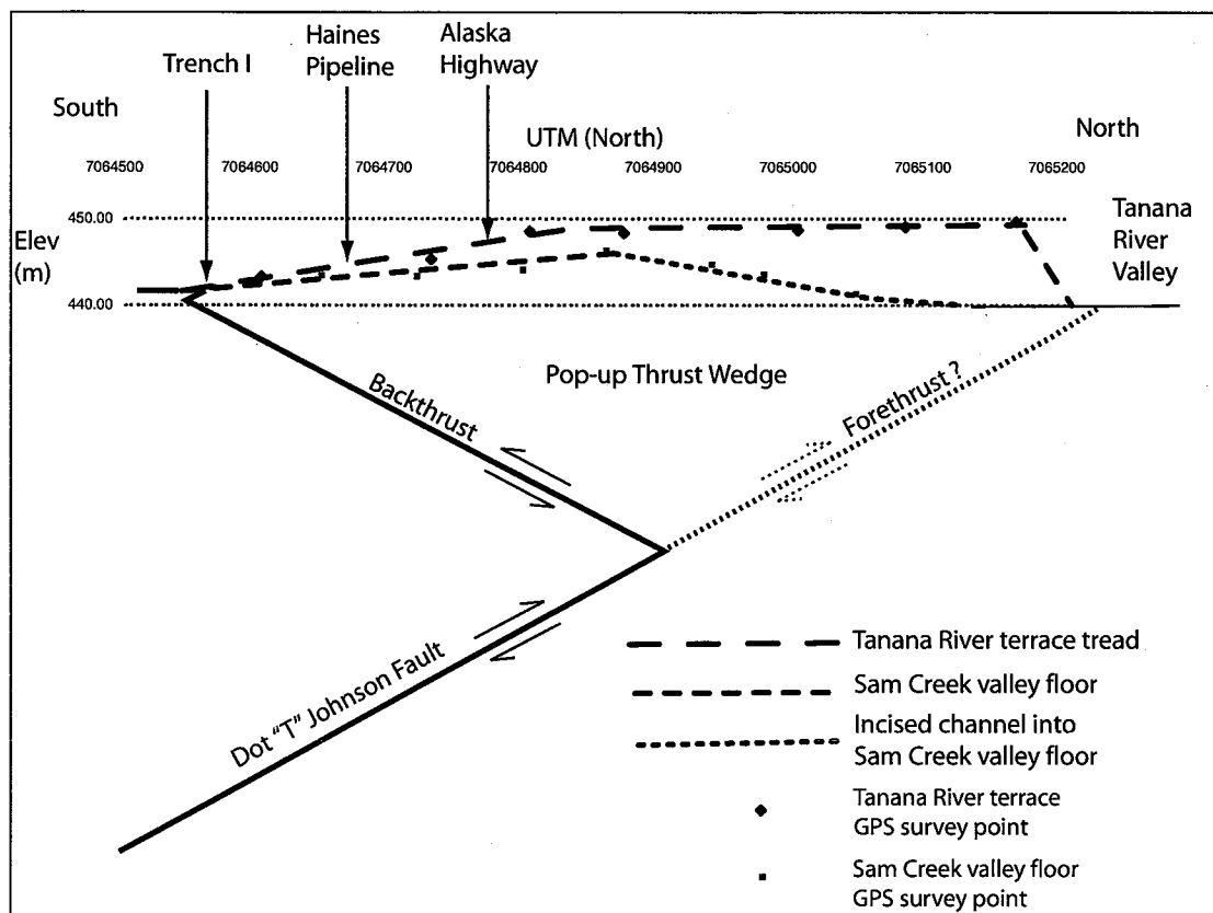
Figure 13. Profiles of the deformed Tanana River terrace and the floor of Sam Creek valley and the structural model for the pop-up thrust wedge on the Dot "T" Johnson fault at trench site I. Profiles were constructed using mapping grade GPS.
