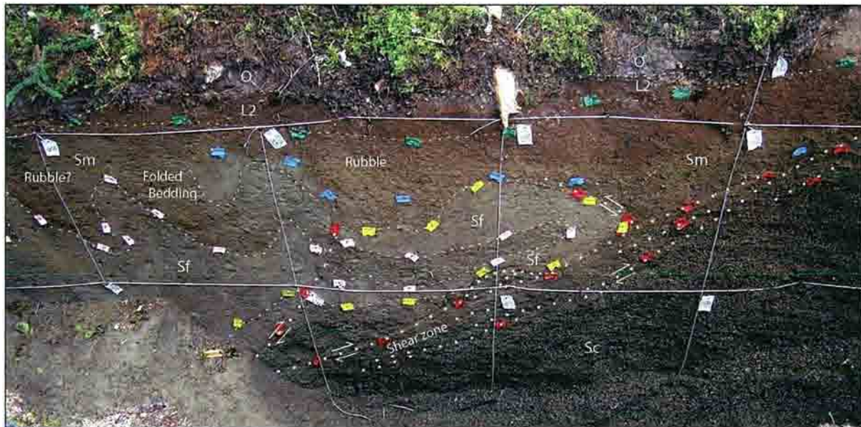
Figure 19. Photograph of the west wall of trench II on the Dot "T" Johnson fault. Grid spacing is 1 m. Unit labels as shown in figure 18. Strike of shear zone is N90°E and dip is between 24° and 33°S.
