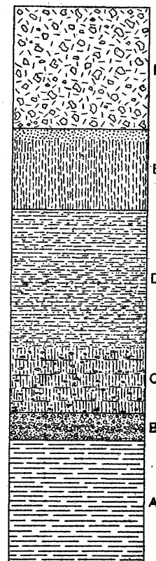
FIGURE 3.—Section on St. Mary River north of Sloan's ranch, Mont. A, Shale; B, northeastern drift, 2 feet, containing many decomposed boulders; C, typical loess, 5 feet, containing concretions, hard shells and bones of small animals; D, soil, 10 feet of black clayey loam, consisting of the weathered upper part of the lower loess bed; E, loess, 6 feet, sandy at the top; F, northeastern till, containing crystalline boulders. (From F. H. H. Calhoun.)
