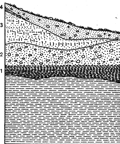
FIGURE 5.—Section on Belly River near Lethbridge, Alberta. 1, Quartzite gravel ("Saskatchewan," interglacial), 10 to 15 feet, overlying Cretaceous shale; 2, pre-Wisconsin till of Keewatin ice sheet (Iowan or Illinoian?), 25 by 30 feet; 3, loess and wind-blown sand, 0 to 50 feet, overlain by laminated silt, 1 to 3 feet (interglacial); 4, Wisconsin till of Keewatin ice sheet, 3 to 13 feet
