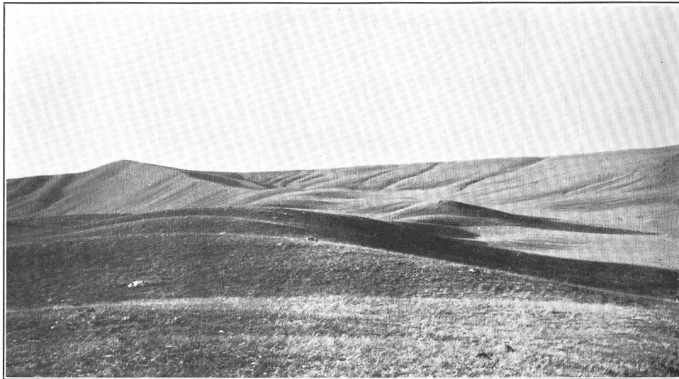
A. TERMINAL MORAINE OF SUN RIVER GLACIER 4 MILES NORTH OF GILMAN, MONT. View north from Park to Park Highway, showing the moraine extending from the Sun River Valley up onto No. 2 bench in the background. The glacier lay at the left (west). Photograph by Eugene Stebinger.
