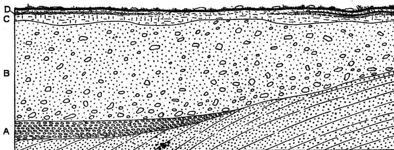
FIGURE 2.—Section on St. Mary River 1 mile south of Kimball, Alberta. A, Quartzite gravel ("Saskatchewan"), interglacial (?), 0 to 15 feet, overlying sandstone; B, glacial till of Keewatin glacier, 50 to 100 feet; C, loesslike clay, 10 feet; D, gravel overlain by a few feet of soil
