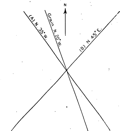
FIG. 8.—Structure at Brown quarry, Dedham.
