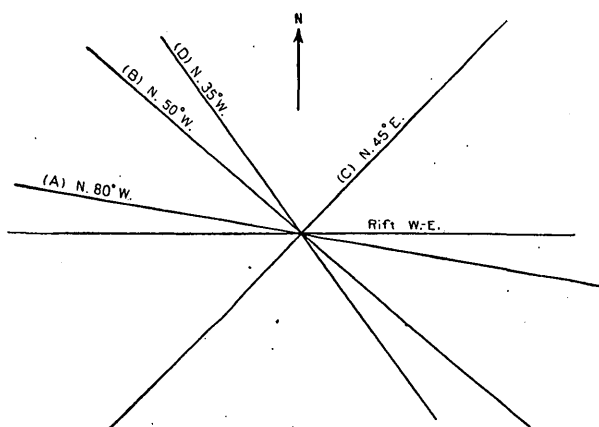
FIG. 22.—Structure at High Isle quarry, Knox County.
