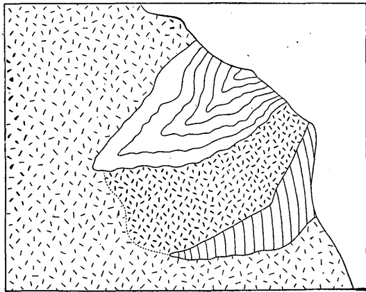
FIG. 29.—Schist inclusions at southwest end of Waldoboro quarry. Total height, 45 feet. The coarse material, between the two inclusions, is pegmatite. The finer is muscovite-biotite granite.
