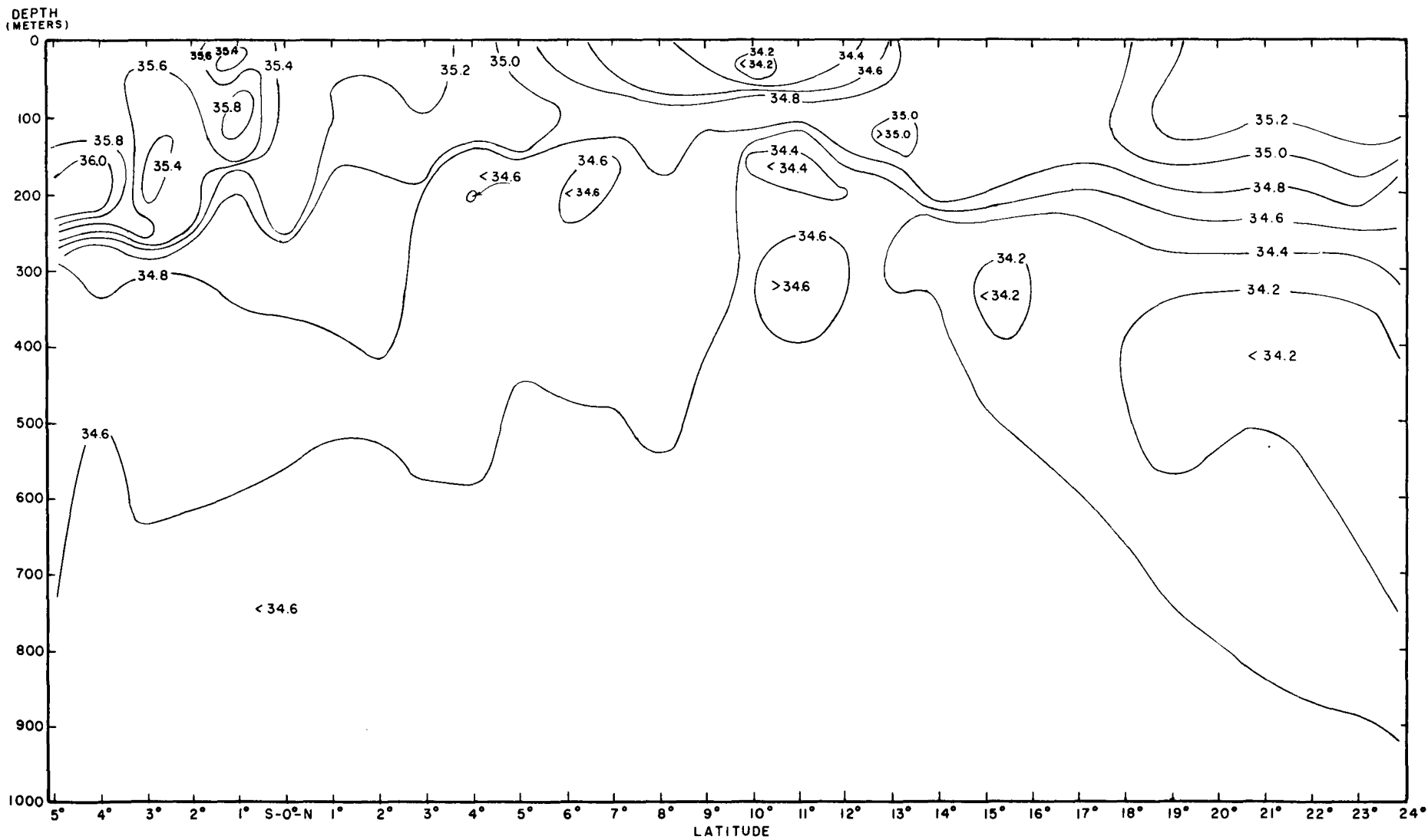
FIG. 12. VERTICAL SALINITY SECTION M/V HUGH M. SMITH CRUISE II STATIONS 1-26 ISOHALINES DRAWN FOR INTERVALS OF .2 ‰
