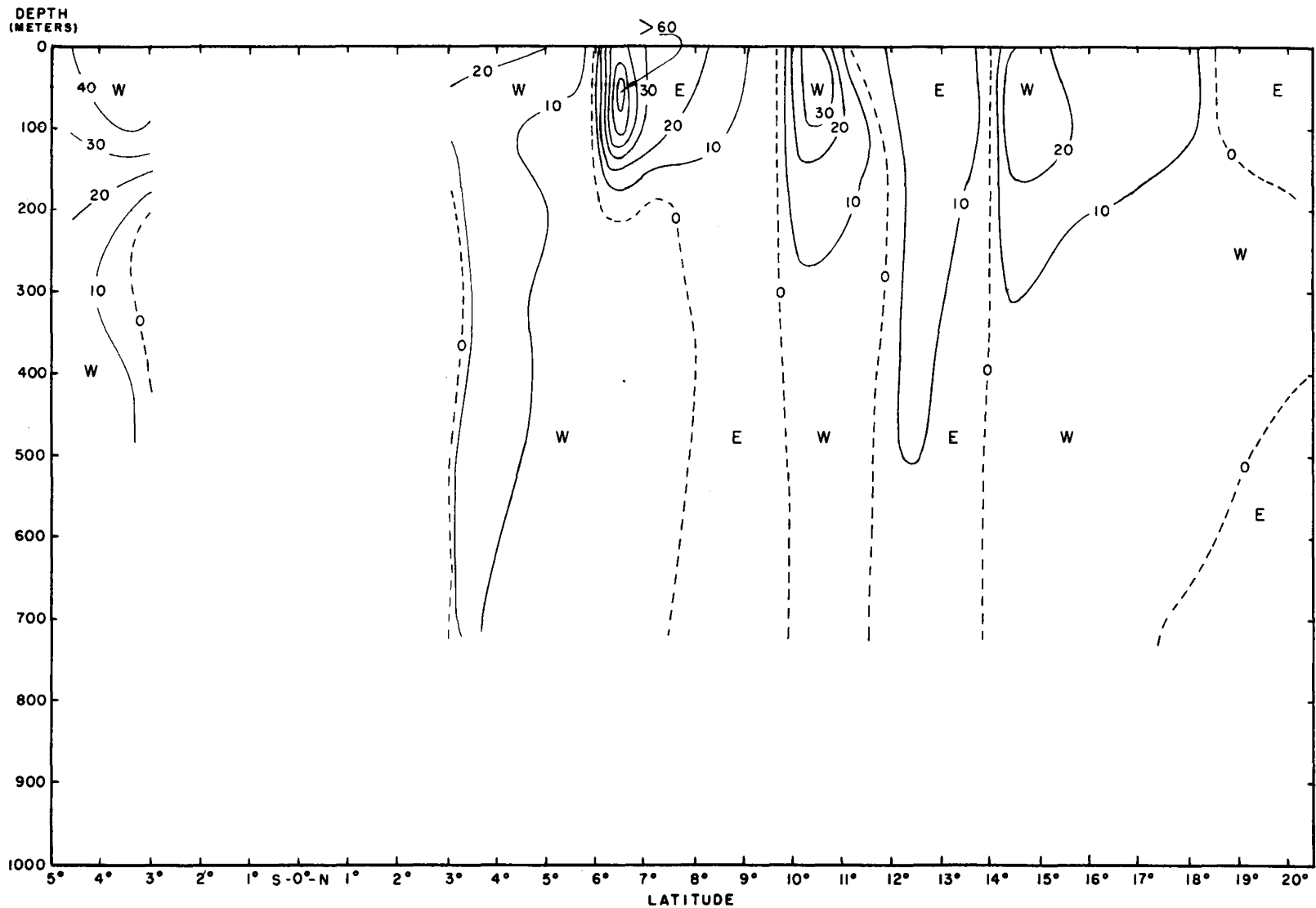
FIG. 7 VERTICAL SECTION OF CURRENTS ASSOCIATED WITH THE DISTRIBUTION OF MASS, M/V HUGH M. SMITH CRUISE II STATIONS 30-53. COMPUTATIONS BASED ON SMOOTHED DYNAMIC CONTOURS. (SEE FIG. 3). CURRENT SPEED INDICATED IN CM/SEC.
