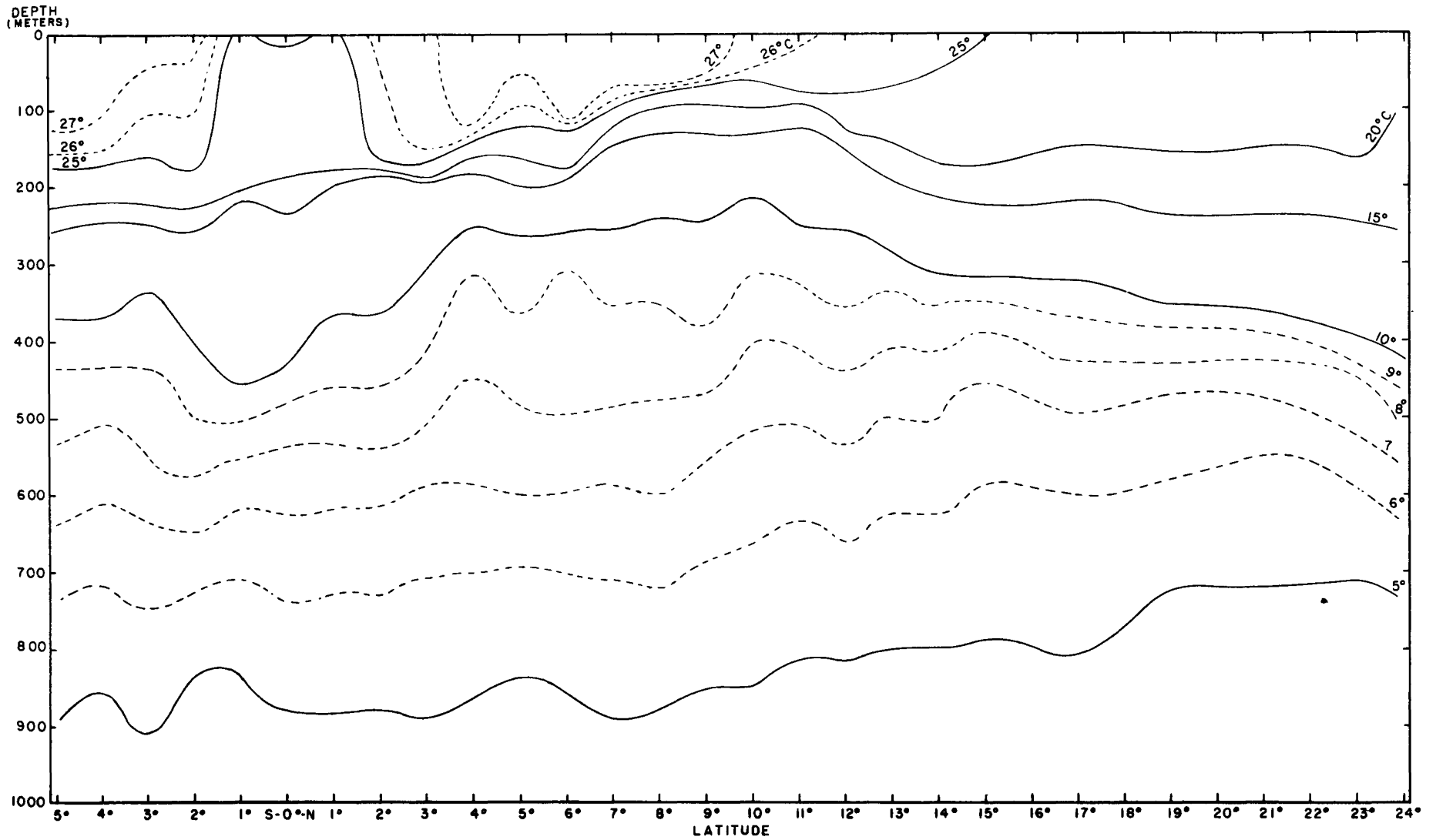
FIG. 8. VERTICAL TEMPERATURE SECTION. M/V HUGH M. SMITH CRUISE II STATIONS 1-26 EVERY DEGREE CENTIGRADE BETWEEN 5°C AND 10°C AND GREATER THAN 25°C ENTERED AS DASH- ED ISOTHERMS.
