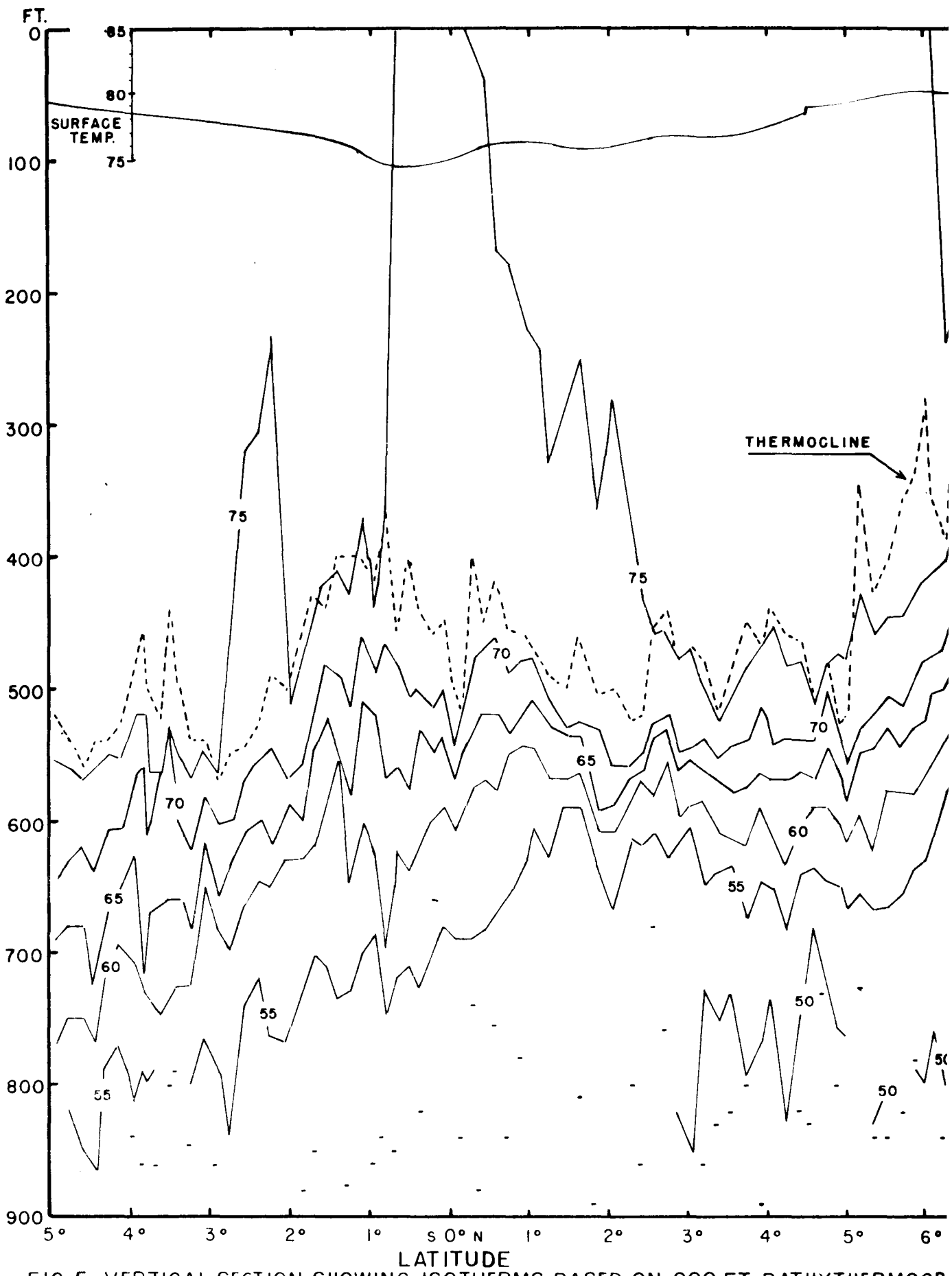
FIG. 5. VERTICAL SECTION SHOWING ISOTHERMS BASED ON 900 FT. BATHY THERMOGR. HORIZONTAL DASHES REPRESENT MAXIMUM DEPTH OF OBSERVATION WHEN LESSING TO INSET TEMPERATURE SCALE. FEBRUARY 18 TO MARCH 1, 1950.
