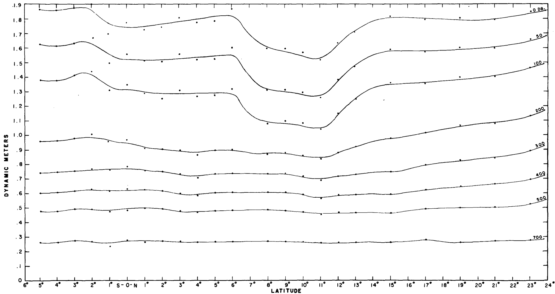
FIG. 2 SMOOTHED PROFILES OF ISOBARIC SURFACES RELATIVE TO THE 1000 DECIBAR SURFACE. CRUISE II M/V HUGH M. SMITH STATIONS № 1-26. POINTS ARE THE RESULT OF THE DYNAMIC COMPUTATIONS.
