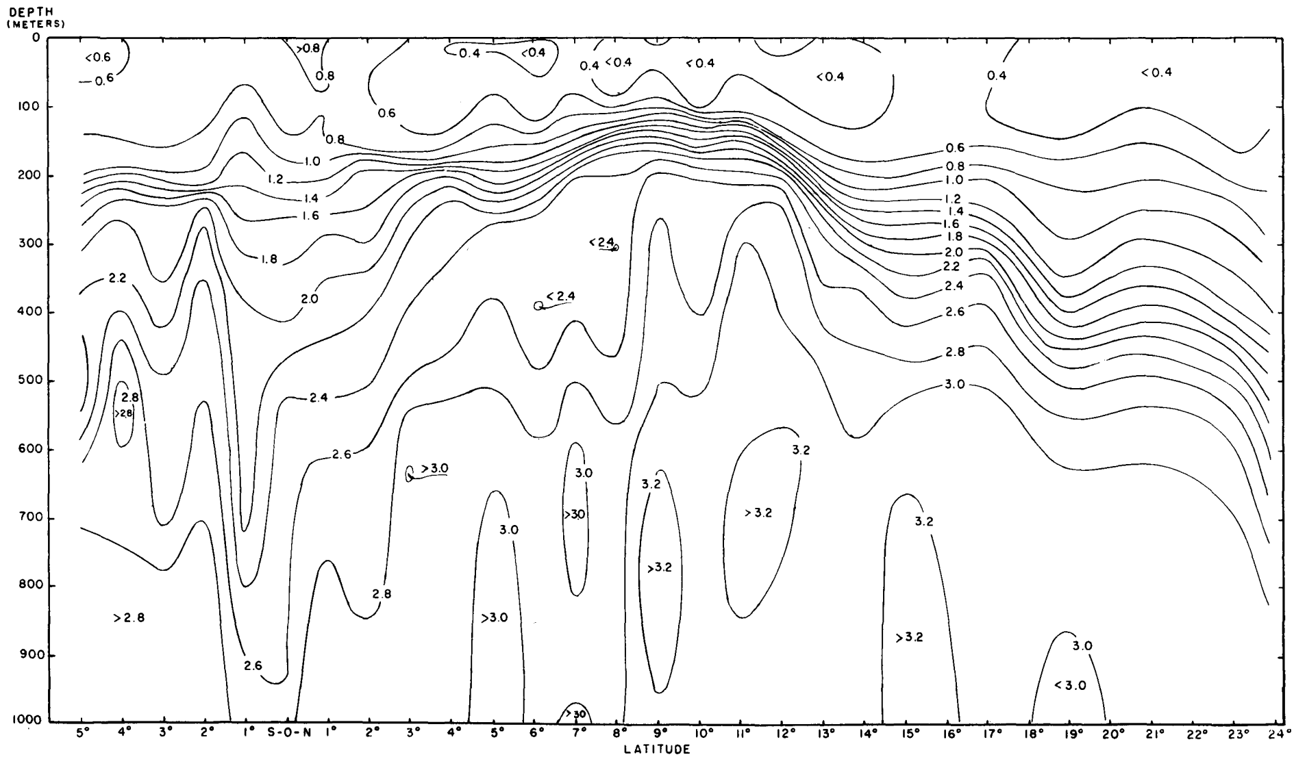
FIG. 10 VERTICAL PHOSPHATE SECTION M/V HUGH M. SMITH CRUISE II STATIONS 1-26 CONCENTRATIONS INDICATED IN \mu\text{g AT/L OF PO}_4\text{-P}
