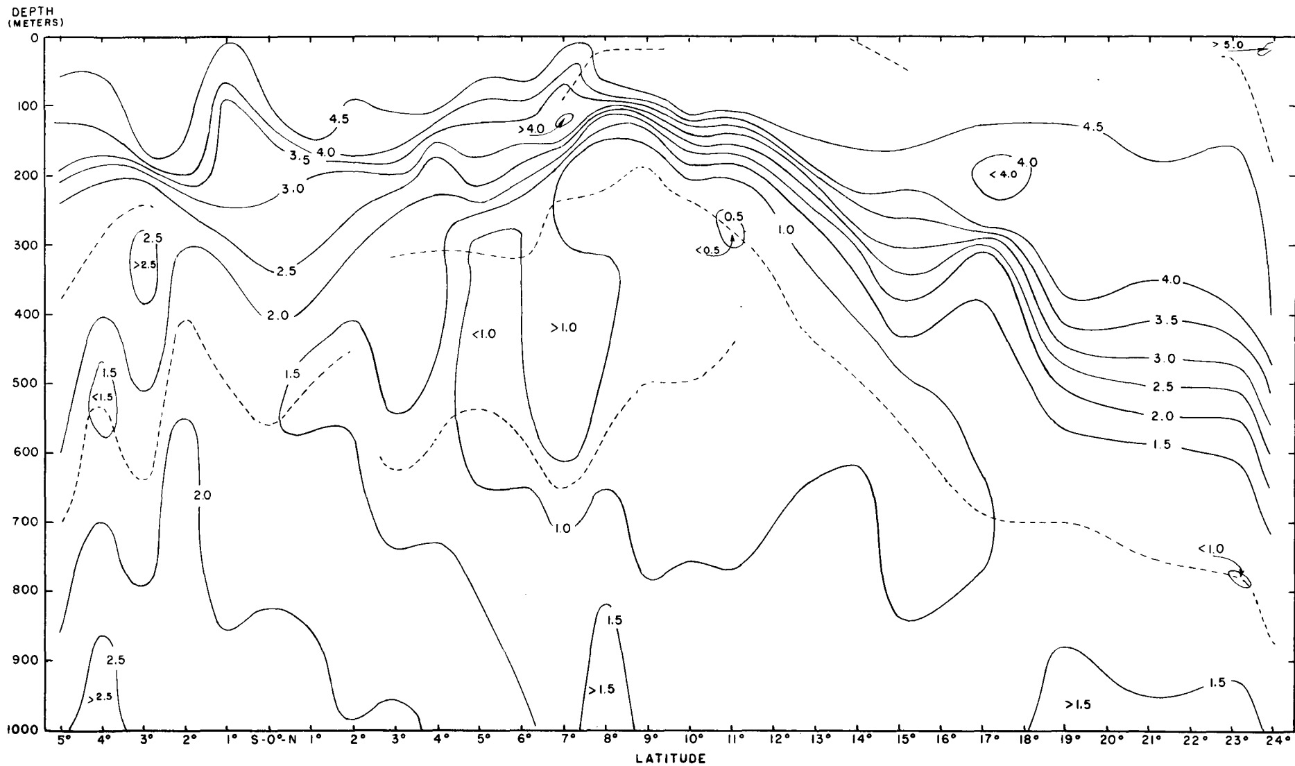
FIG. 14. VERTICAL OXYGEN SECTION M/V HUGH M. SMITH CRUISE II STATIONS 1-26 CONCENTRATIONS INDICATED IN ML/L. DASHED LINES FOLLOW LEVELS OF MINIMUM OXYGEN CONTENT.
