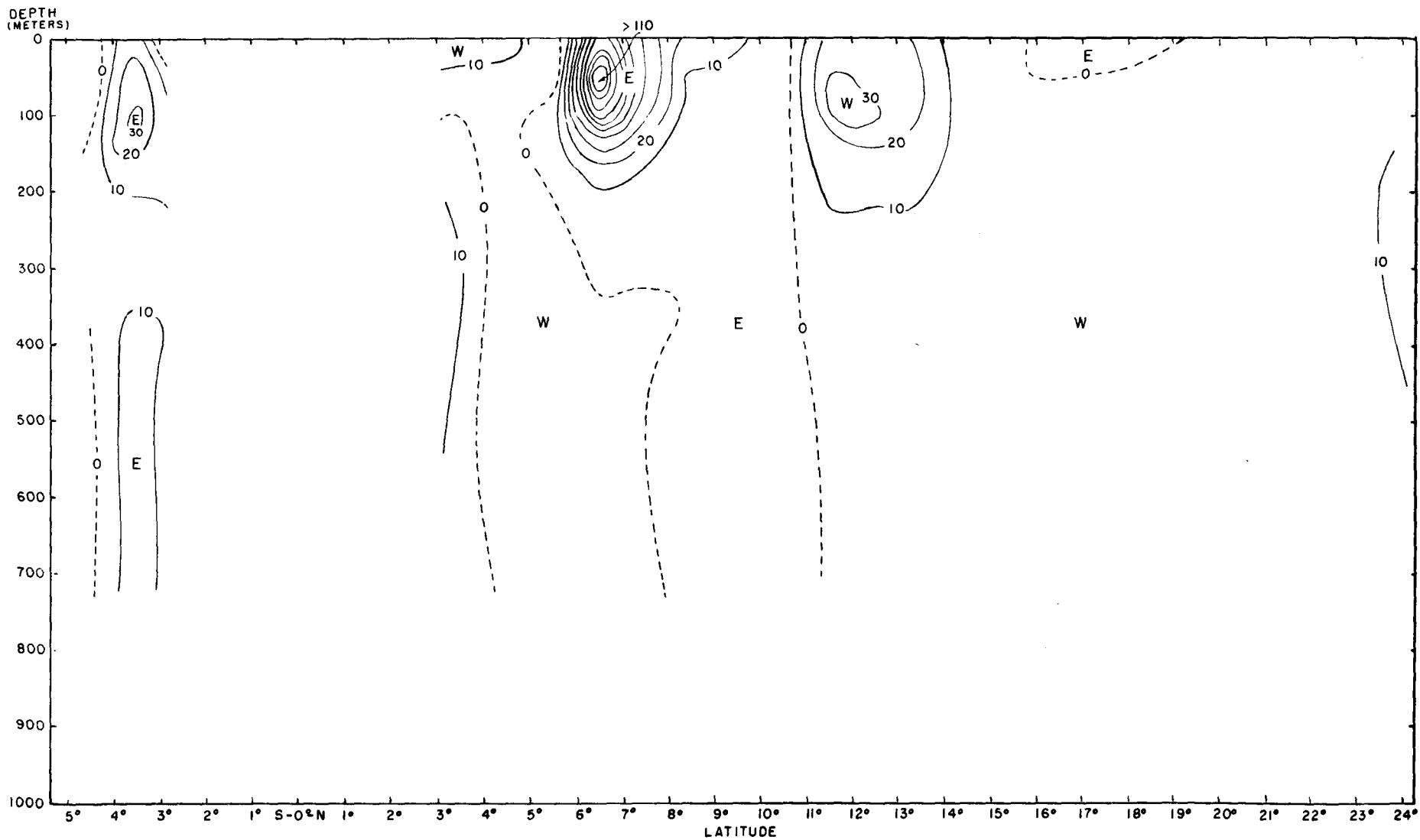
FIG. 6. VERTICAL SECTION OF CURRENTS ASSOCIATED WITH THE DISTRIBUTION OF MASS. M/V HUGH M. SMITH CRUISE II STATIONS 1-26. COMPUTATIONS BASED ON SMOOTHED DYNAMIC CONTOURS (SEE FIG.2). CURRENT SPEED INDICATED IN CM/SEC.
