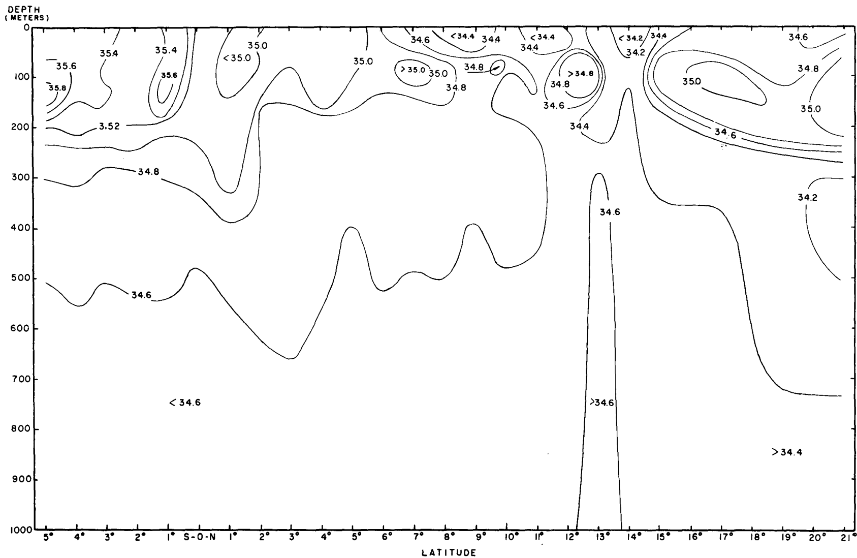
FIG. 13. VERTICAL SALINITY SECTION M/V HUGH M. SMITH. CRUISE II STATIONS 30-53 ISOHALINES DRAWN FOR INTERVALS OF 2‰.
