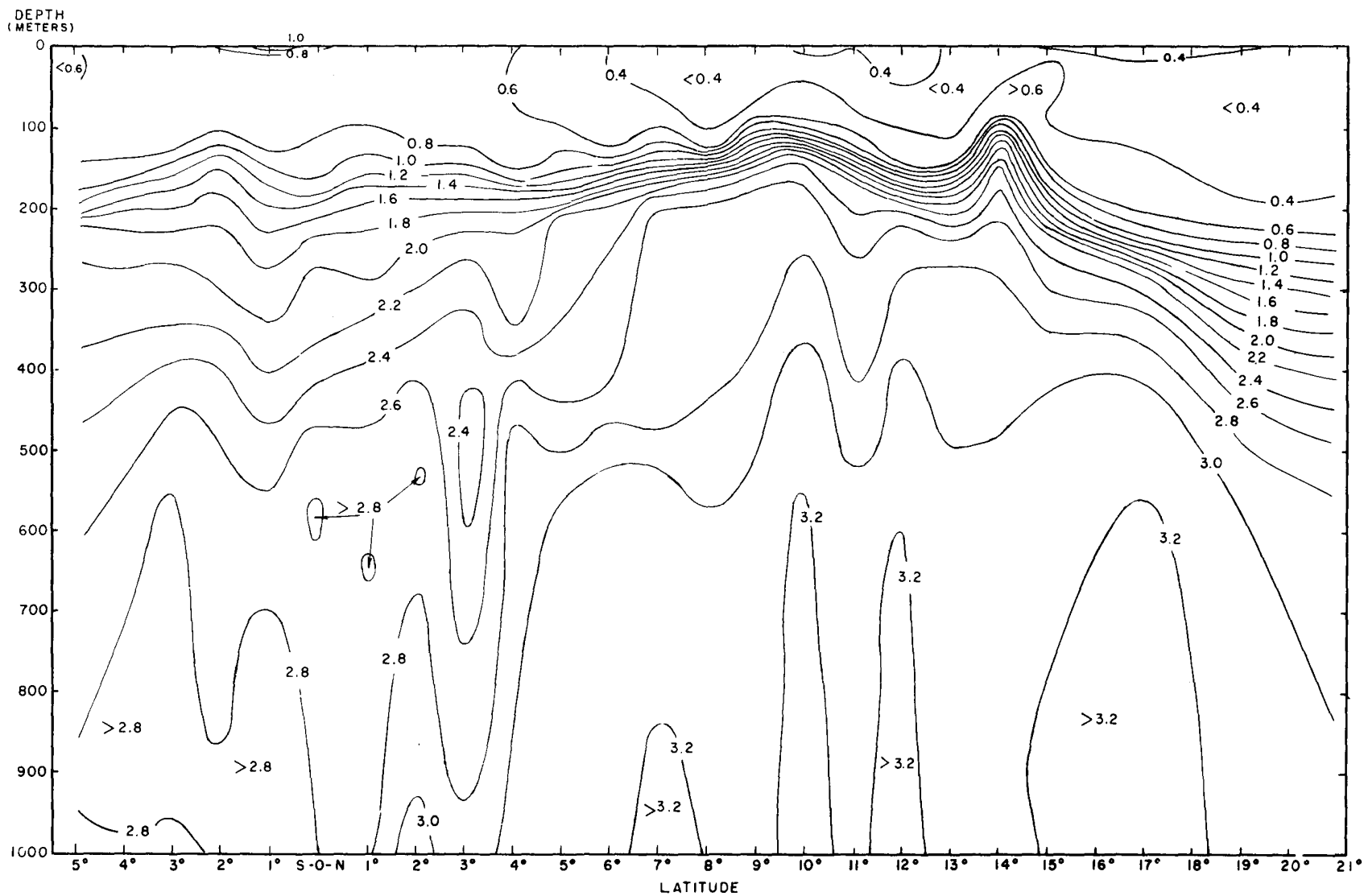
FIG. II. VERTICAL PHOSPHATE SECTIONS M/V HUGH M. SMITH CRUISE II STATIONS 30-53. CONCENTRATIONS INDICATED IN \mu\text{g AT/L OF PO}_4\text{-P}
