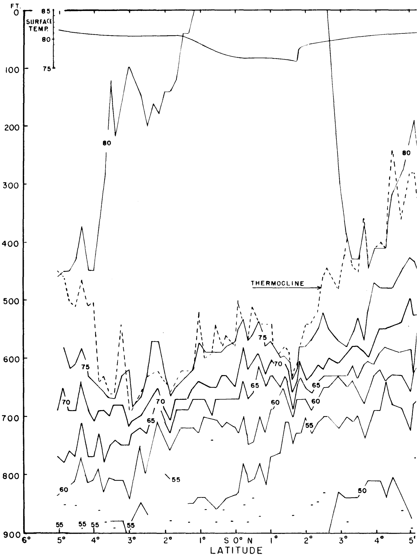
FIG. 4. VERTICAL SECTION SHOWING ISOTHERMS BASED ON 900 FT. BATH. HORIZONTAL DASHES REPRESENT MAXIMUM DEPTH OF OBSERVATION WHEN INSET TEMPERATURE SCALE. JANUARY 26 TO FEBRUARY 8, 1950.
