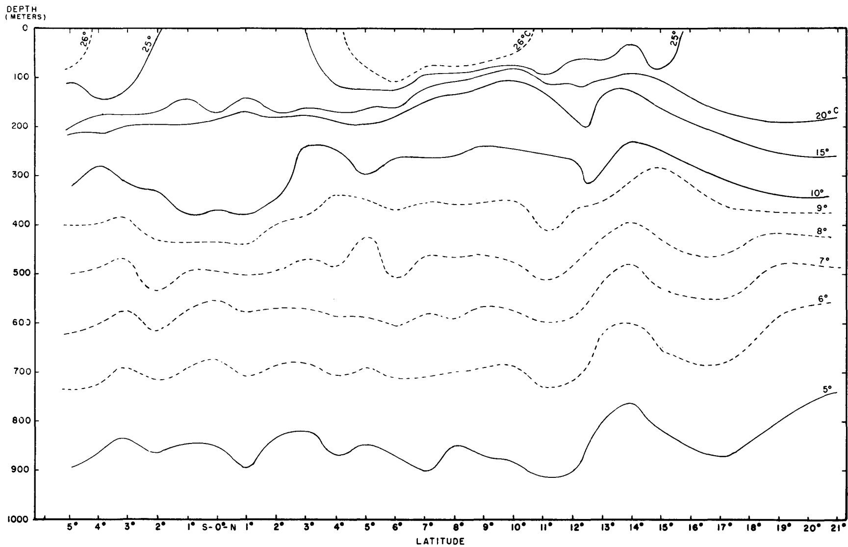
FIG. 9 VERTICAL TEMPERATURE SECTION. M/V HUGH M. SMITH CRUISE II STATIONS 30-53 EVERY DEGREE CENTIGRADE BETWEEN 5°C AND 10°C AND GREATER THAN 25°C ENTERED AS DASHED ISOTHERMS.
