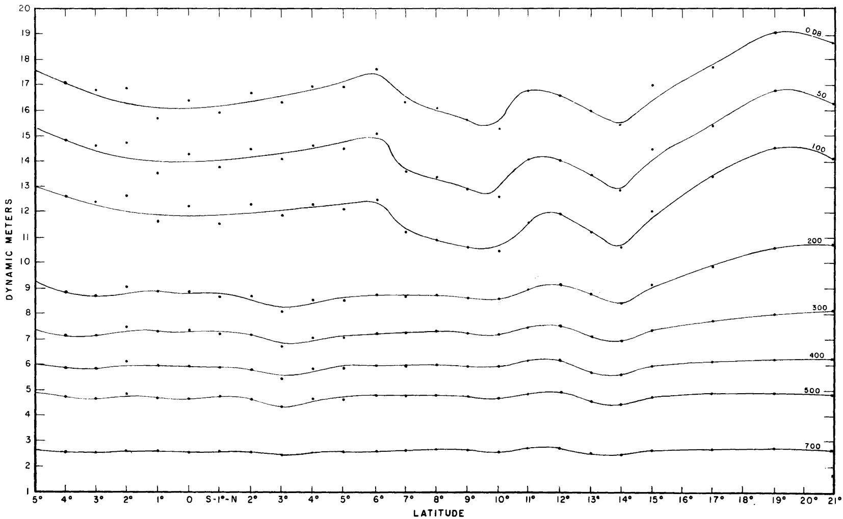
FIG. 3. SMOOTHED PROFILES OF ISOBARIC SURFACES RELATIVE TO THE 1000 DECIBAR SURFACE. CRUISE II M/V HUGH M. SMITH STATION № 30-53. POINTS ARE THE RESULTS OF THE DYNAMIC COMPUTATIONS.
