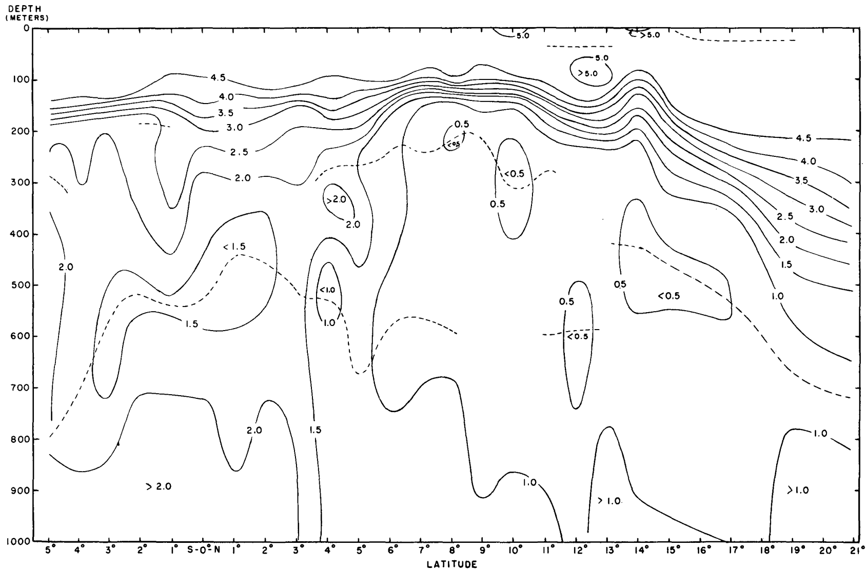
FIG. 15 VERTICAL OXYGEN SECTION M/V HUGH M. SMITH CRUISE II STATIONS 30-53. CONCENTRATIONS INDICATED IN ML/L. DASHED LINES FOLLOW LEVELS OF MINIMUM OXYGEN CONTENT.
