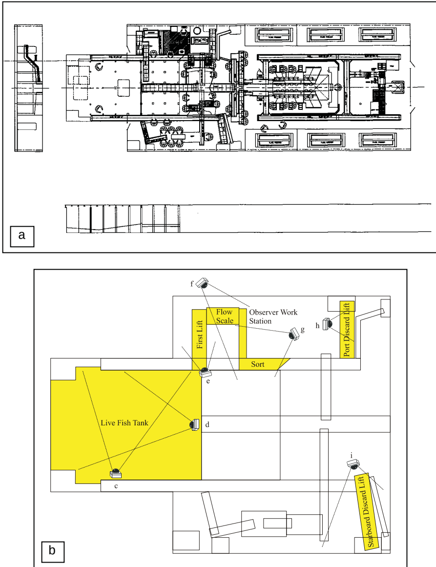
Figure 7. Detailed drawing of F/T Seafisher factory deck (a), and a simplified, closer view of the electronically monitored port conveyor system (b). Factory camera positions and their respective fields of view are included, and the letters c – i correspond to camera images in Figure 8. Gantry cameras (a and b) not shown. (Detailed schematic courtesy of Cascade Fisheries Ltd.)
