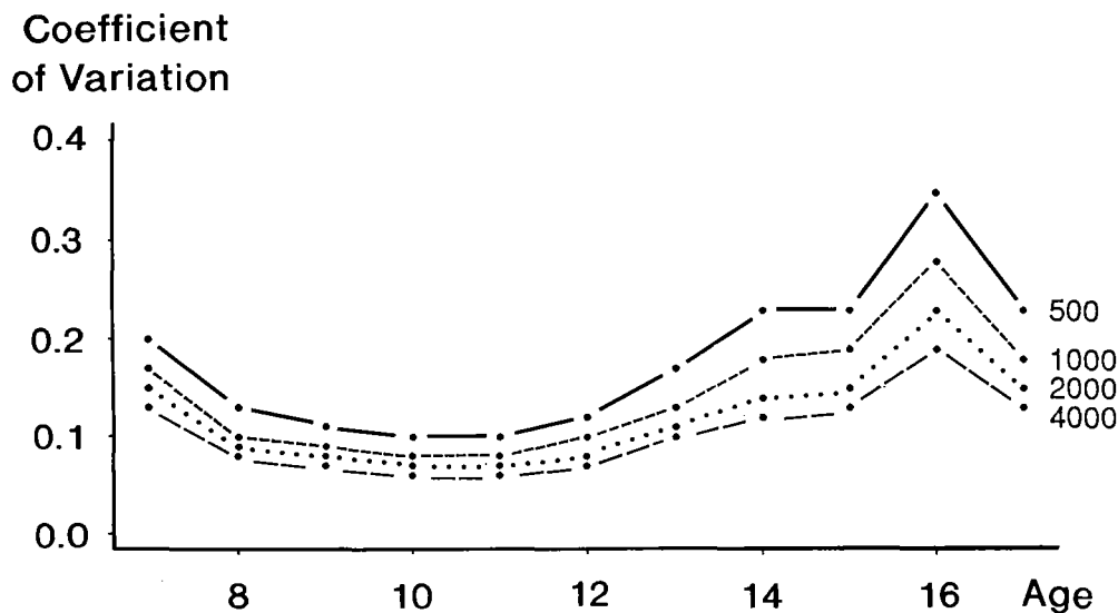
Figure 3. Coefficient of variation of estimated proportion at age, by market sample size, based on data from Area 2B.
