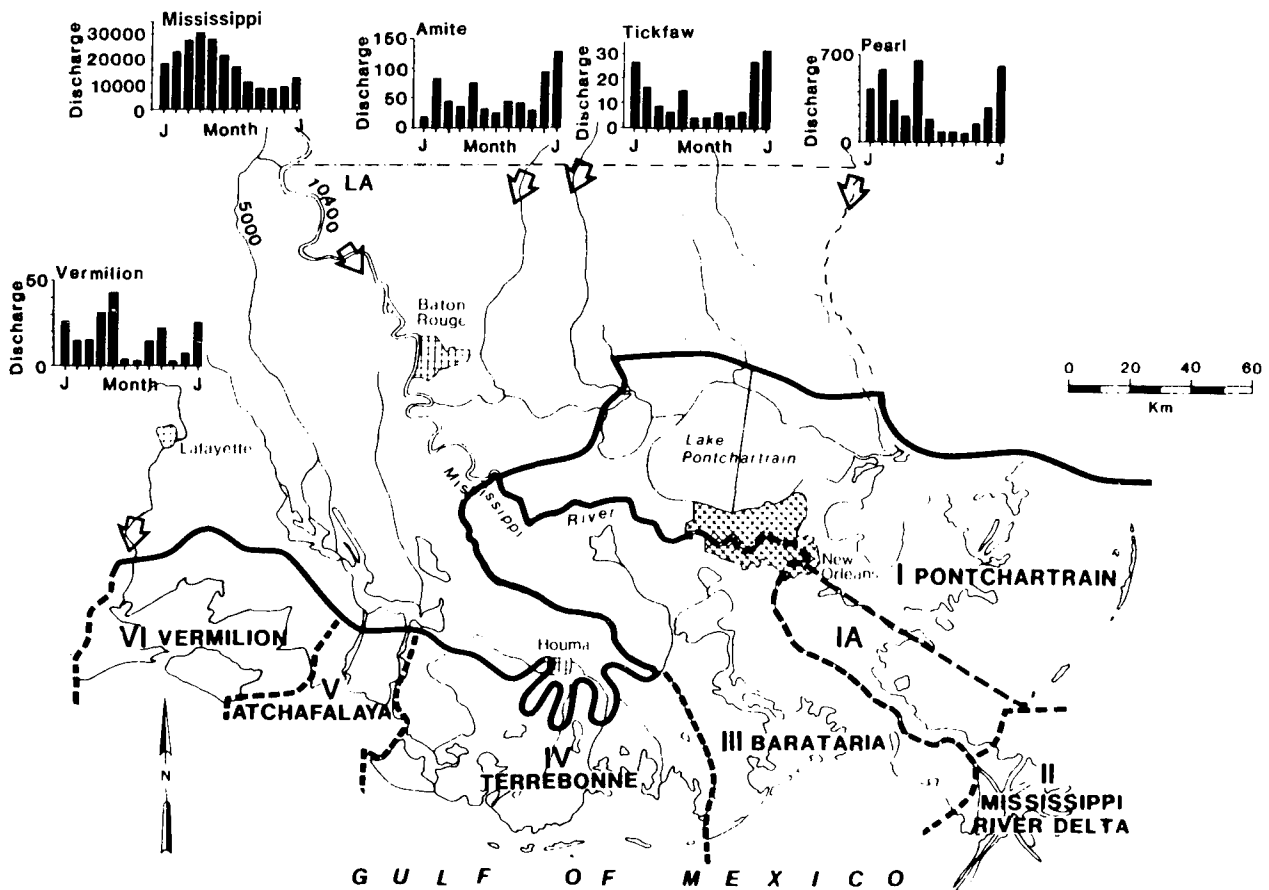
Figure 10. Freshwater inflows to the Mississippi Delta. (Data from USGS 1978). Discharges are in cume. All discharges are for water year 1978 except Mississippi River, which is a long-term mean representing the combined average annual discharge above the confluence of the lower Mississippi (10400 cume) and the Atchafalaya (5000 cume) Rivers.
