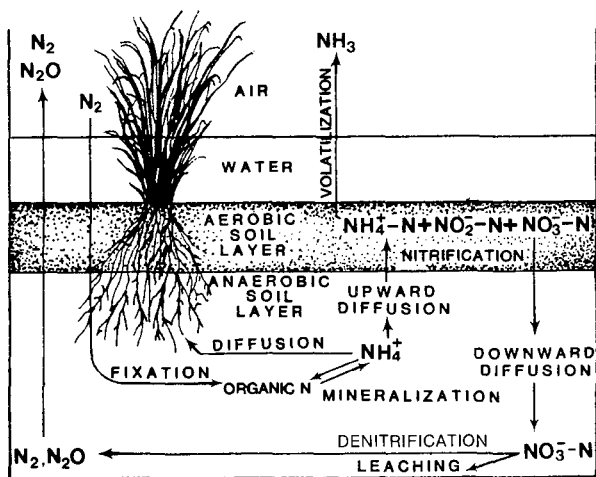
Figure 63. A schematic outline of the redox zones in a submerged soil showing some of the N transformations. The aerobic layer has been drawn thick for clarity. In reality, it is seldom over 1-2 mm in flooded marshes. (Patrick 1982. Copyright. Reprinted from "Nitrogen in Agricultural Soils," with permission of the American Society of Agronomy.)
