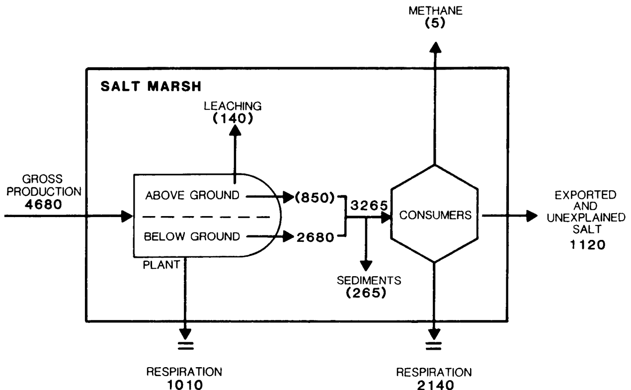
Figure 62. Carbon budget of a Mississippi River deltaic salt marsh (see Table 29 for sources). Rates (g C/m²/yr) are from CO 2 flux measurements, except numbers in parentheses, which are from other sources.
