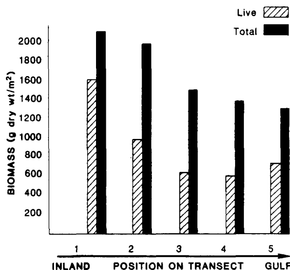
Figure 45. Gulf-inland variations in live and total biomass in Spartina alterniflora marshes (Gosselink et al. 1977).
