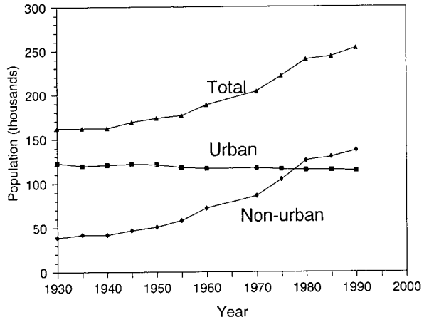
Fig. 1.5. Urban and non-urban population growth in the Buzzards Bay watershed.
