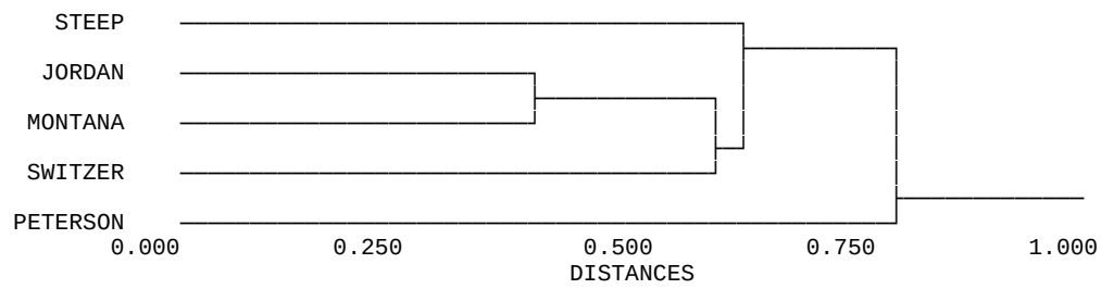
Figure 3. —Cluster diagram of distances (1 – correlations) between time series of coho salmon escapement indices in five systems along the Juneau road system (1981-2004).
