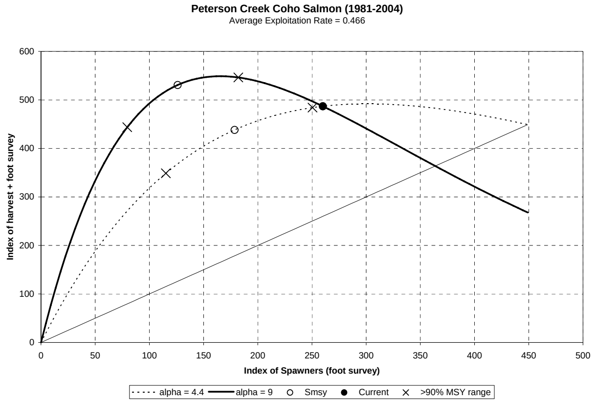
Figure 7. —Theoretical Ricker stock-recruitment relationships based on an average foot survey of 260 and average indexed harvest of 227 coho salmon (1981-2004; • ) in Peterson Creek. The dotted line represents the Ricker curve with an \alpha -parameter of 4.4; the solid line represents the Ricker curve with an \alpha -parameter of 9, and the solid straight line represents replacement. Smsy (o) and escapements that produce 90% of MSY (×) are also shown.
