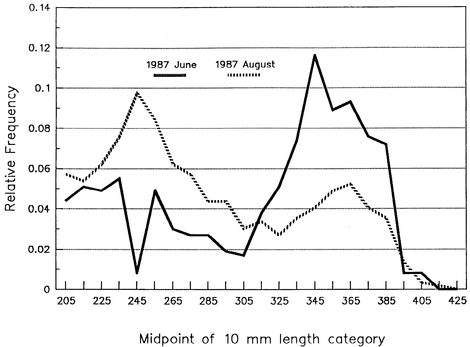
Figure 3. Relative length frequency distributions of Arctic grayling captured in June of 1987 and August of 1987.
