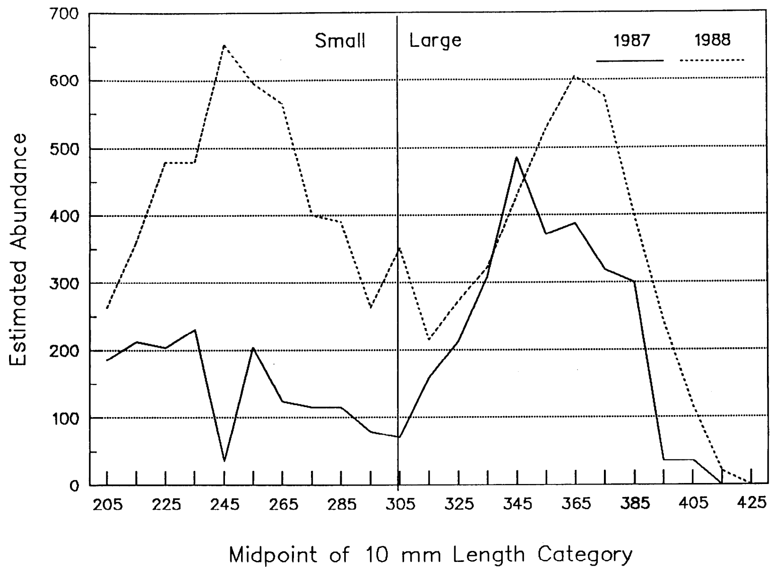
Figure 2. Length frequency distributions of Arctic grayling captured in June of 1987 and 1988.
