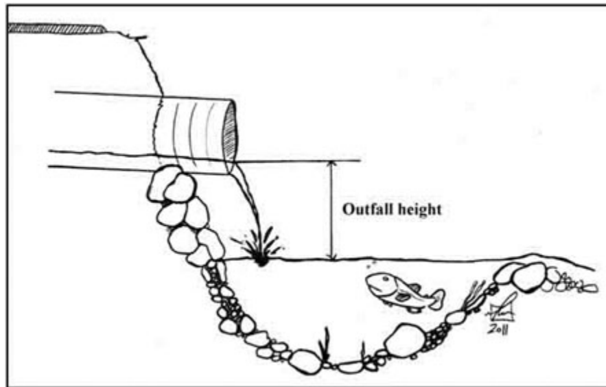
Figure 4.—Illustration showing where outfall height is measured on a freefall into pool outfall type.
