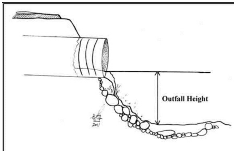
Figure 5.—Illustration showing the outfall height measurement for a free fall onto riprap and cascade over riprap outfall types.
